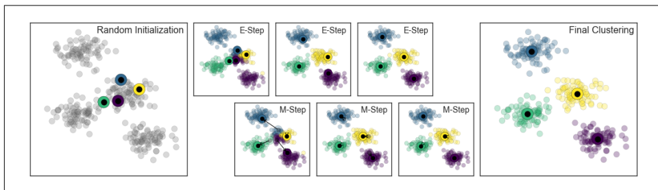
Figure 5-112. Visualization of the E–M algorithm for k-means
