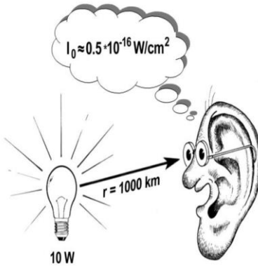
Figure 1: Visualizing the threshold of hearing in terms of the minimum audible intensity I_0 .
