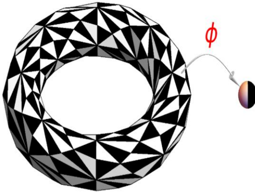
Figure 1: Triangulation of torus, the map \phi maps white triangles to the white hemisphere (of the small sphere) and the black ones to the black hemisphere.
