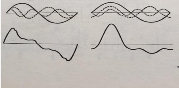
Figure 68. Two sound waves made up of the same fundamental and two harmonics, but in different phase relationship.
