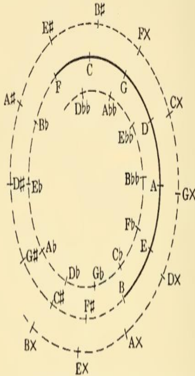
Fig. 55. The form assumed by the clock-face of fig. 54, when true fifths are used. There is now an endless series of notes, such notes as B \sharp , C and D \flat\flat being of different pitch.
