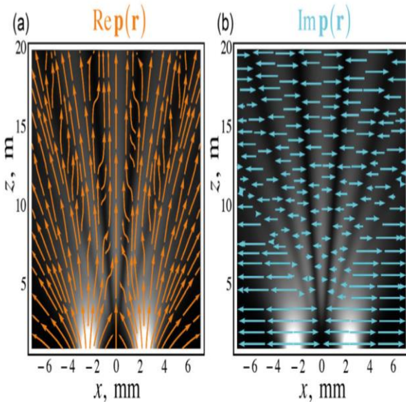
Figure 2. Stream distributions of the real (a) and imaginary (b) parts of the local momentum \mathbf{p}(\mathbf{r}) , equations (9)–(11), for the two-beam interference of figure 1.
