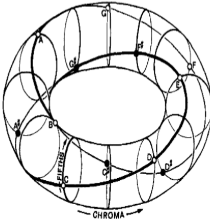
Figure 5. The double helix wound around a torus. (From "Structural Representations of Musical Pitch" by R. N. Shepard. In D. Deutsch (Ed.), Psychology of Music . New York: Academic Press, 1982. Copyright 1982 by Academic Press, Inc. Reprinted by permission.)
