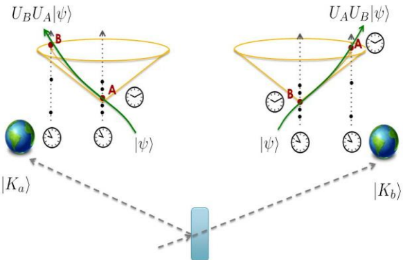
Quantum control of temporal order
