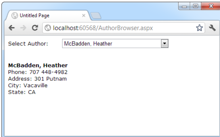
Figure 14-11. Author information
