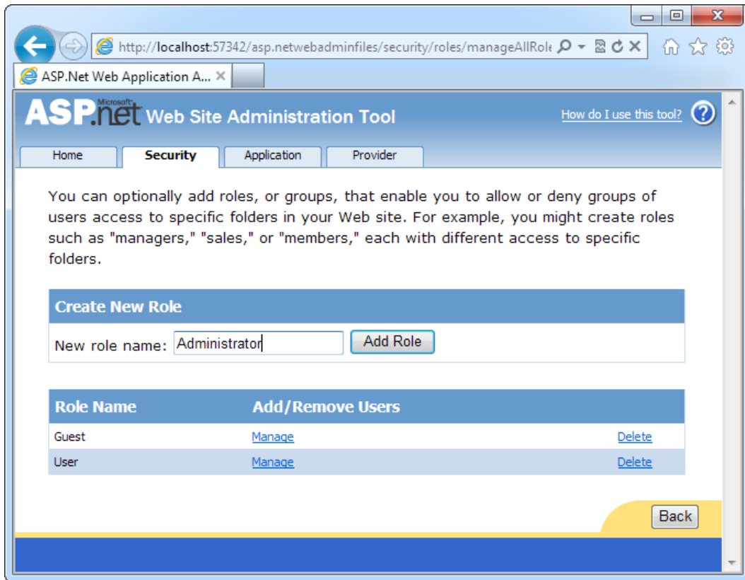
Figure 20-13. Creating roles
