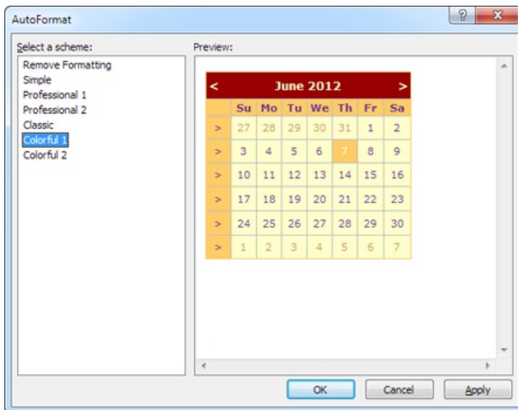
Figure 10-3. Calendar styles
