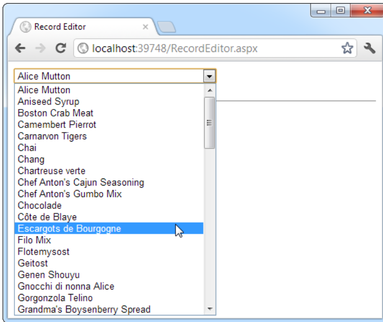
Figure 15-9. Product choices
