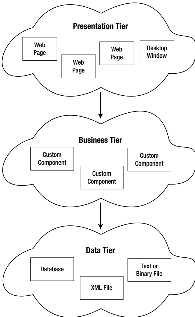
Figure 22-1. Three-tier design
