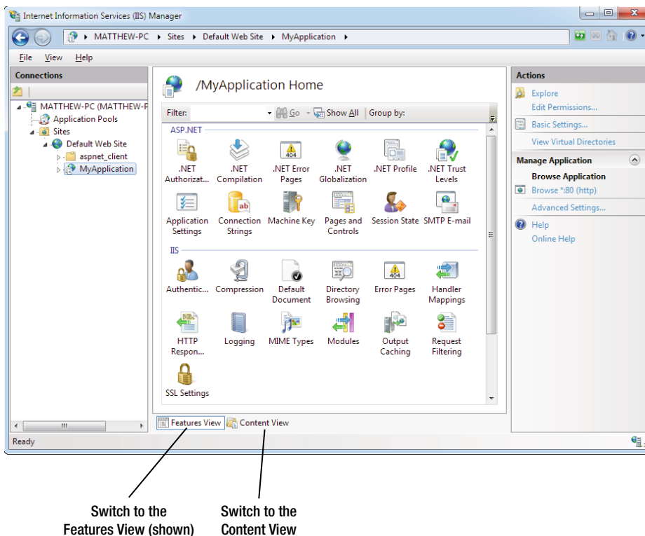
Figure 26-3. IIS Manager
