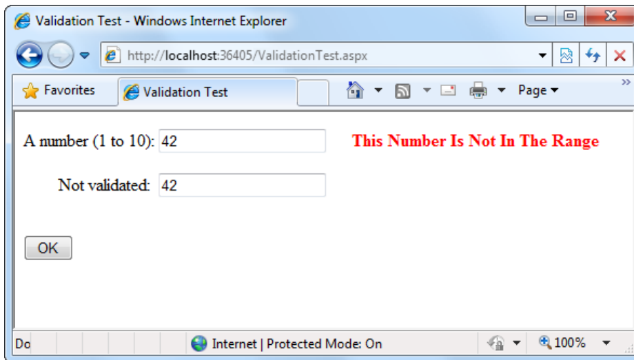
Figure 9-2. Failed validation
