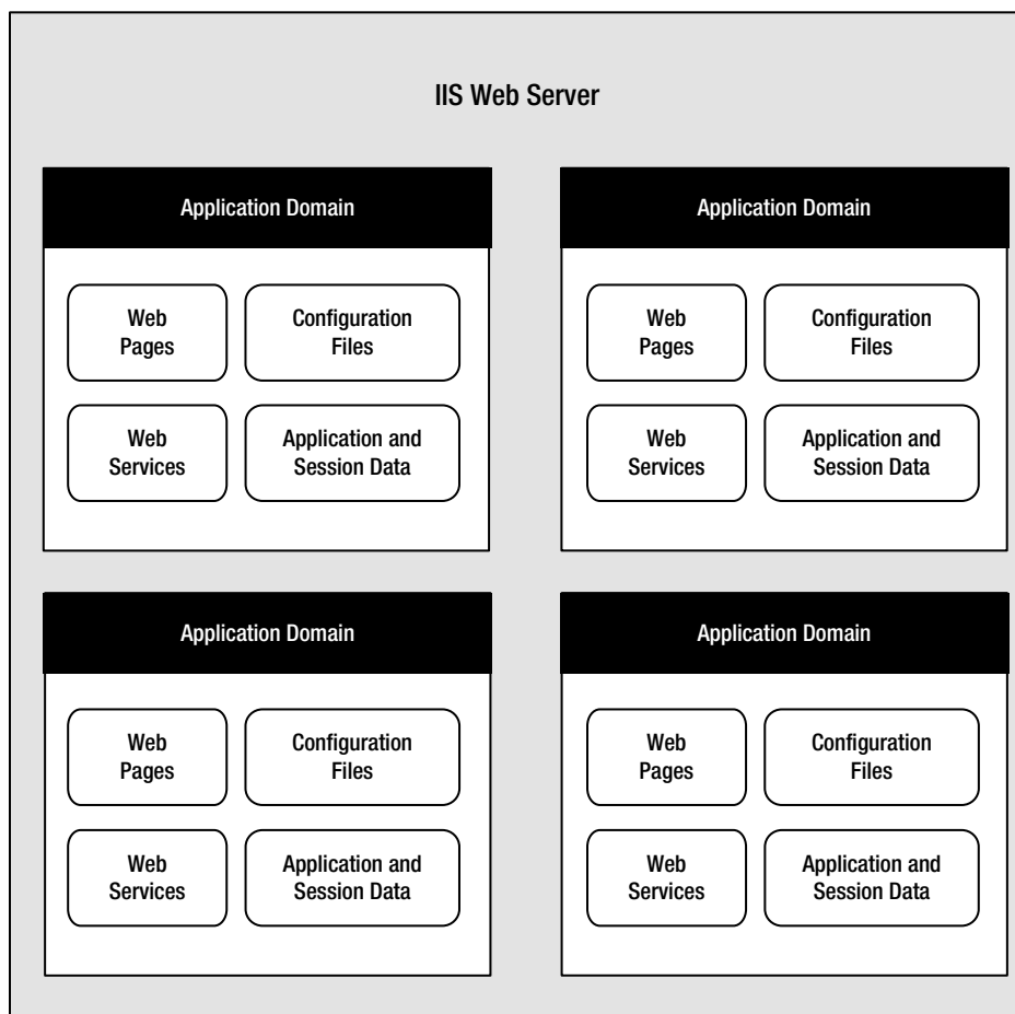
Figure 5-1. ASP.NET applications
