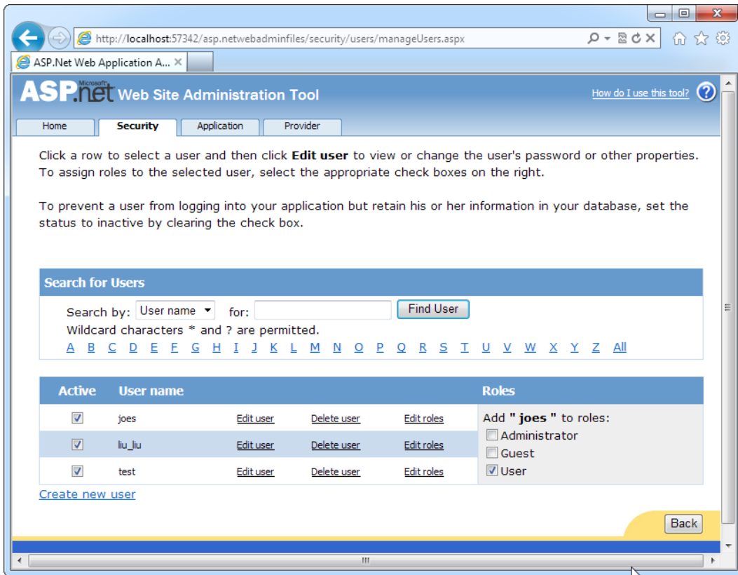
Figure 20-14. Applying roles
