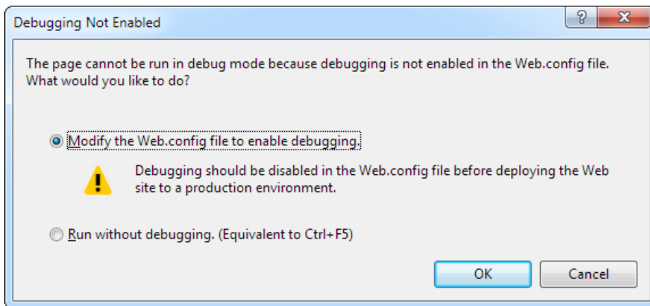
Figure 4-21. Enabling debugging
