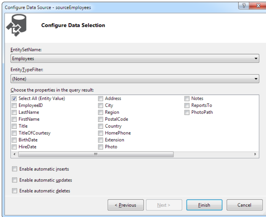
Figure 24-15. Choosing columns
