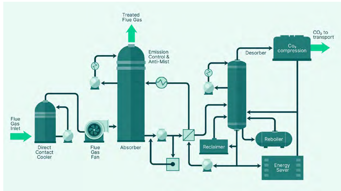
Aker Carbon Capture's Advanced Carbon Capture (ACC™)
