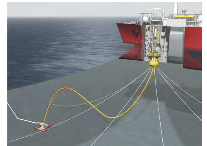
Submerged Turret Loading
