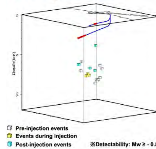
Fig. 5 Results of micro-seismicity of monitoring
