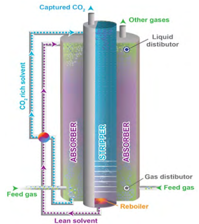
Figure 2: KC8 patented concentric absorption / stripping column configuration
