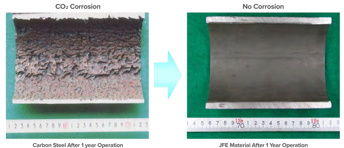
Figure 1: Example of CO 2 Corrosion
