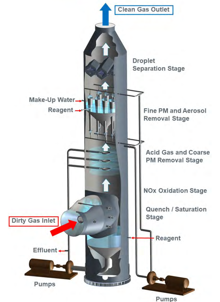
TYPICAL BELCO® WET SCRUBBER
