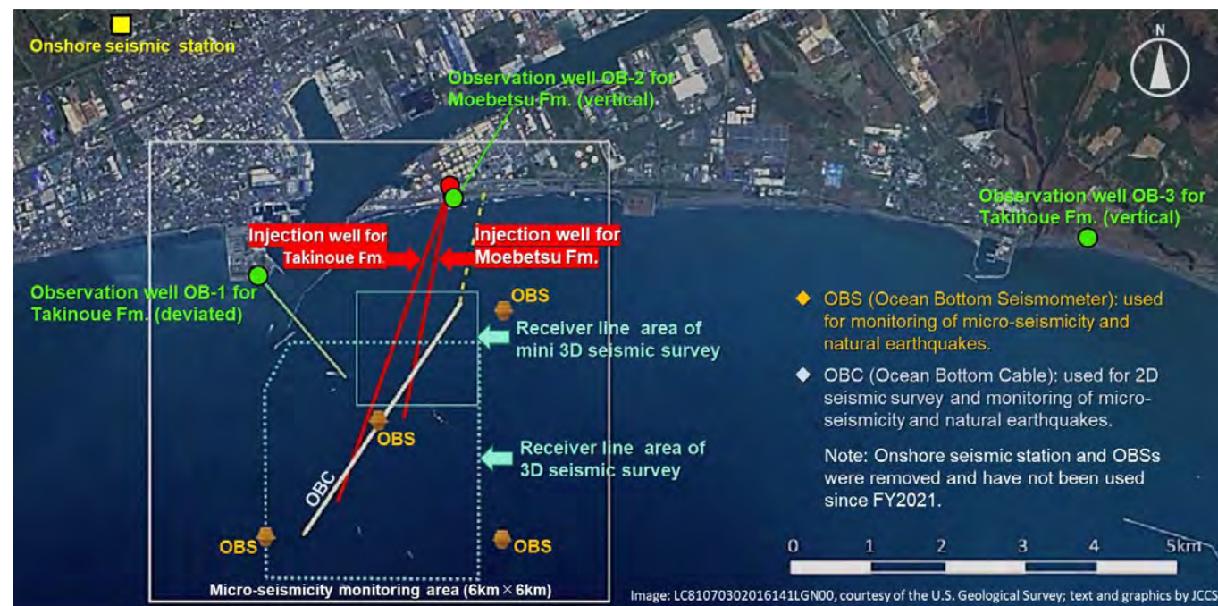
Fig. 4 Layout of monitoring system of the project
