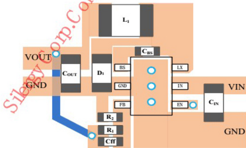
Figure4. PCB Layout Suggestion
