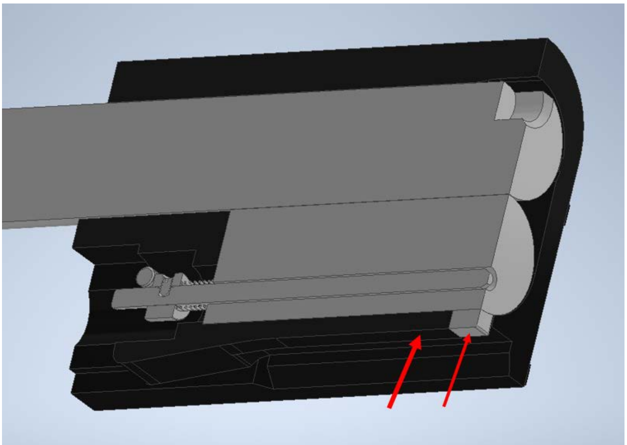
Figure 11: The height of the bottom of the round pickup should align with the height of the rib on the bottom of the bolt housing.
