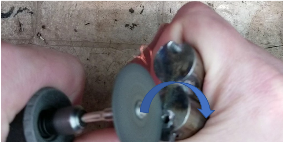
Figure 6: Use gentle, light cuts in an arc around the firing pin hole to round out the edges of the hole.
