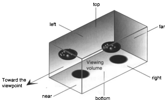
Figure 3-15 Orthographic Viewing Volume
