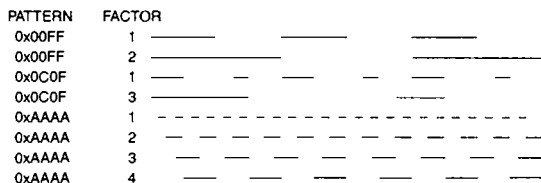
Figure 2-8 Stippled Lines
