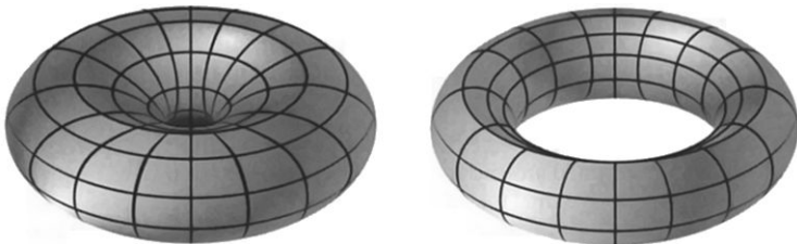
Figure 9-9 Texture-Map Distortion
