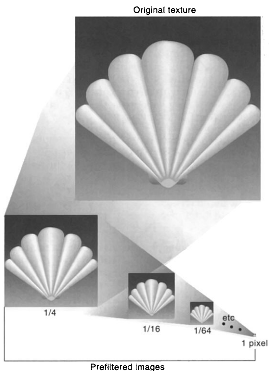
Figure 9-6 Mipmaps
