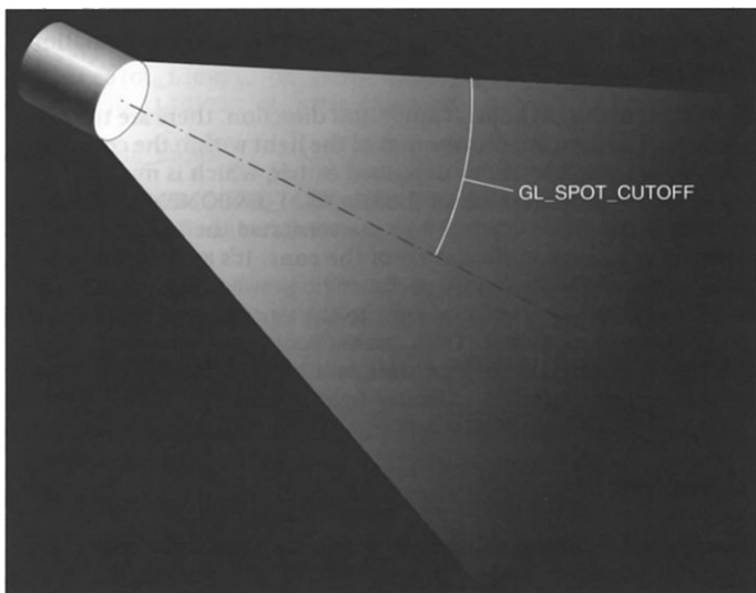
Figure 5-2 GL_SPOT_CUTOFF Parameter
