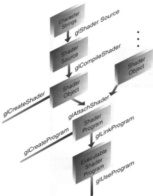
Figure 15-4 Shader Creation Flowchart
