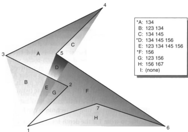
Figure 14-2 Concave Polygon
