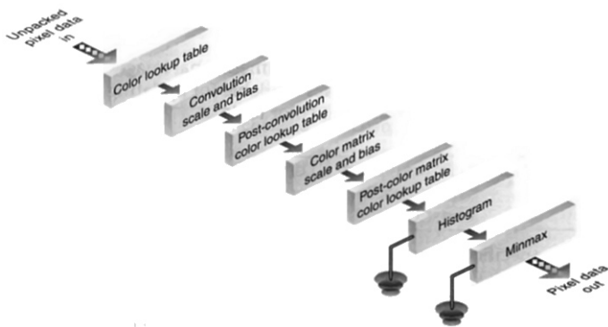
Figure 8-14 Imaging Subset Operations
