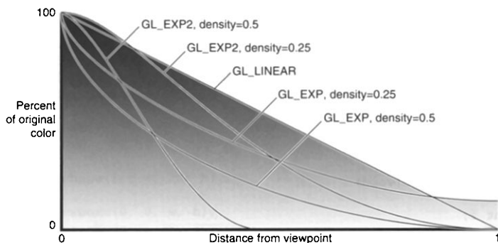
Figure 6-4 Fog-Density Equations
