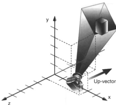
Figure 3-12 Using gluLookAt()
