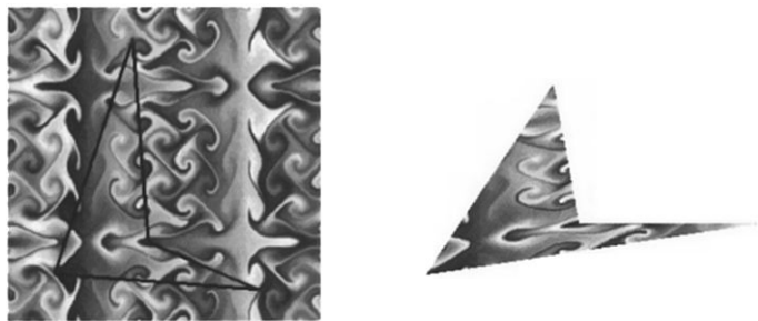
Figure 9-1 Texture-Mapping Process
