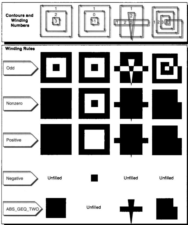
Figure 11-3 How Winding Rules Define Interiors
