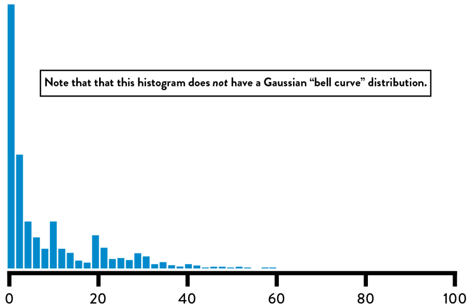
Figure 31: Downloads per minute: histogram of data showing non-Gaussian distribution
