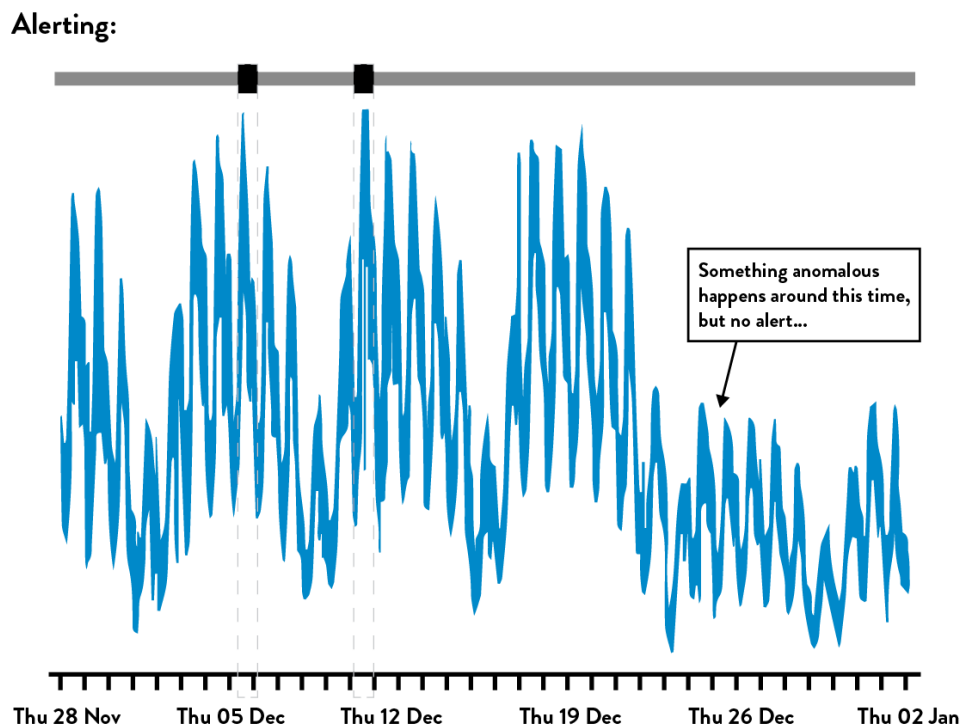
Figure 35: Transaction volume: under-alerting using “3 standard deviation” rule
