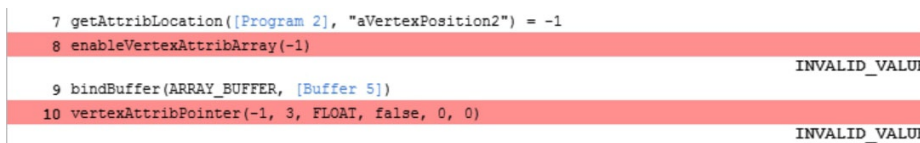
Figure 9-16. WebGL inspector error caused by invalid attribute location value
