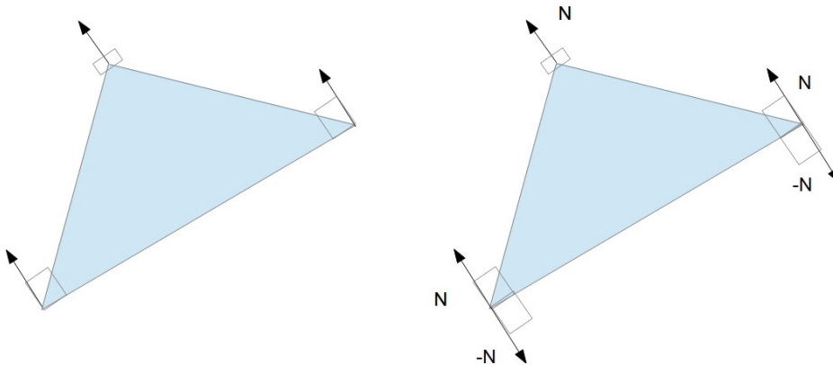
Figure 3-15. A triangle with vertex normal vectors (all identical in value) that are perpendicular to the triangle surface. Two of the three negative normals are visible on the right
