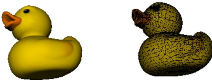
Figure 8-6. Left: rendering of a rubber duck; right: wireframe overlaid on image, showing hundreds of triangles that comprise it
