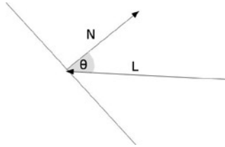
Figure 4-6. The normal ( N ) and lighting ( L ) vectors of a Lambert reflection
