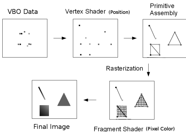
Figure 2-2. WebGL rendering process overview
