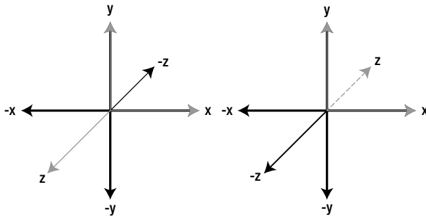
Figure B-2. Two distinct 3D coordinate system orientations
