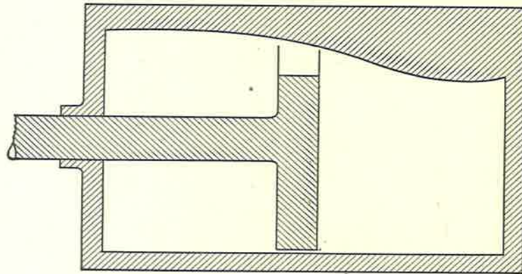
FIG. 8. Hydraulic Brake.
