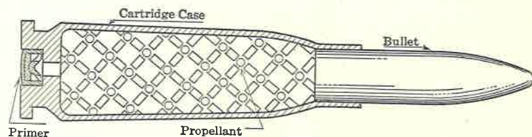
FIG. 1. Cartridge Components.
