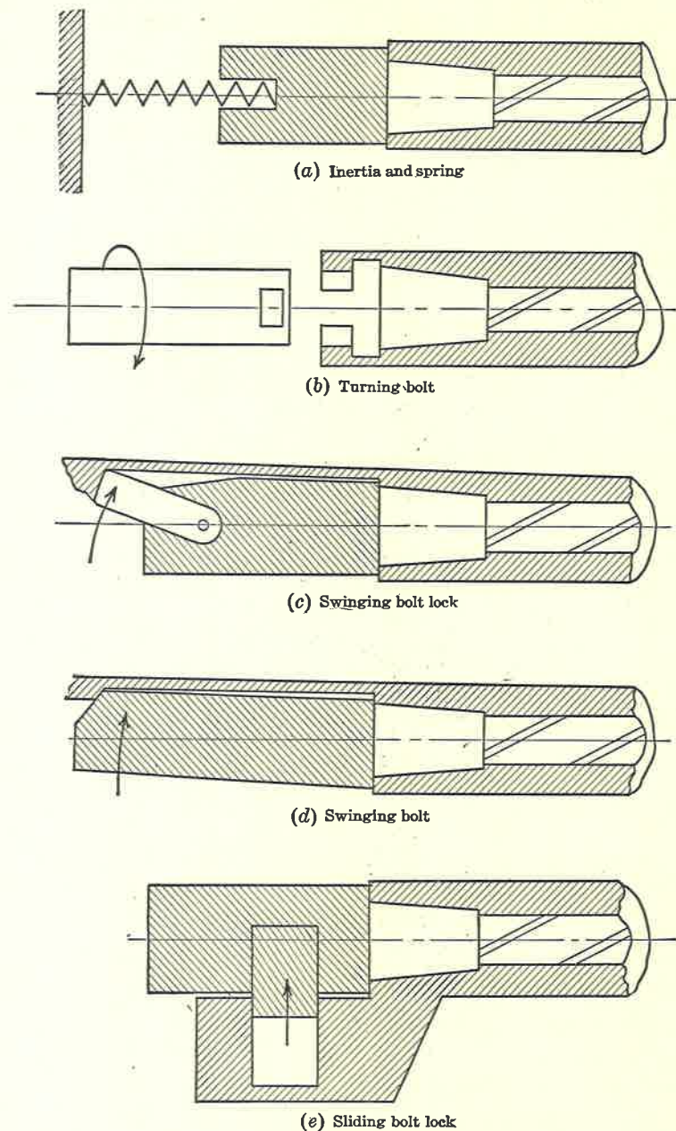
FIG. 10. Types of Locks.
