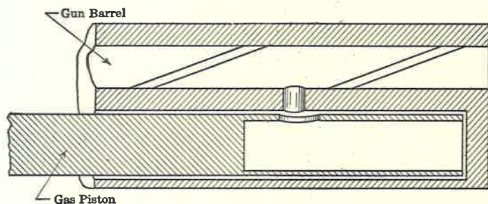
FIG. 20. Gas Expansion System (White).
