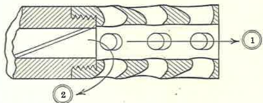
FIG. 7. Muzzle Brake.
