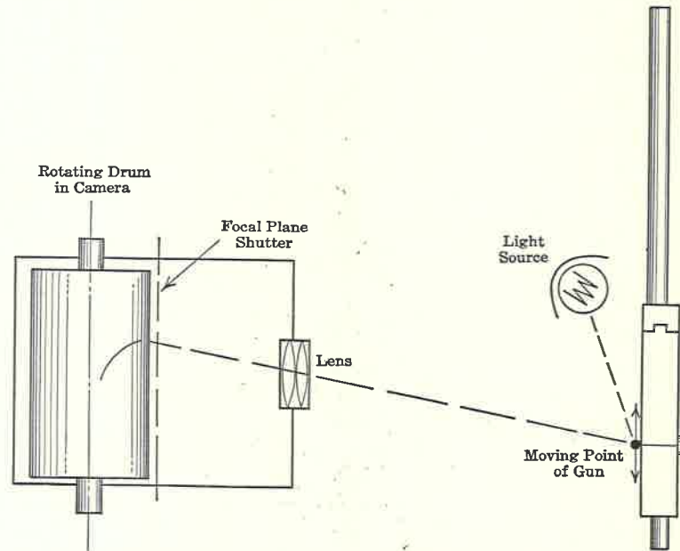
FIG. 50. Time-Displacement Camera.
