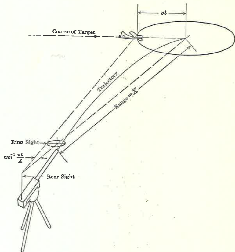
FIG. 43. Principle of Ring Sight.
