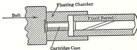
FIG. 23. Floating Chamber System.
