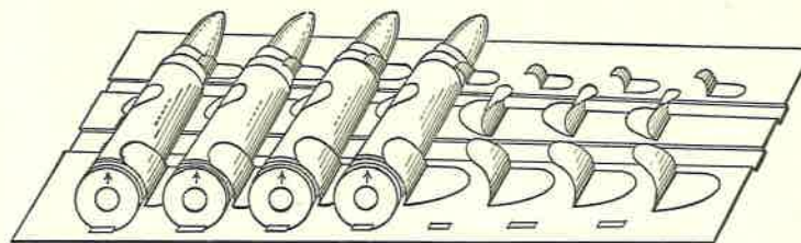
FIG. 38. Feed Strip (Hotchkiss).
