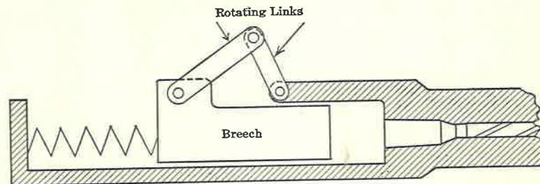
FIG. 15. Action of Schwarzlose Machine Gun.
