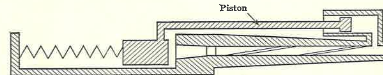
FIG. 18. Elementary Gas-Operated Gun.
