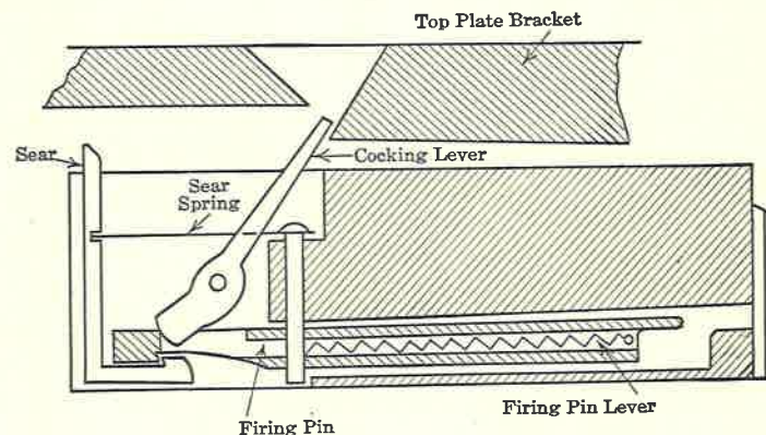
FIG. 27. Browning Machine Gun—Firing Chain.
