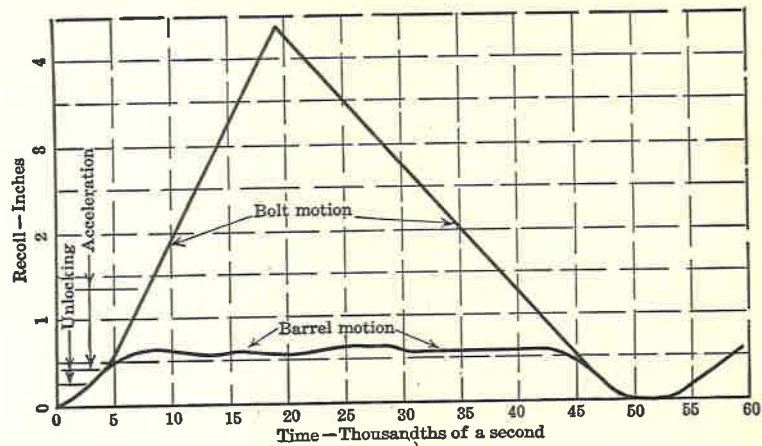
FIG. 26. Browning Machine Gun—Time-Displacement Curves.
