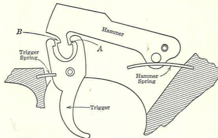
FIG. 34. Semiautomatic Mechanism—Browning.
