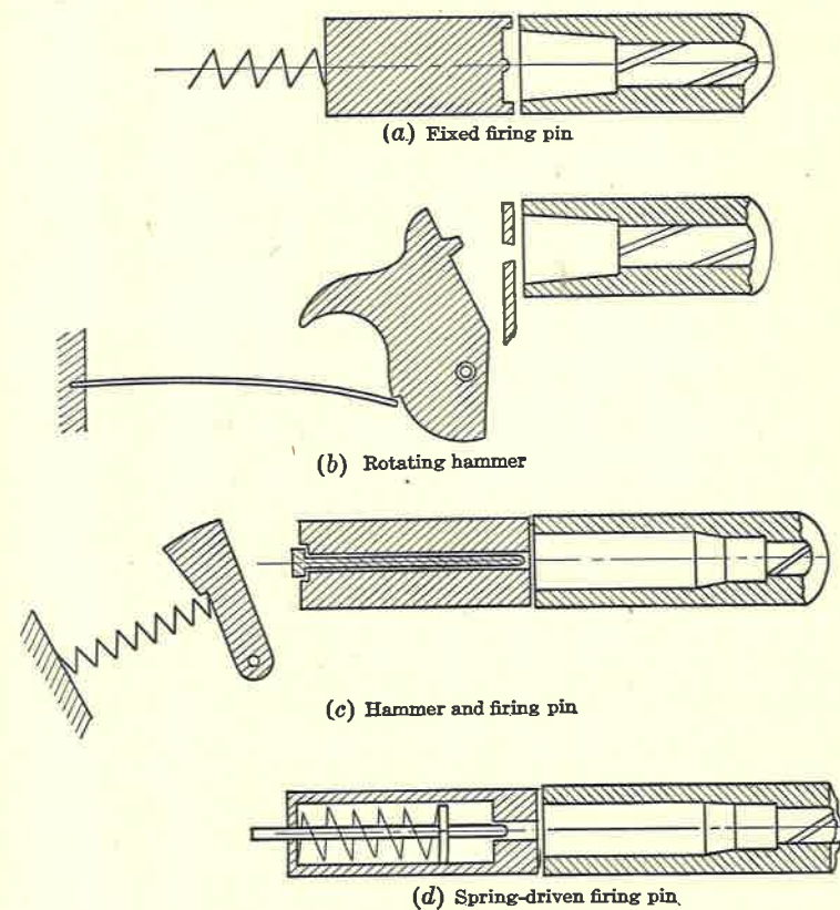
FIG. 11. Firing Arrangements.
