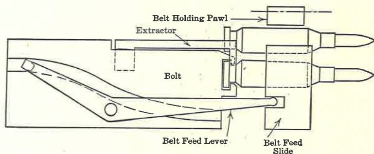
FIG. 28. Browning Machine Gun—Belt Moving Chain.
