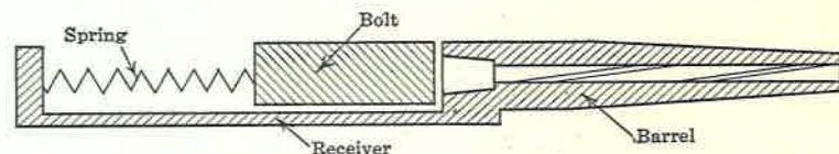
FIG. 14. Elementary Inertia Action.
