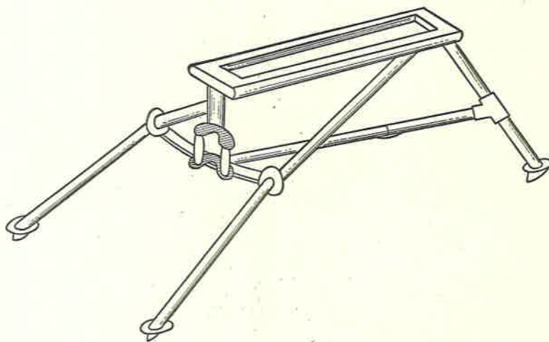
FIG. 55. German Type Tripod.
