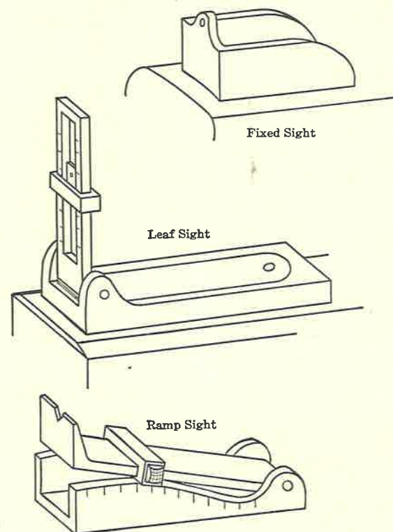
FIG. 44. Rear Sights.
