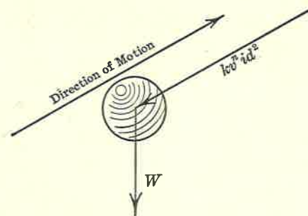
FIG. 52. Forces on Projectile.
