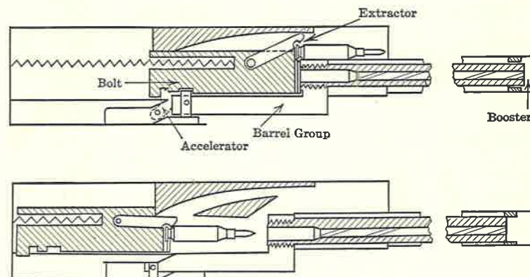
FIG. 25. Browning Machine Gun—Feeding Chain.
