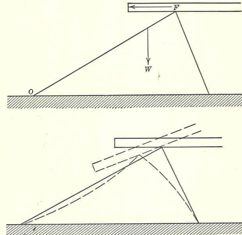
FIG. 53. Force System on Mount.
