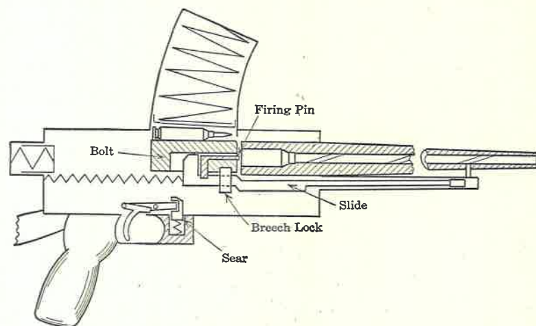
FIG. 30. Japanese Light Machine Gun, Model 99.
