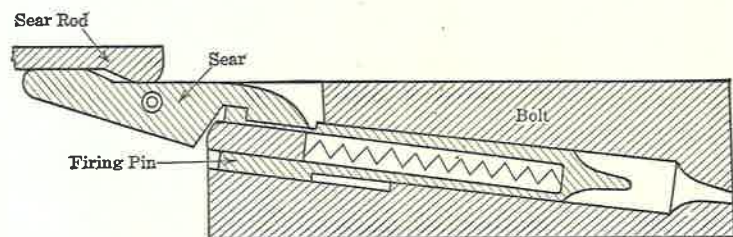
FIG. 33. Fowler Firing Pin Mechanism.
