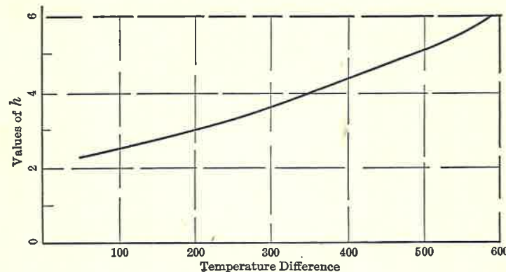
FIG. 5. Radiation and Convection from a Gun Barrel.
