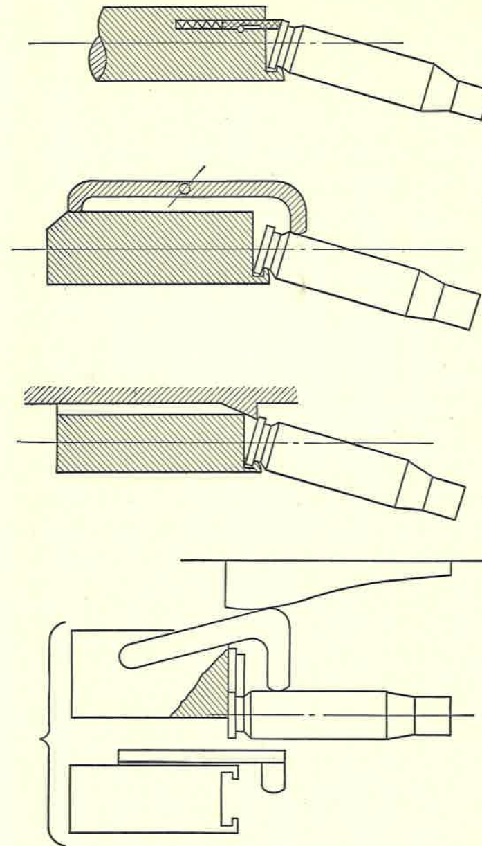
FIG. 13. Types of Ejectors.
