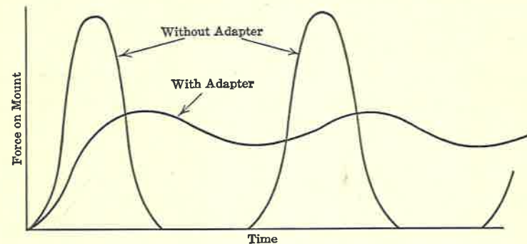
FIG. 54. Effect of Recoil Adapter.
