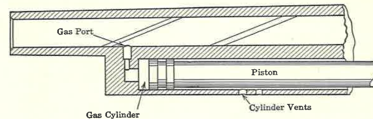
FIG. 19. Gas Port and Piston.
