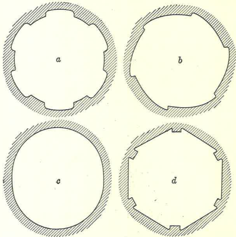
FIG. 4. Forms of Rifling.
