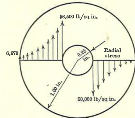
FIG. 3. Stress Distributions in Gun Tube.
