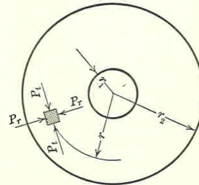
FIG. 2. Stress Definitions.
