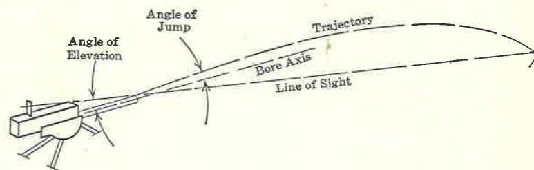
FIG. 41. Effect of Jump on Sights.
