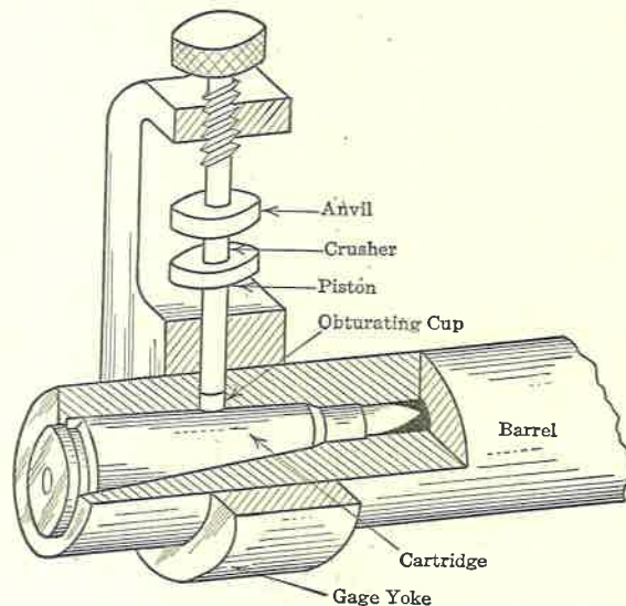
FIG. 46. Crusher Pressure Gage.
