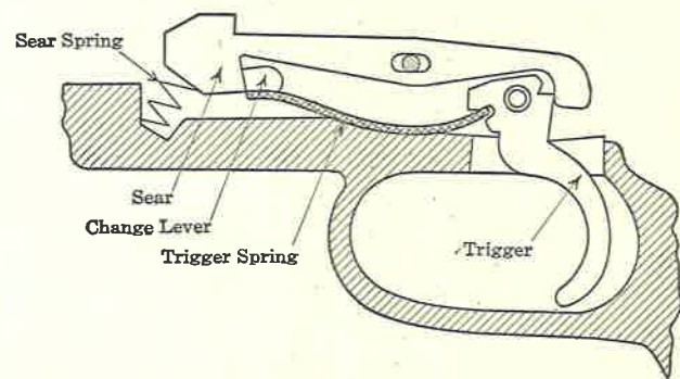
FIG. 35. Convertible Trigger Mechanism (Mendoza).
