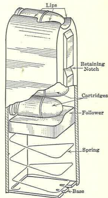
FIG. 36. Magazine.
