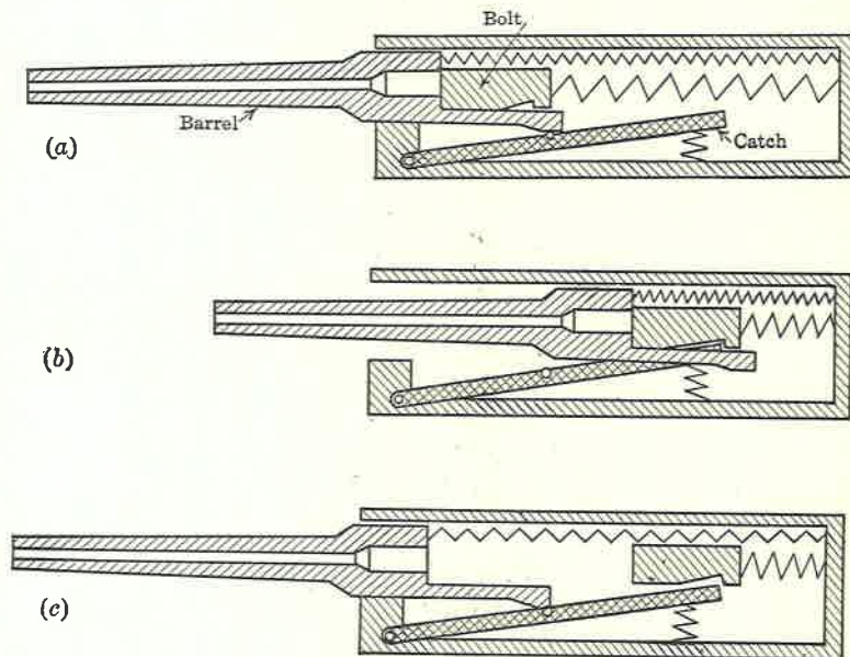
FIG. 17. Elementary Long Recoil Action.
