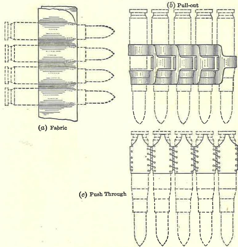
FIG. 37. Feed Belts.
