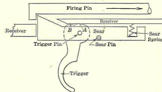
FIG. 32. M1903 Rifle Trigger Mechanism.
