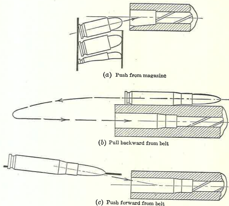
FIG. 9. Methods of Feeding.
