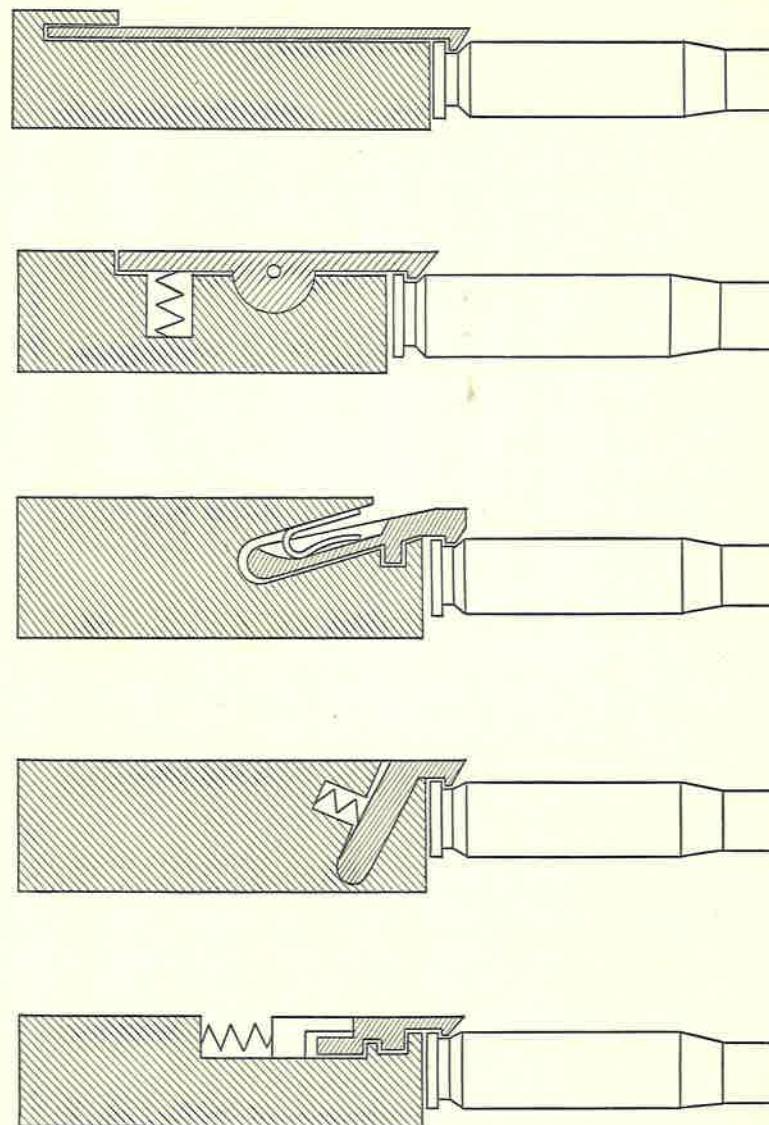
FIG. 12. Types of Extractors.
