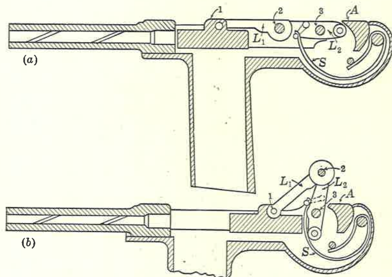
FIG. 16. Short Recoil Pistol (Borchardt).
