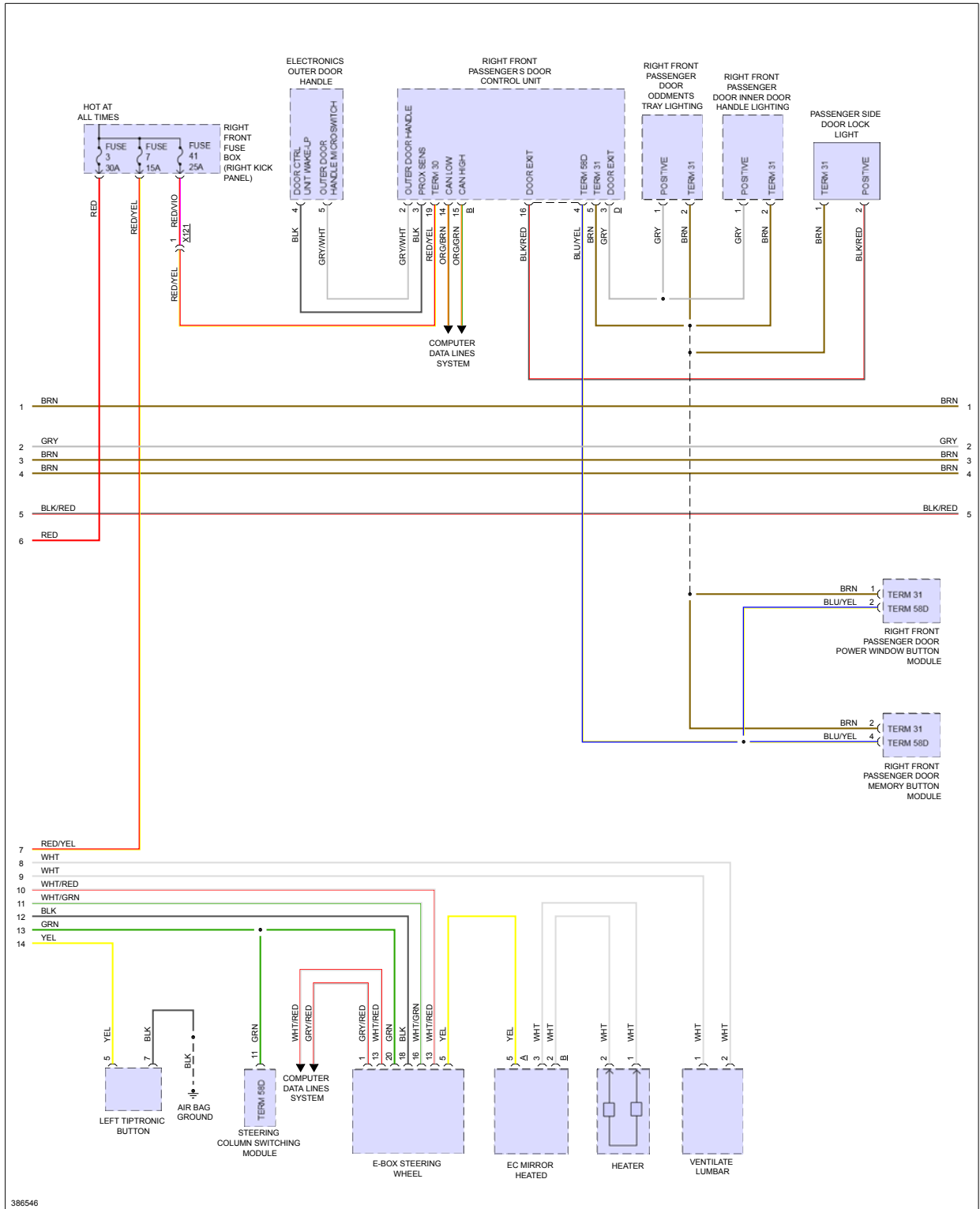
Fig 2: Interior Lights Circuit (2 of 5)
