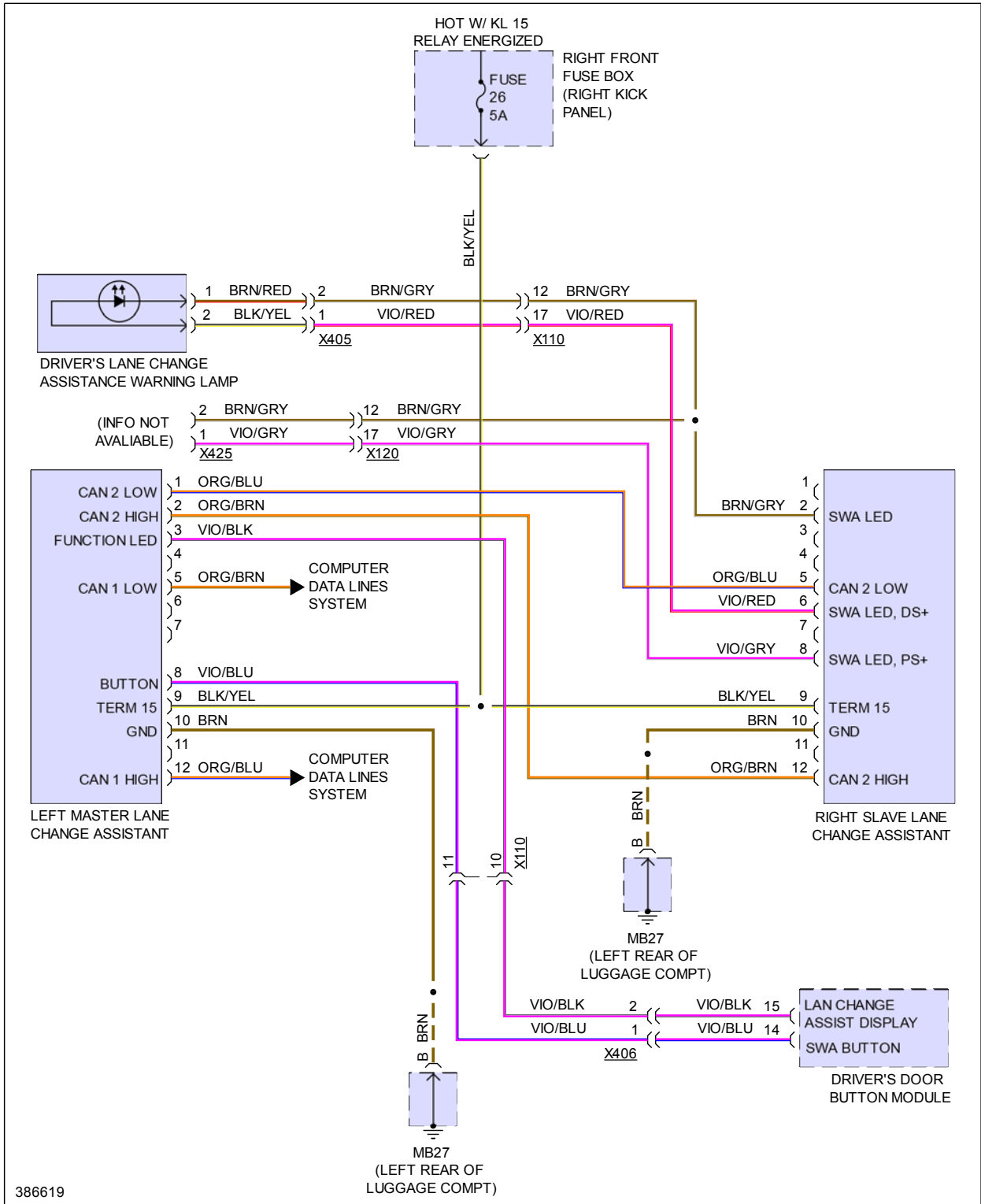
Fig 1: Lane Change Assistance Circuit
