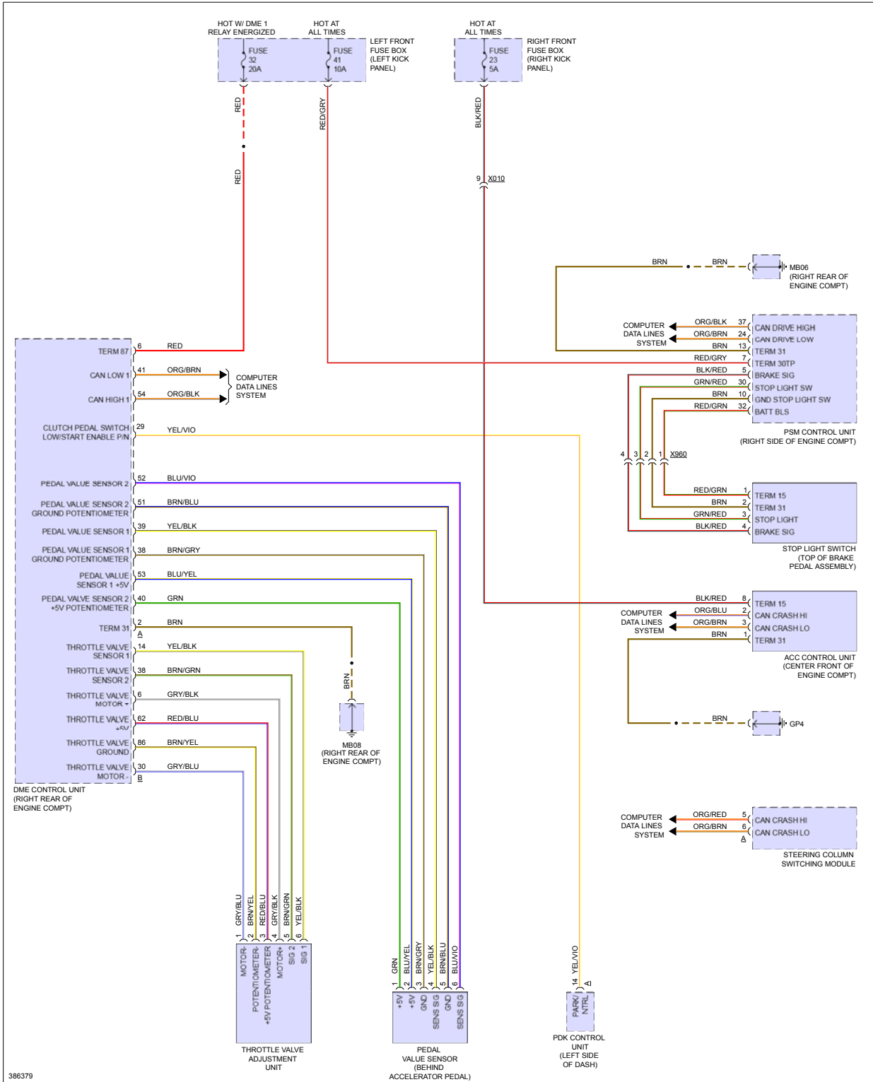
Fig 1: Cruise Control Circuit, Except Hybrid
