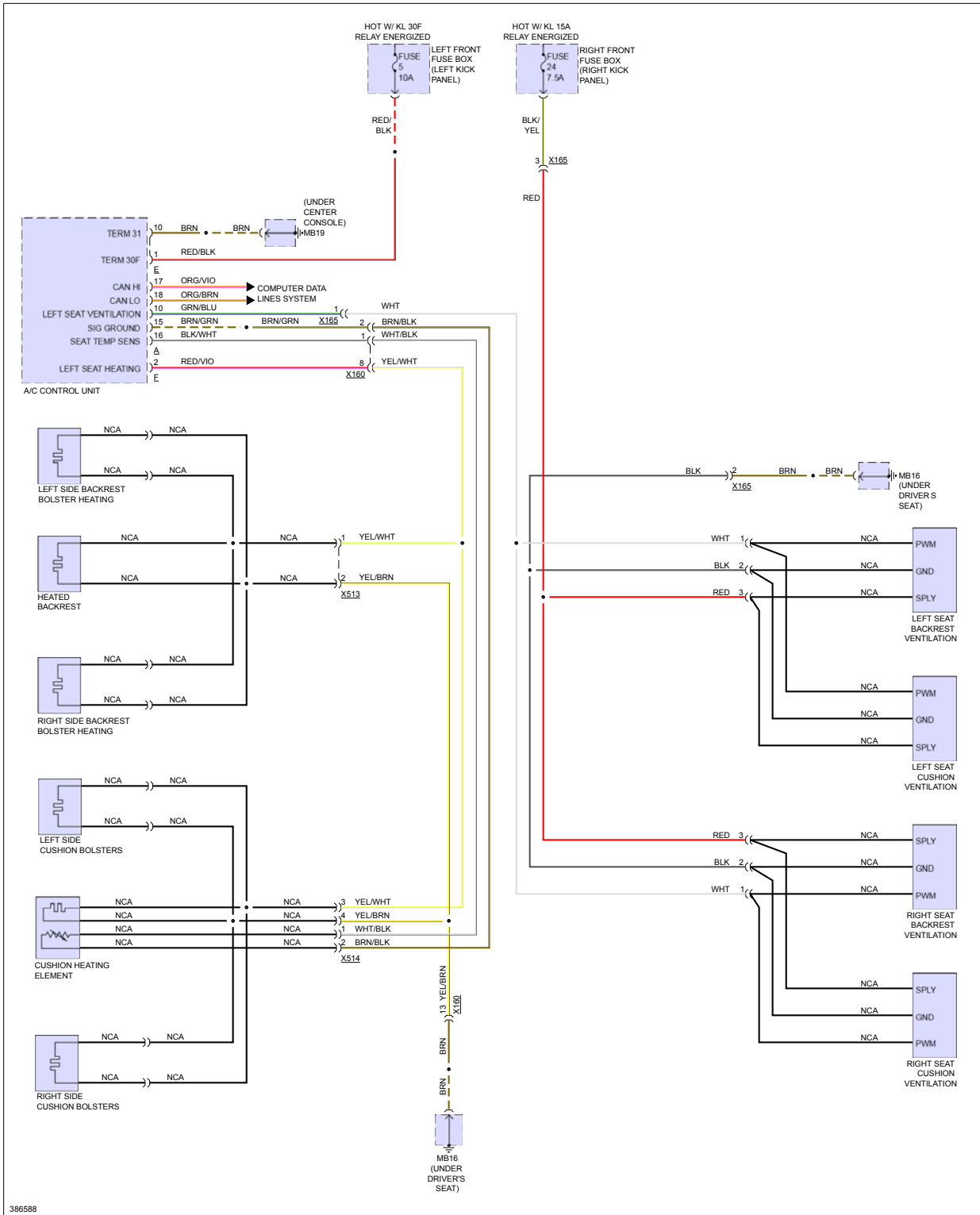
Fig 2: Front Heated Seats Circuit, W/O Passenger Power Seats
