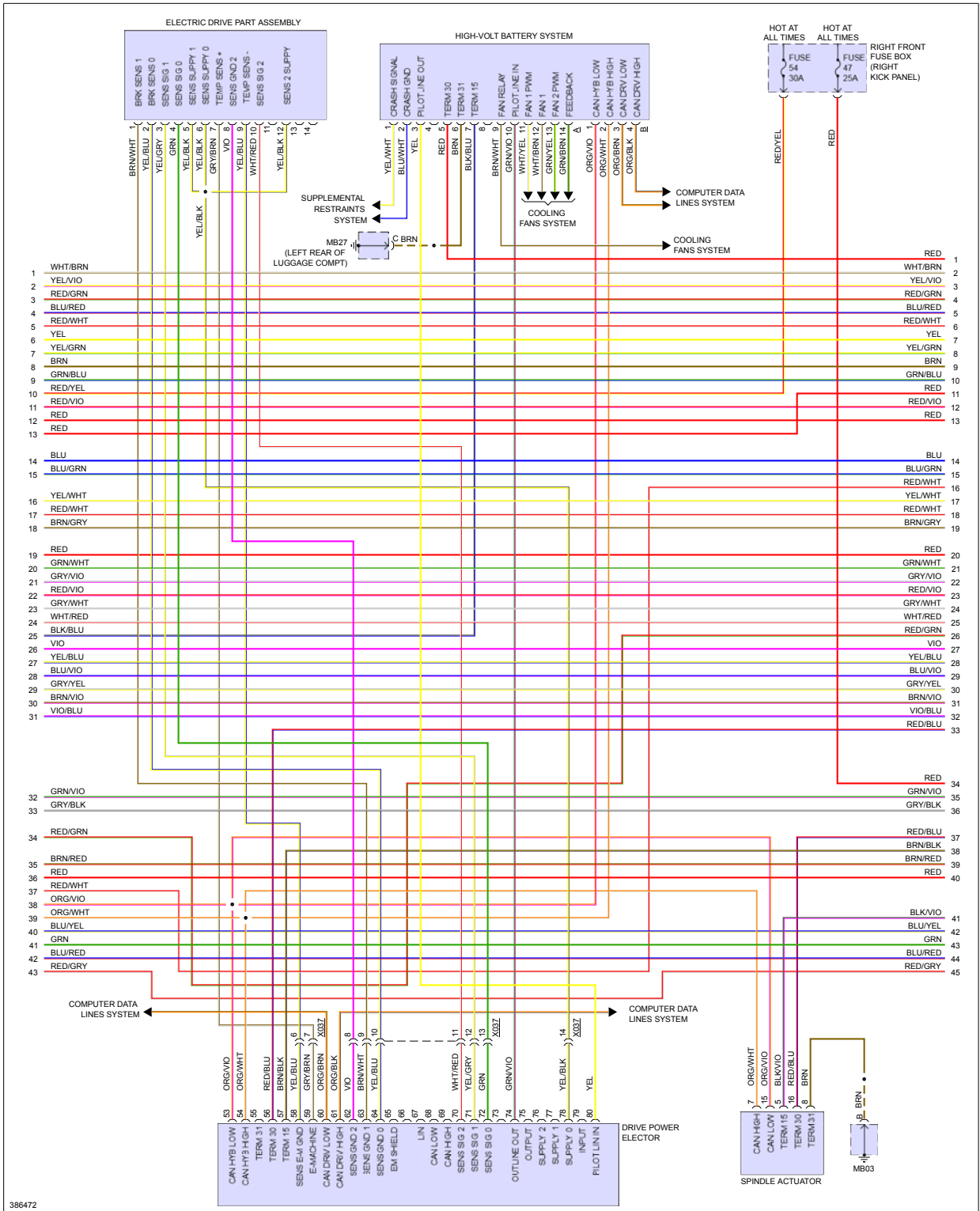
Fig 6: 3.0L Hybrid, Engine Performance Circuit (6 of 7)
