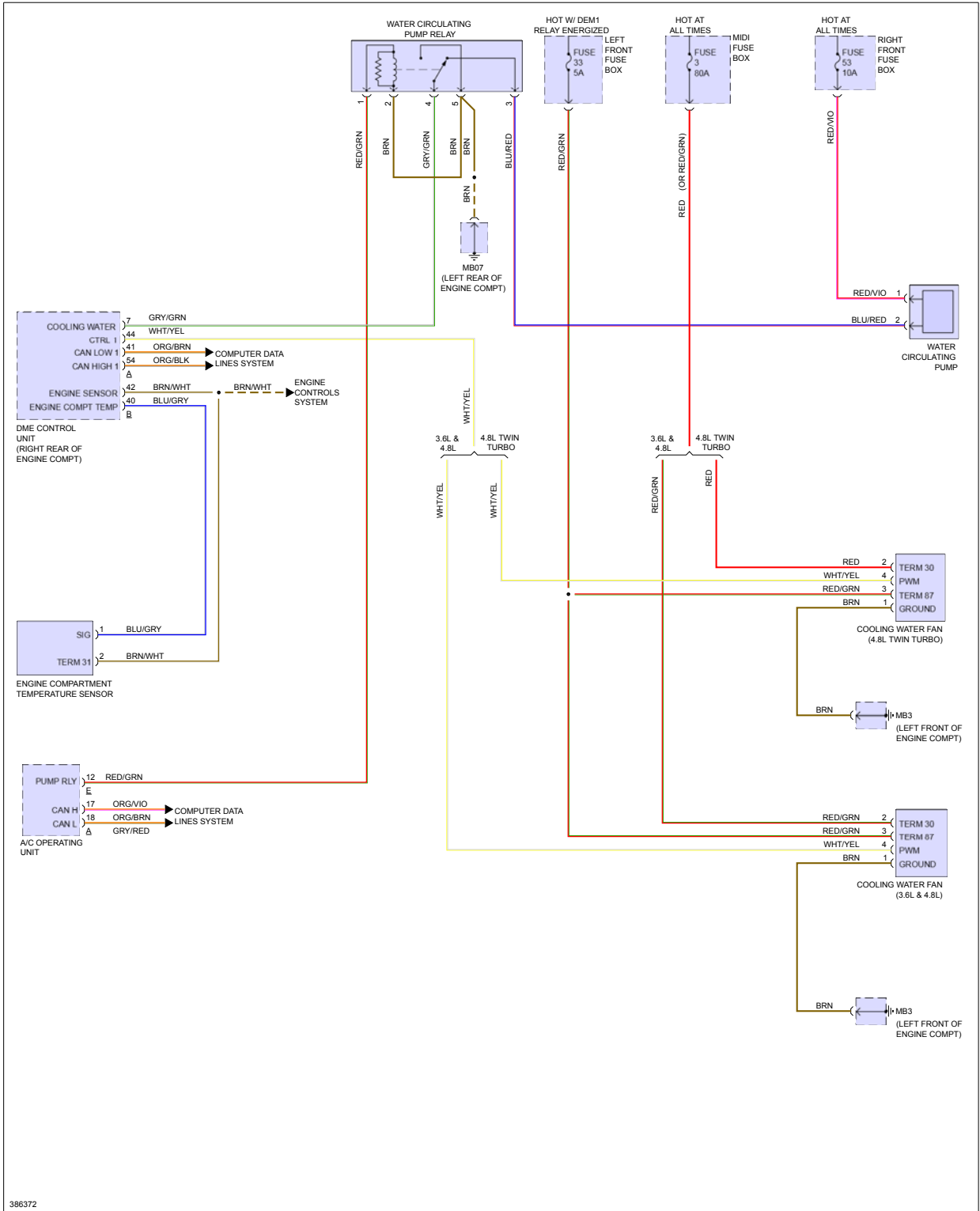
Fig 1: Cooling Fan Circuit, Except Hybrid
