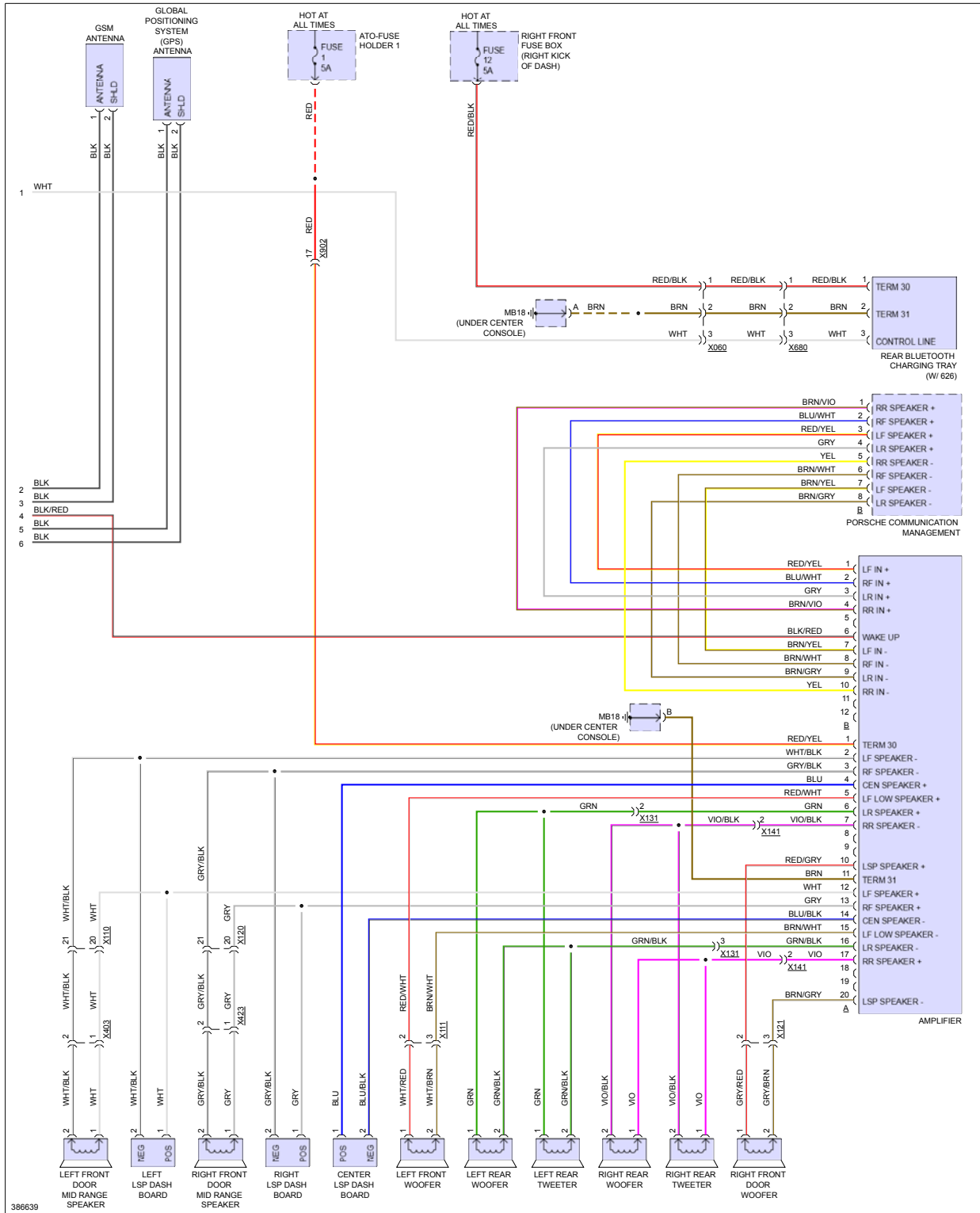
Fig 6: Premium Radio Circuit, W/ ASK (2 of 2)
