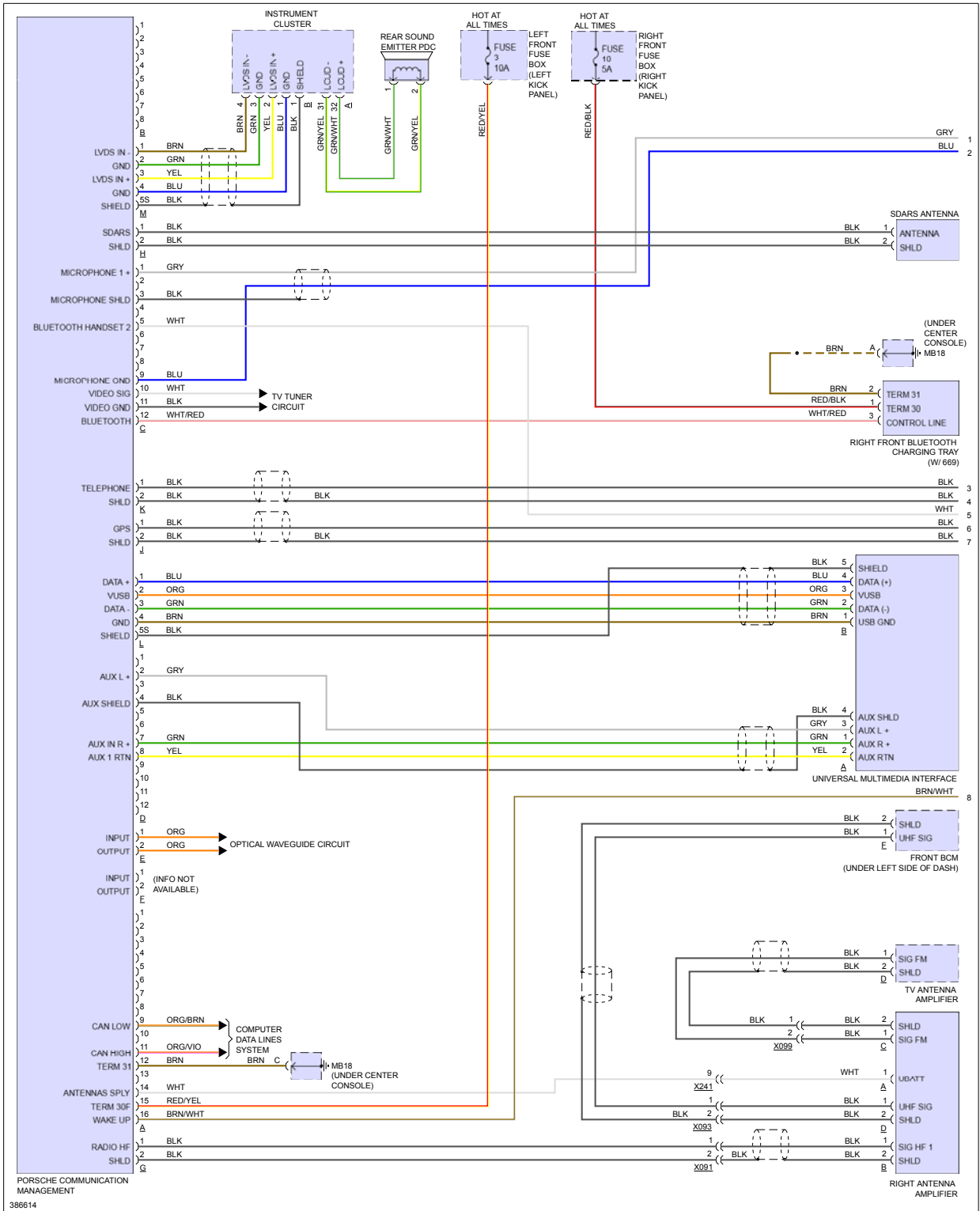
Fig 6: Navigation Circuit, W/ Burmester (1 of 3)
