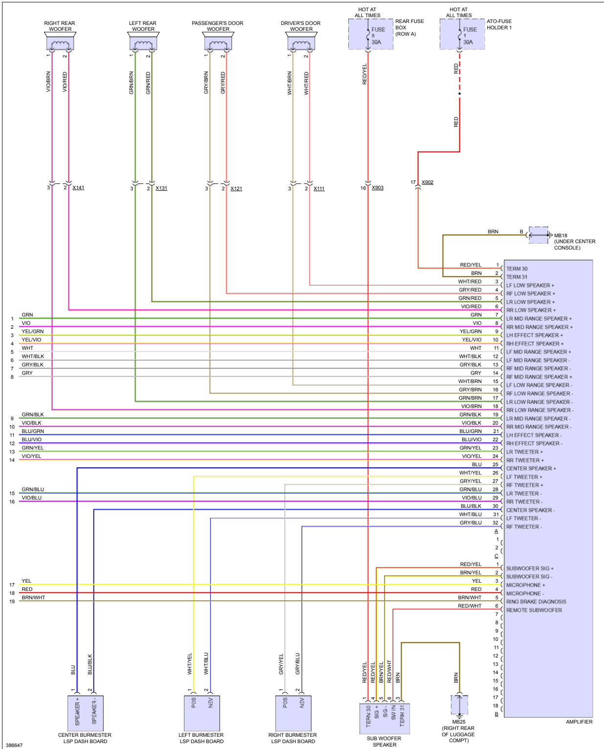
Fig 11: Premium Radio Circuit, W/ Burmester (3 of 3)
