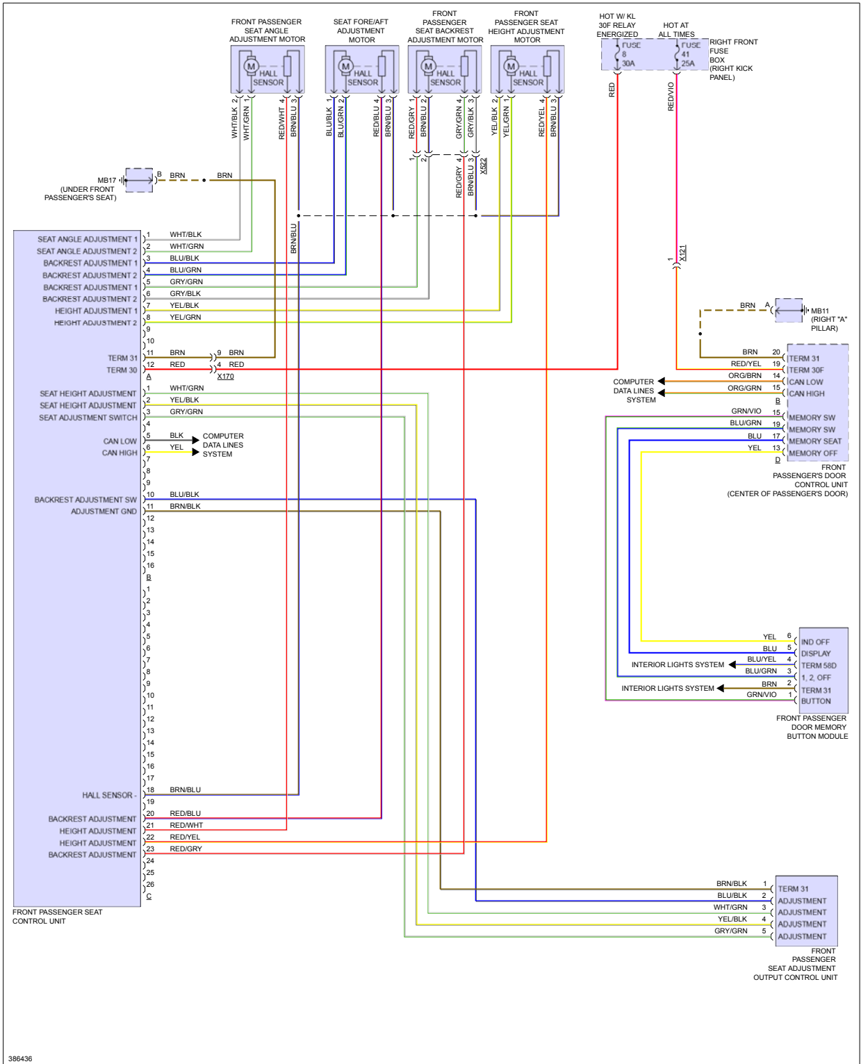
Fig 4: Passenger's Memory Seat Circuit, Except Sport Comfort
