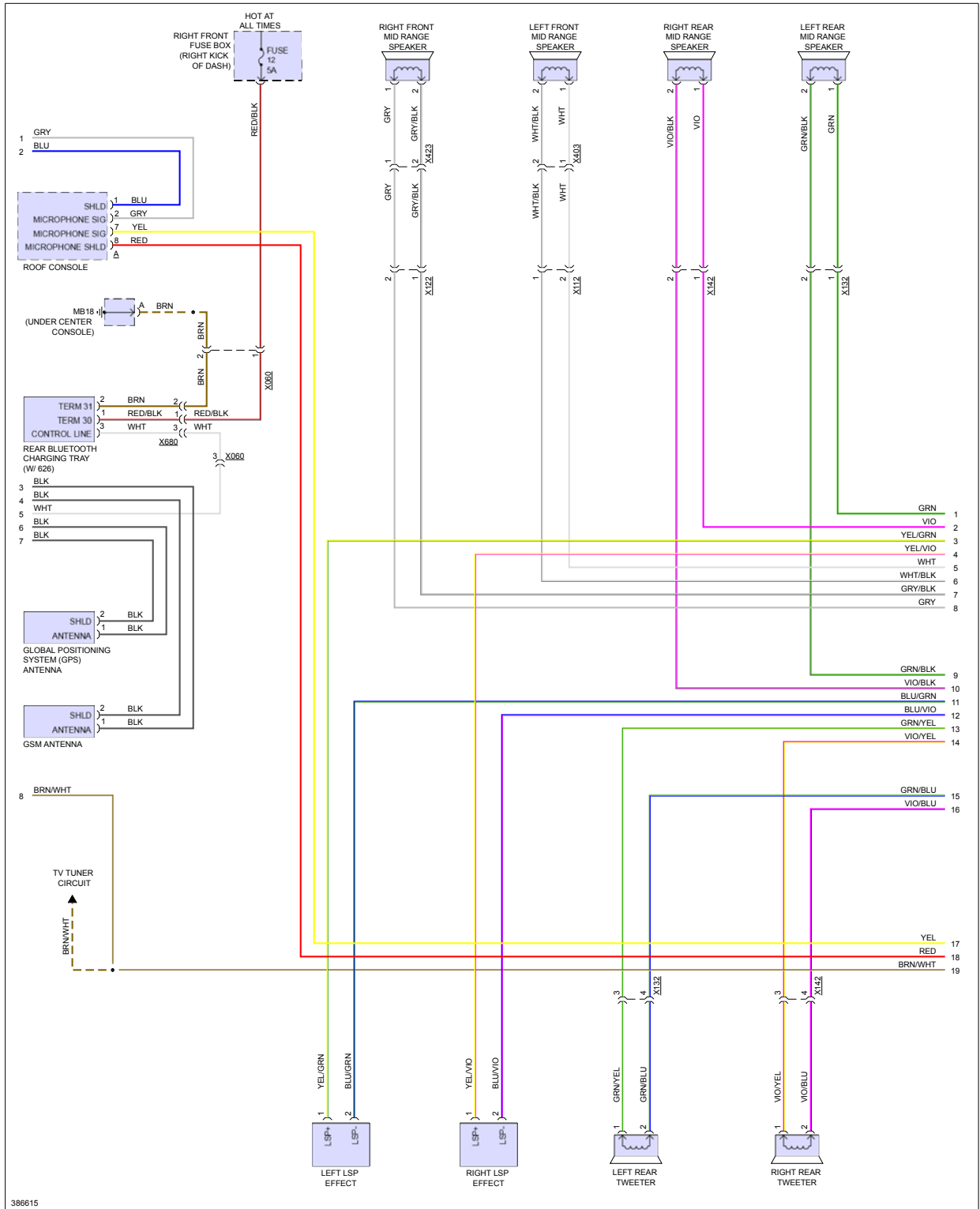
Fig 7: Navigation Circuit, W/ Burmester (2 of 3)
