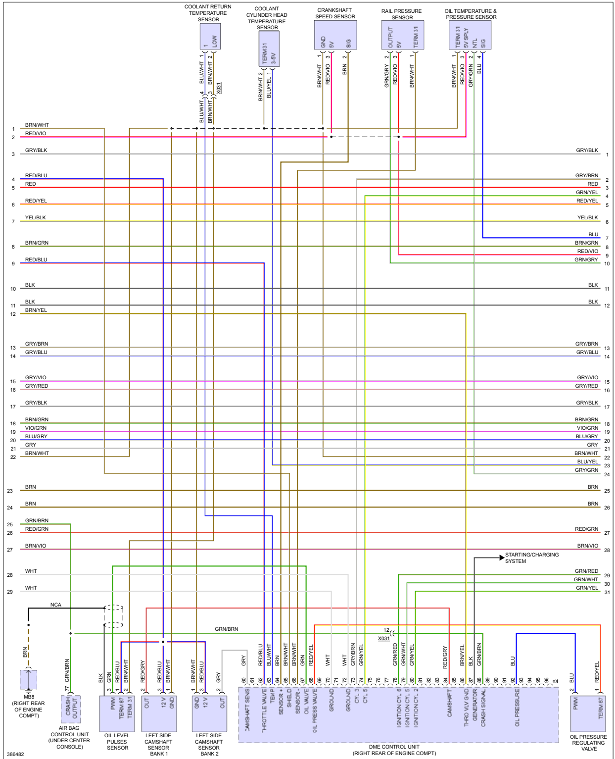
Fig 4: 3.6L, Engine Performance Circuit (4 of 5)
