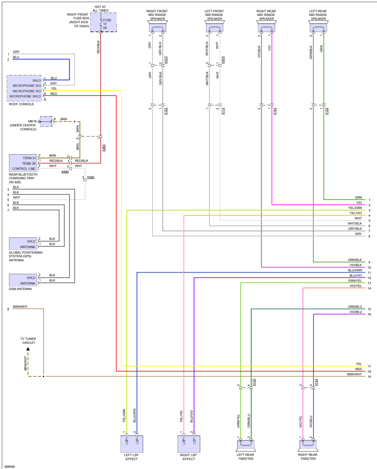
Fig 10: Premium Radio Circuit, W/ Burmester (2 of 3)
