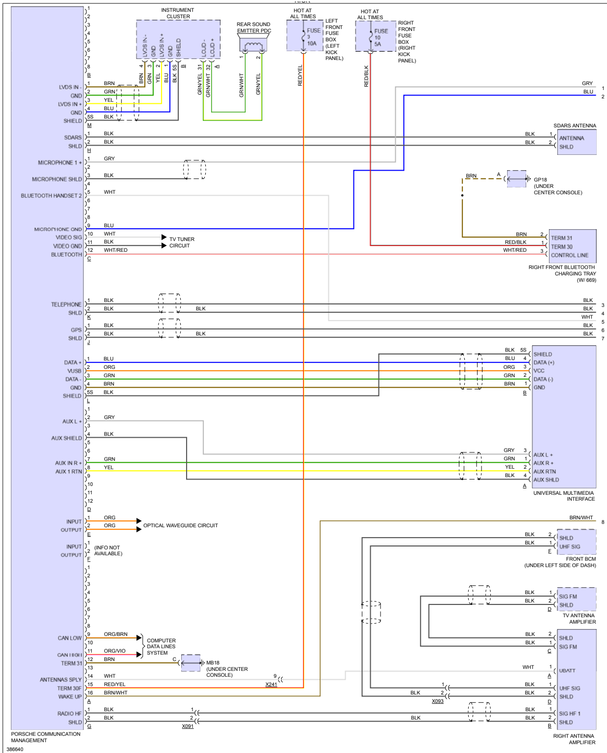
Fig 7: Premium Radio Circuit, W/ Bose (1 of 2)
