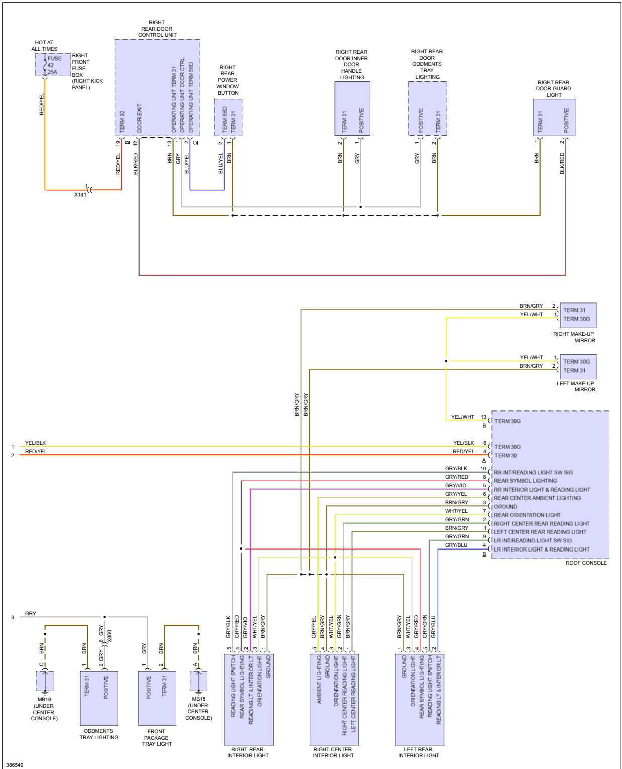
Fig 5: Interior Lights Circuit (5 of 5)
