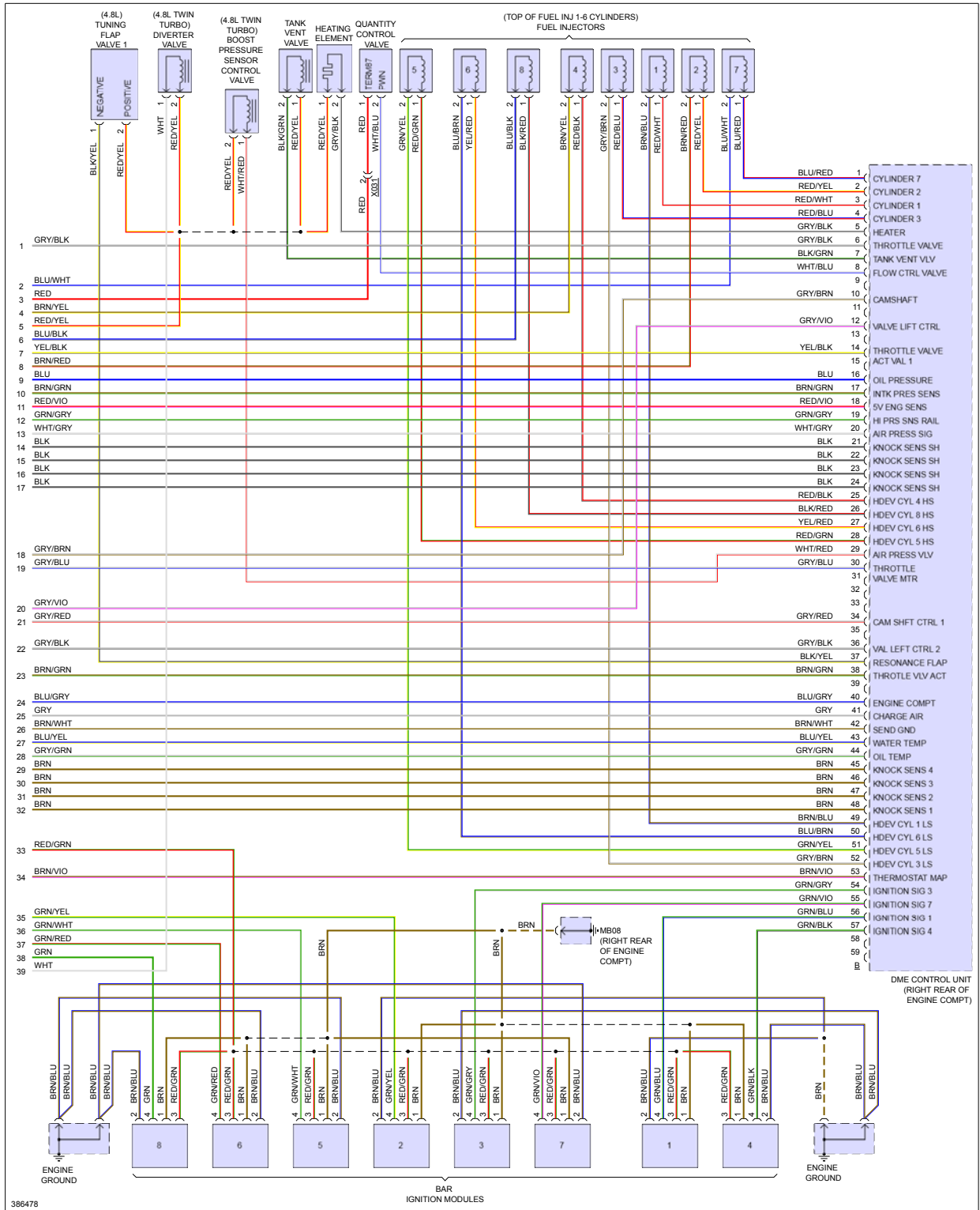
Fig 5: 4.8L, Engine Performance Circuit (5 of 5)
