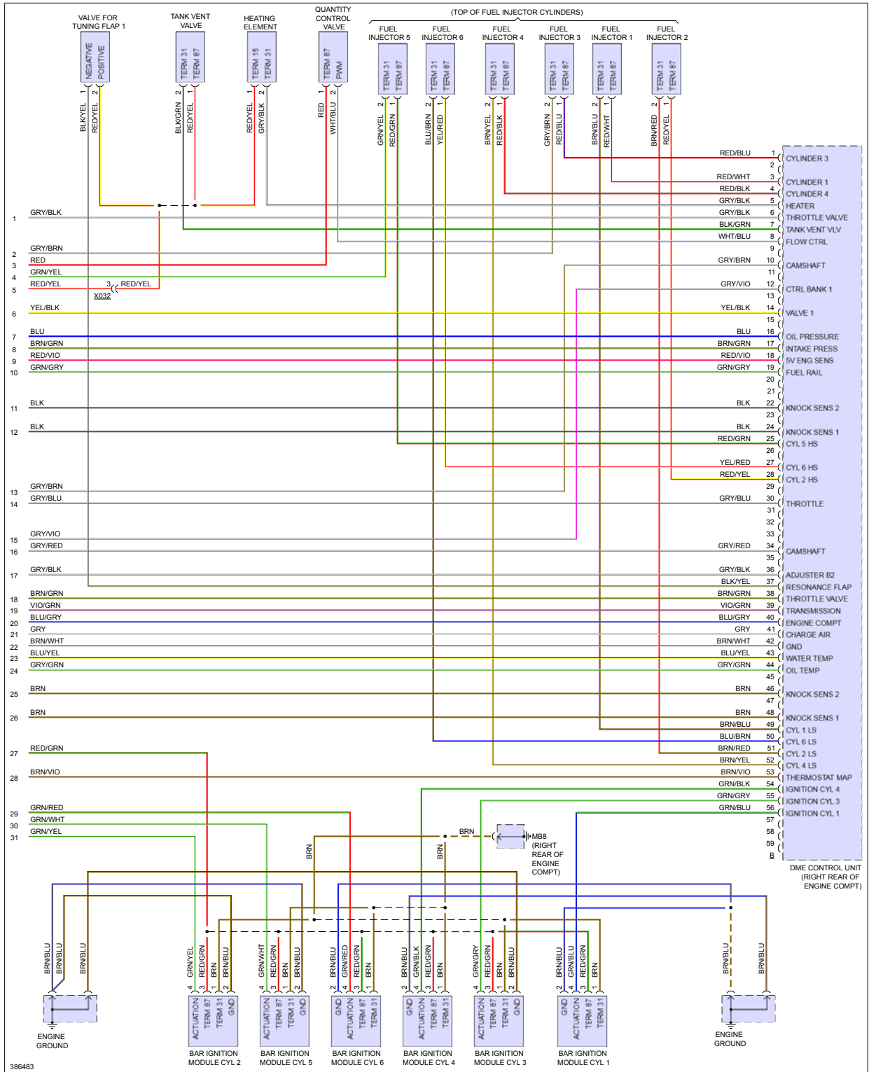
Fig 5: 3.6L, Engine Performance Circuit (5 of 5)
