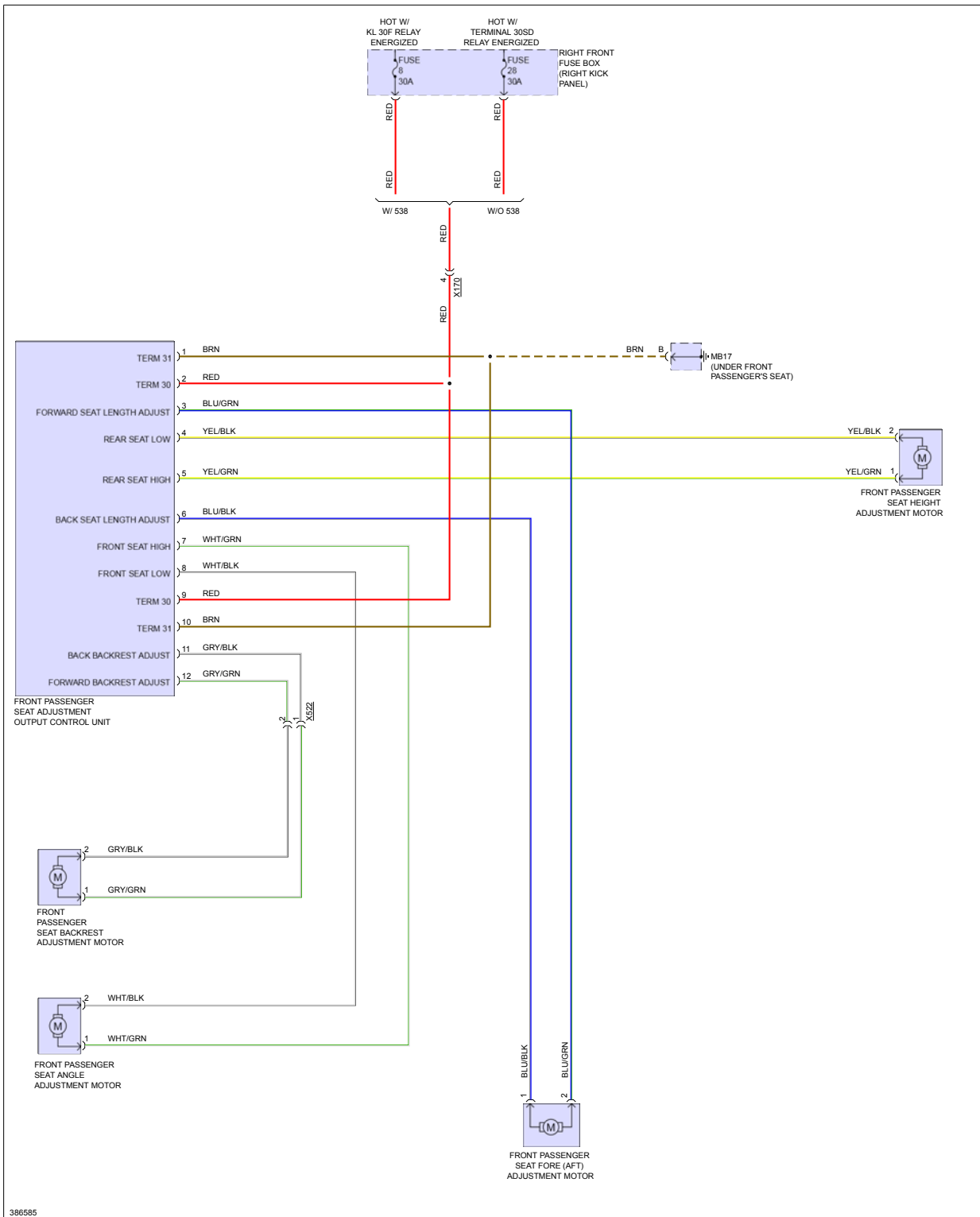
Fig 3: Passenger Power Seat Circuit
