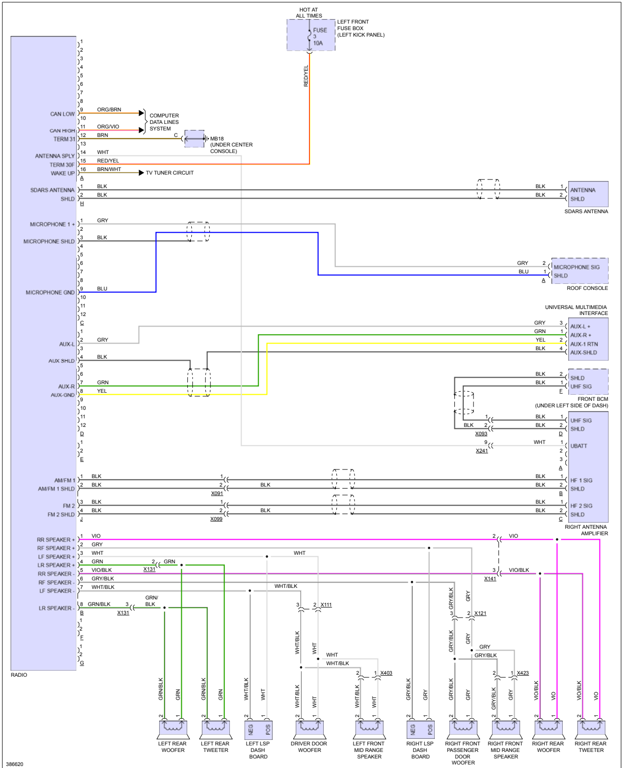
Fig 3: Base Radio Circuit, W/O Amplifier
