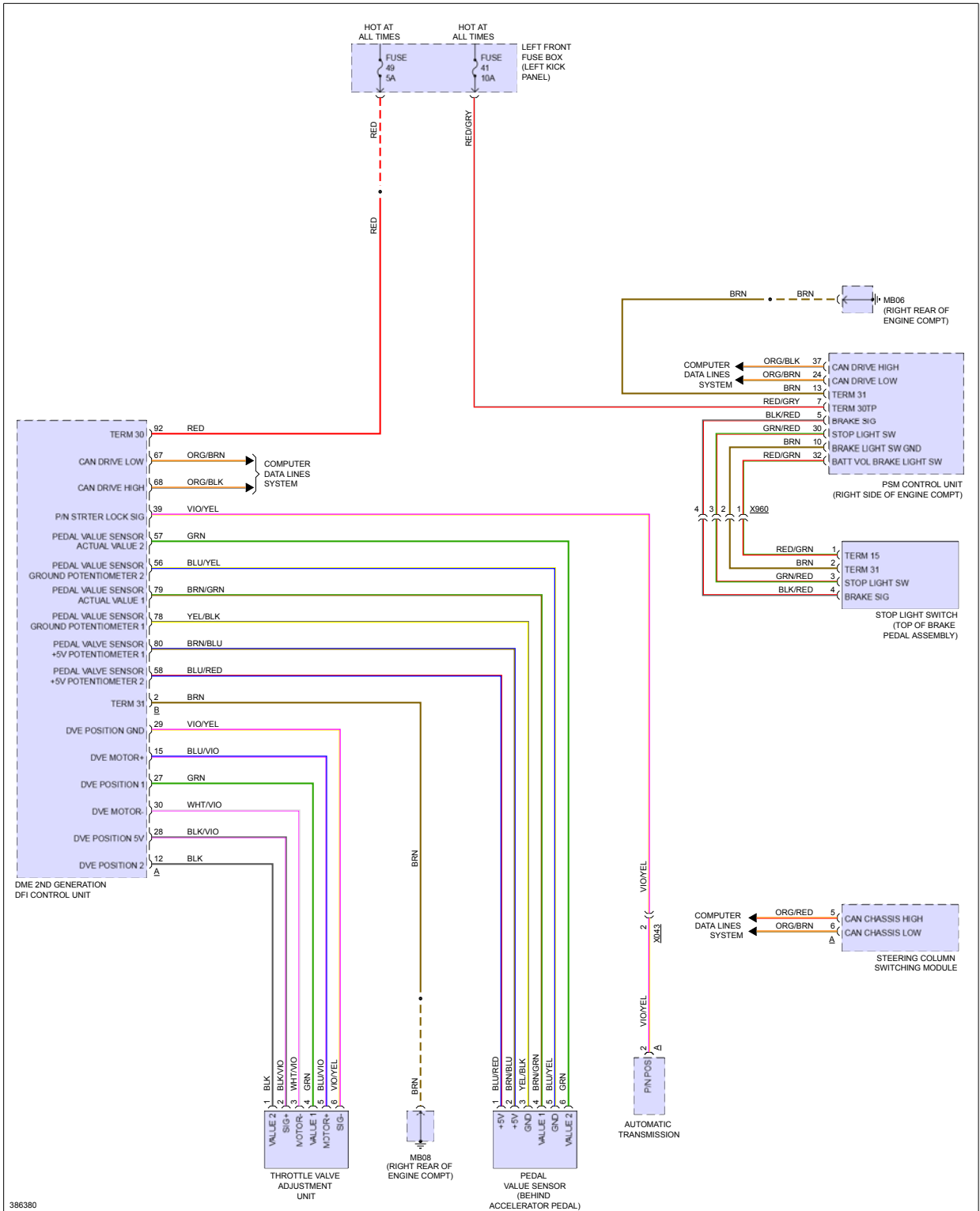
Fig 2: Cruise Control Circuit, Hybrid
