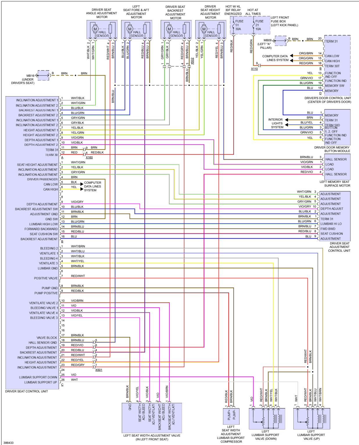
Fig 2: Driver's Memory Seat Circuit, Sport Comfort
