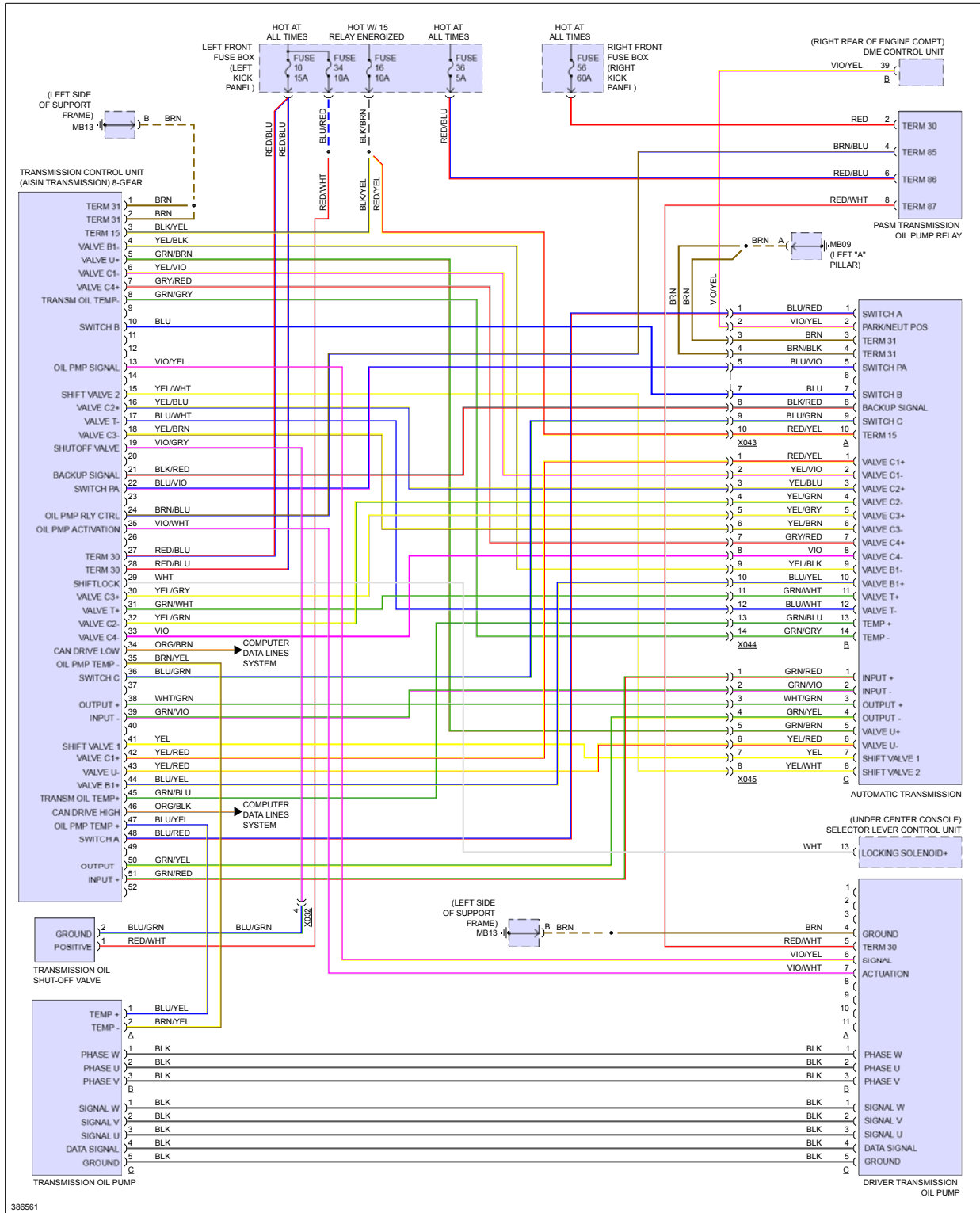
Fig 2: A/T Circuit, Hybrid
