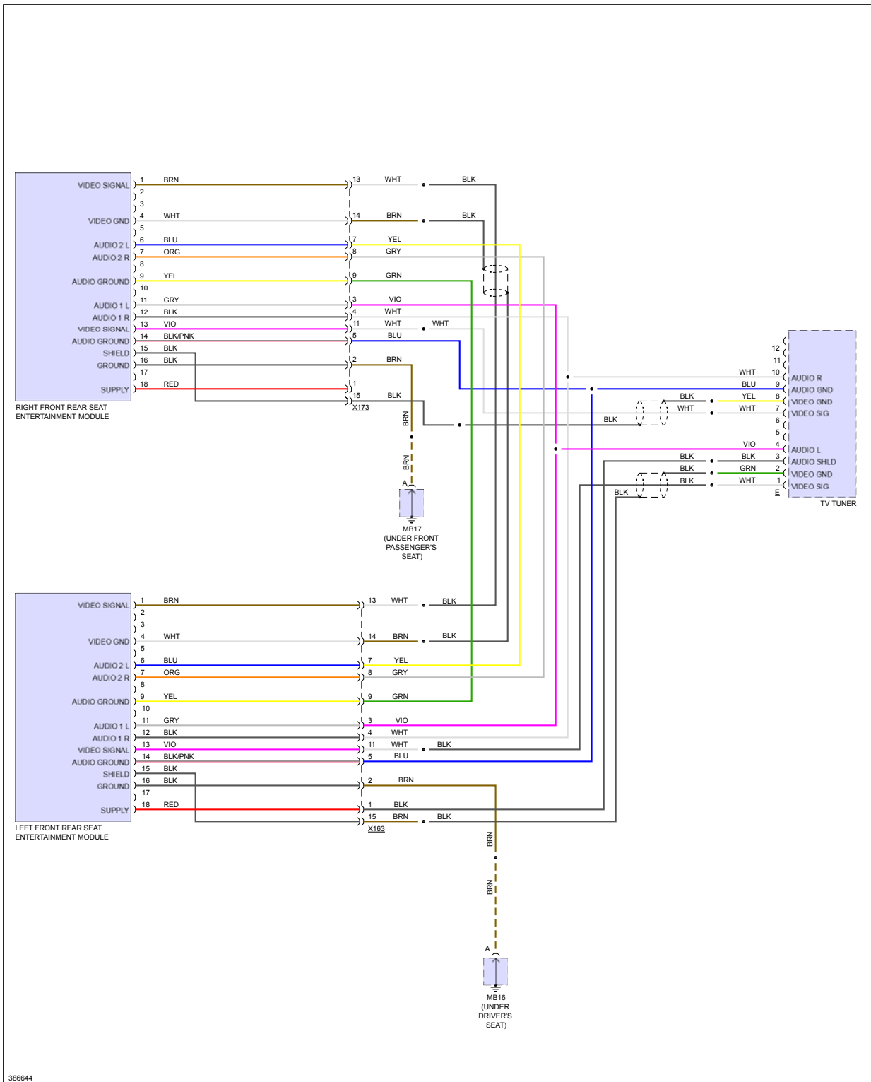
Fig 12: Rear Seat Entertainment Circuit
