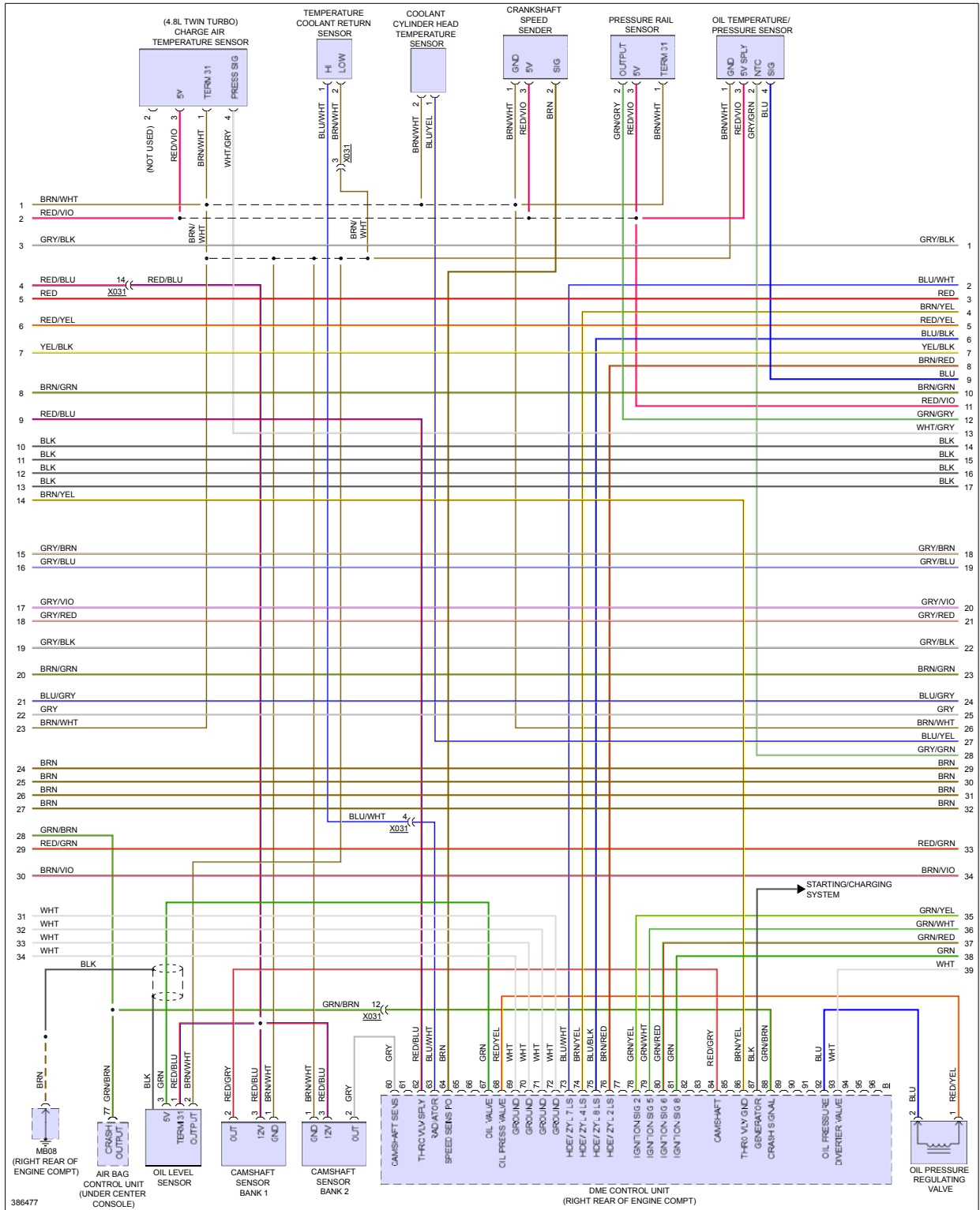
Fig 4: 4.8L Twin Turbo, Engine Performance Circuit (4 of 5)
