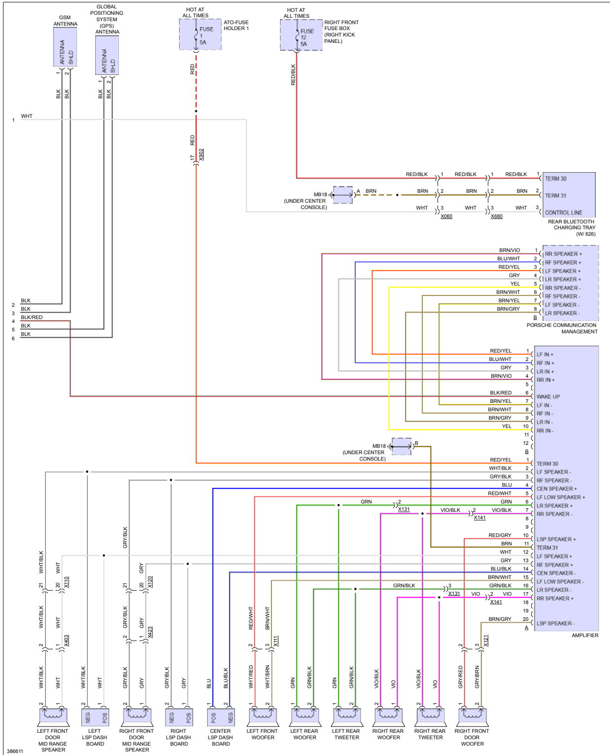
Fig 3: Navigation Circuit, W/ ASK (2 of 2)
