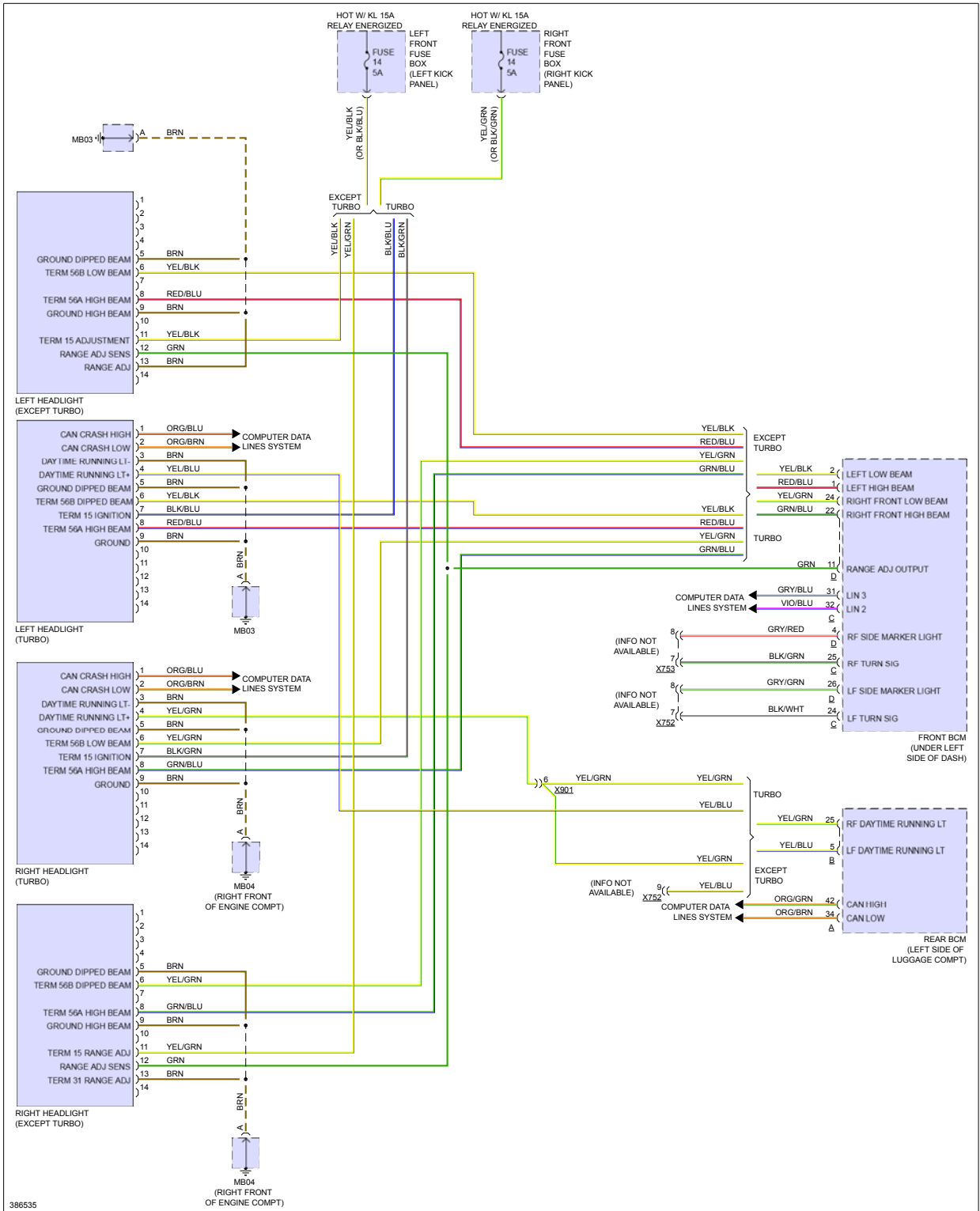
Fig 2: Headlights Circuit, W/O Cornering Headlights
