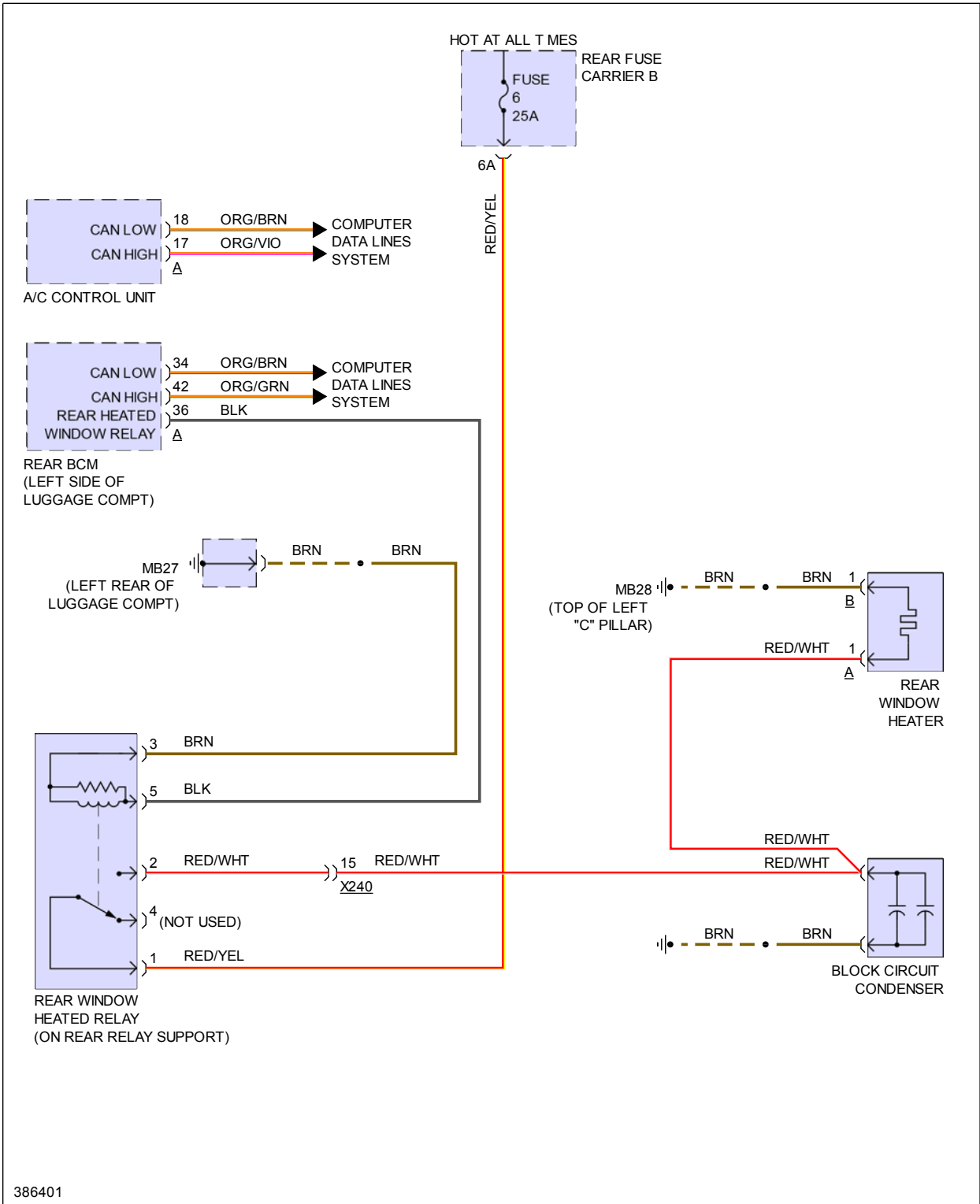
Fig 1: Defogger Circuit
