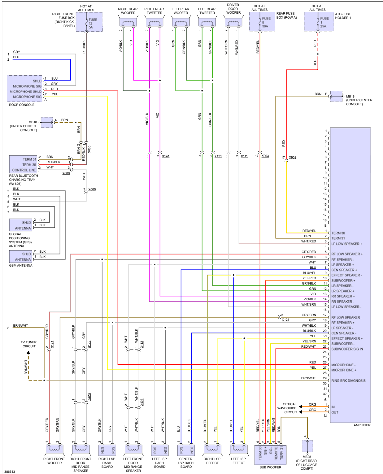
Fig 5: Navigation Circuit, W/ Bose (2 of 2)
