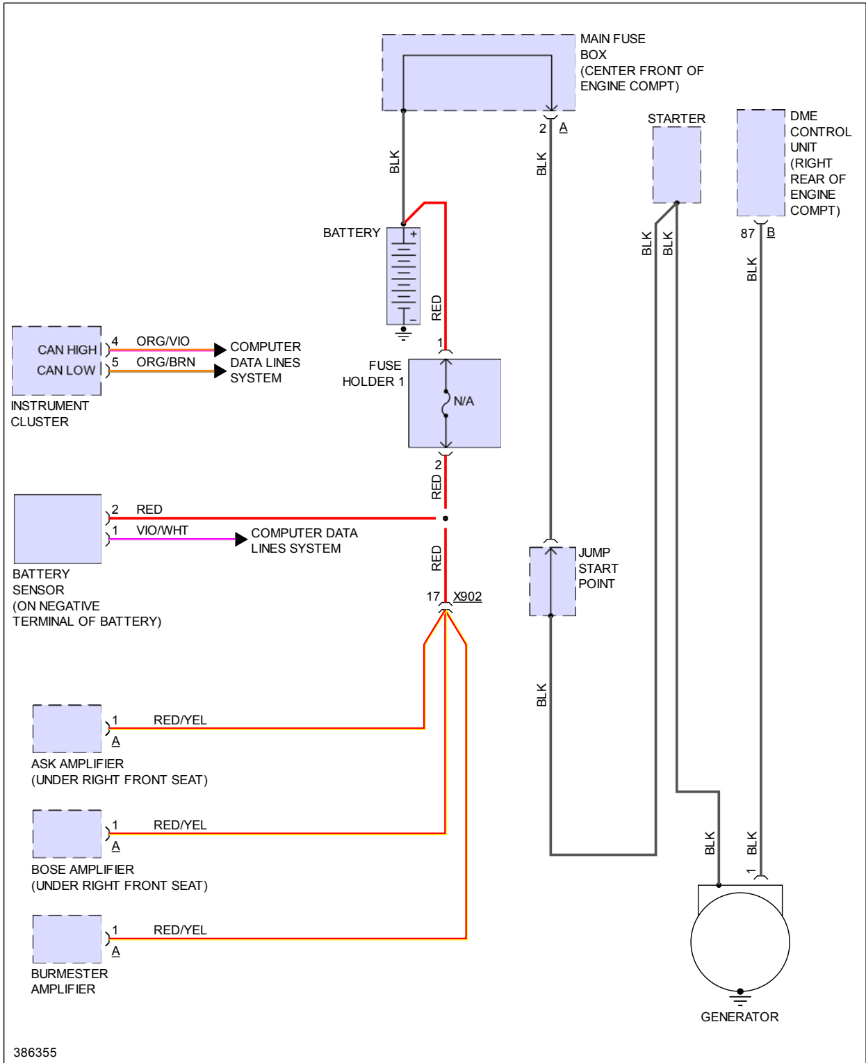
Fig 1: Charging Circuit
