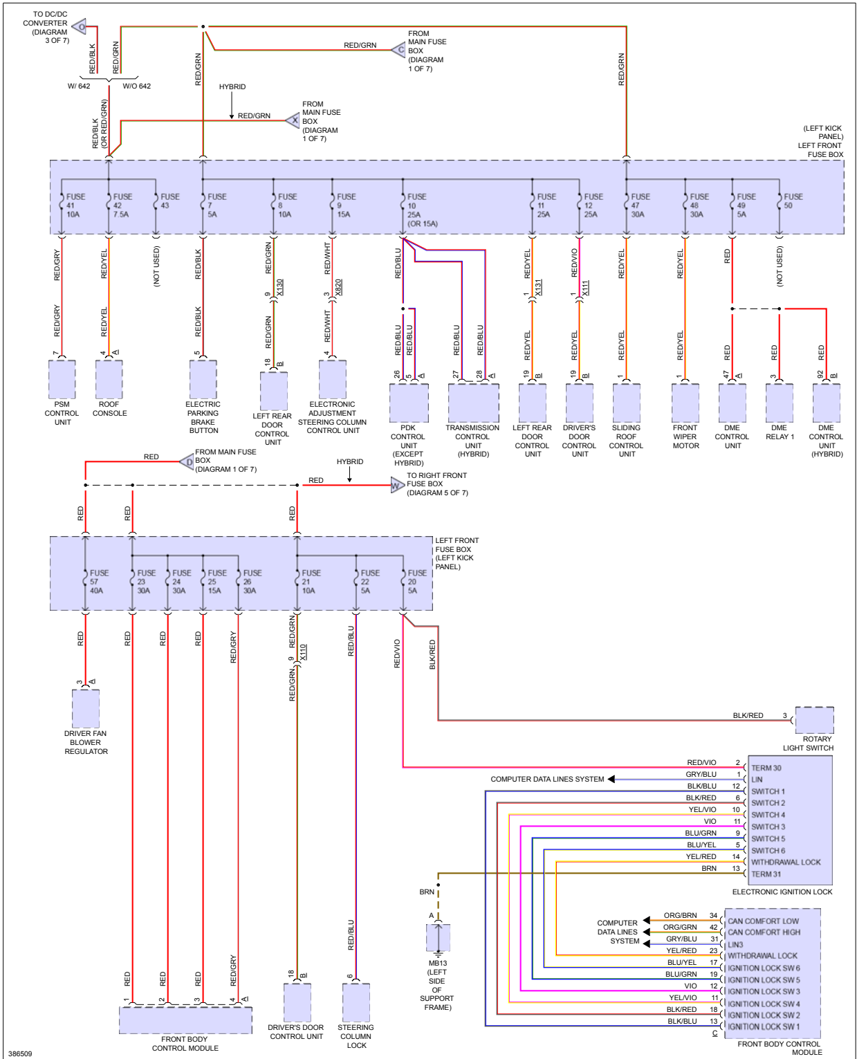
Fig 2: Power Distribution Circuit (2 of 7)
