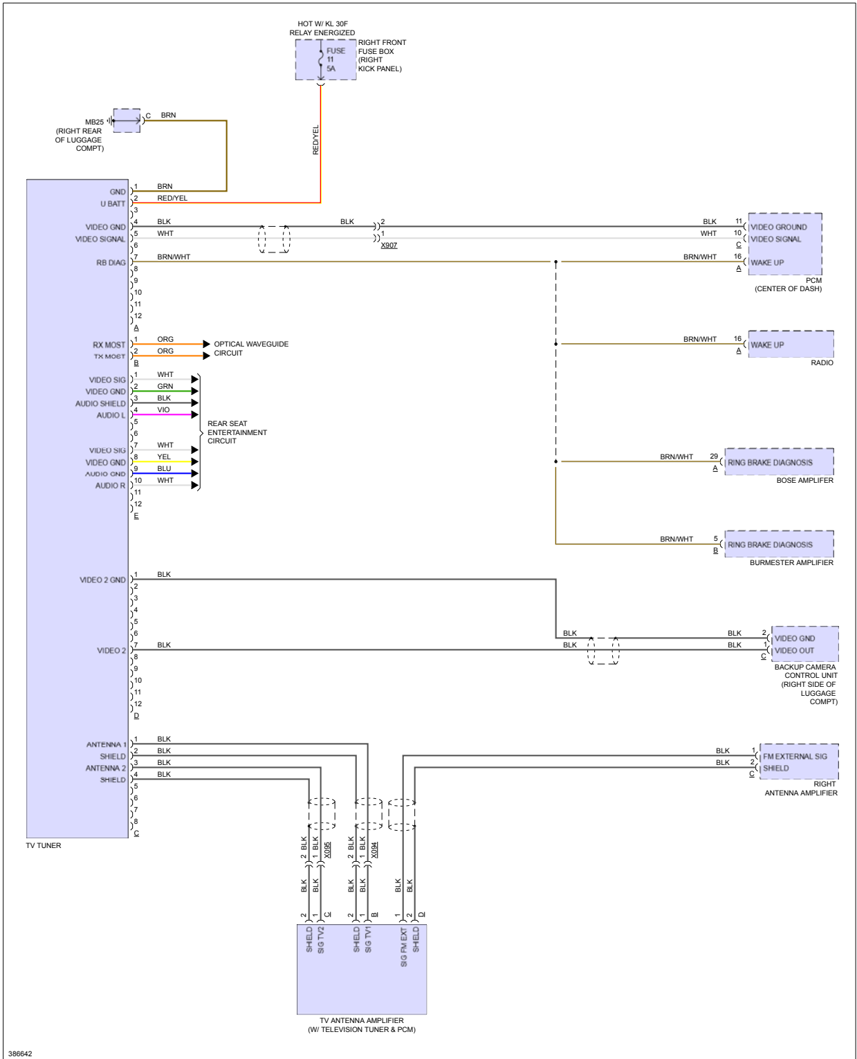
Fig 13: TV Tuner Circuit
