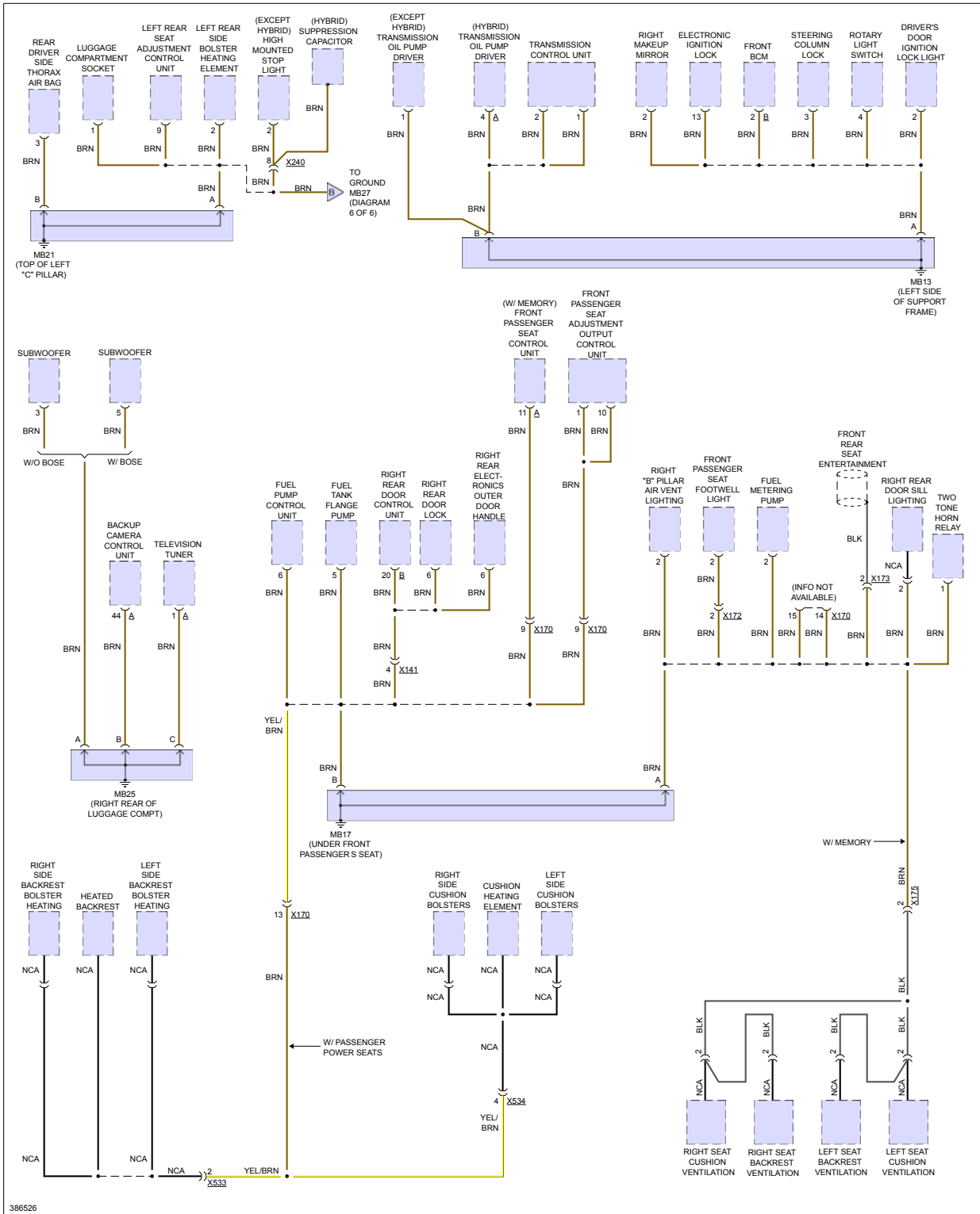
Fig 3: Ground Distribution Circuit (3 of 6)
