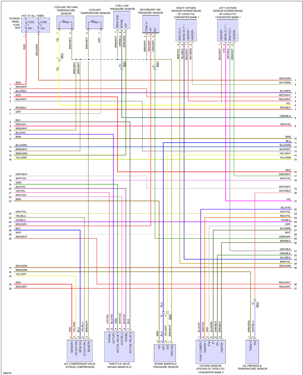
Fig 4: 3.0L Hybrid, Engine Performance Circuit (4 of 7)
