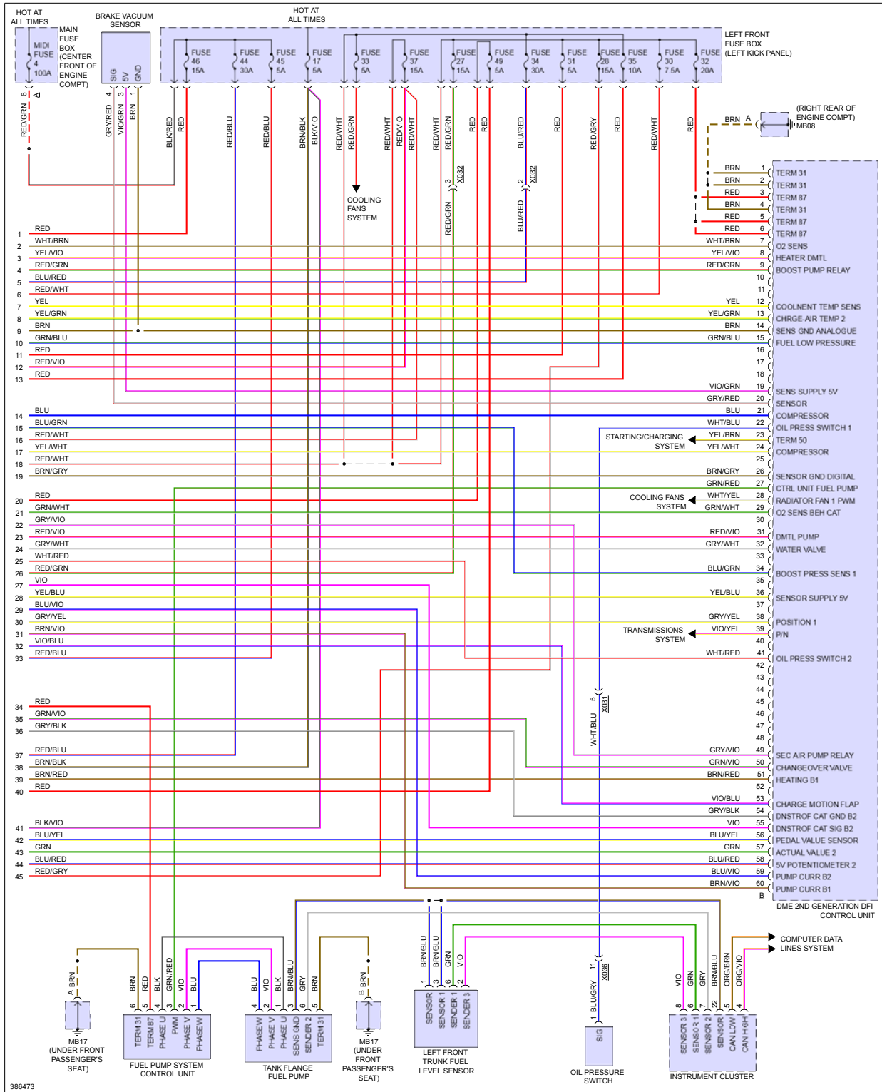
Fig 7: 3.0L Hybrid, Engine Performance Circuit (7 of 7)
