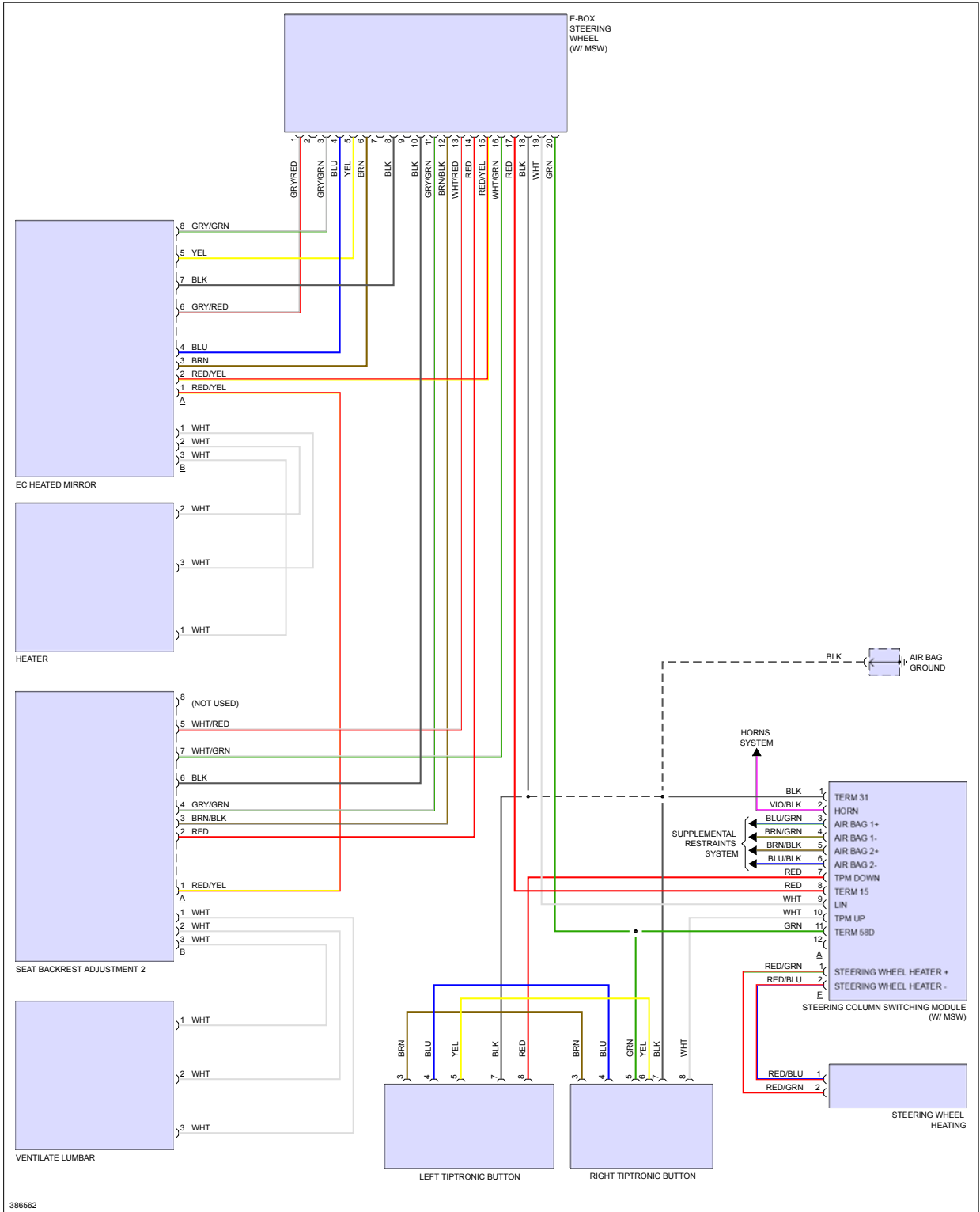
Fig 1: A/T Circuit, Except Hybrid
