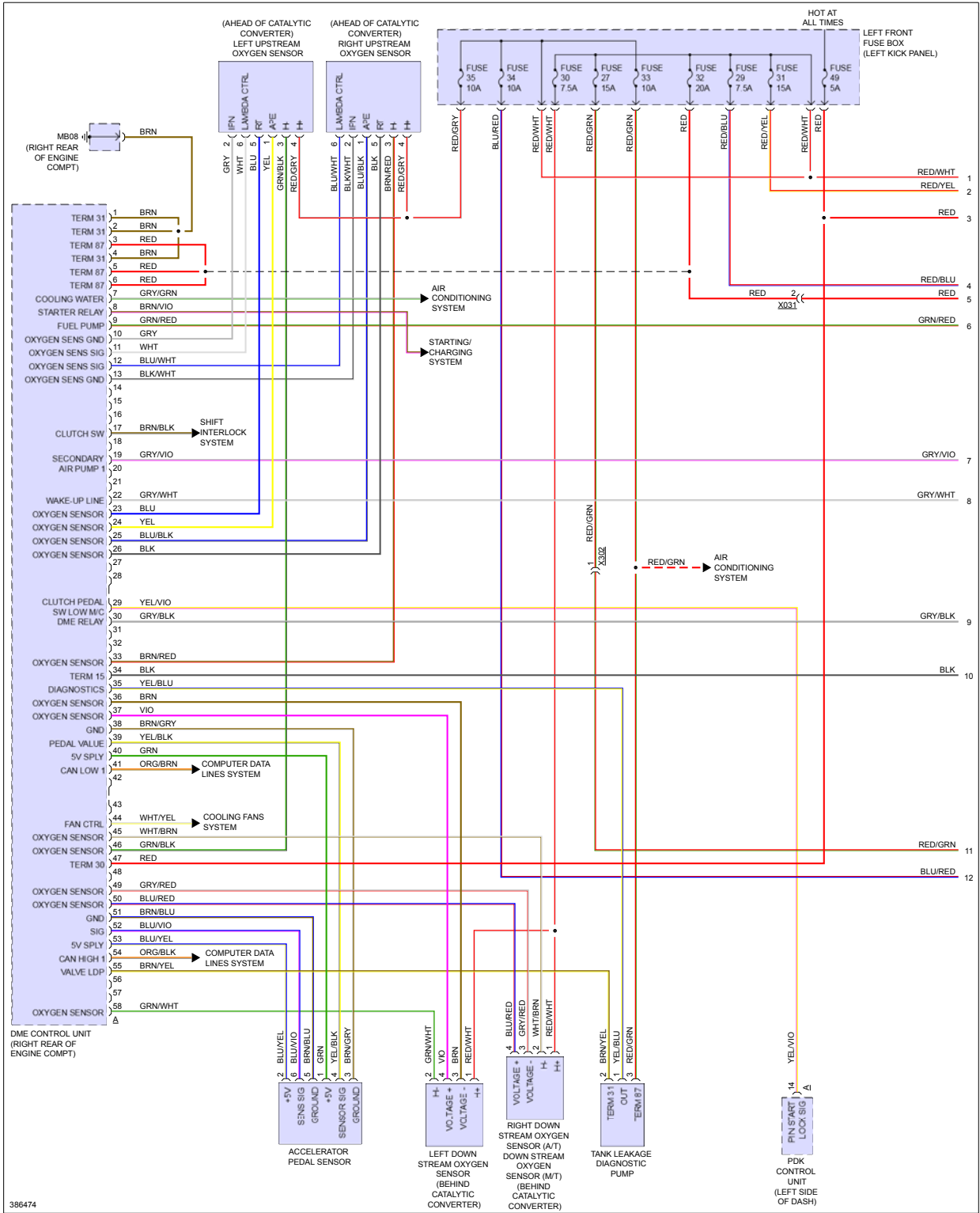
Fig 1: 4.8L, Engine Performance Circuit (1 of 5)
