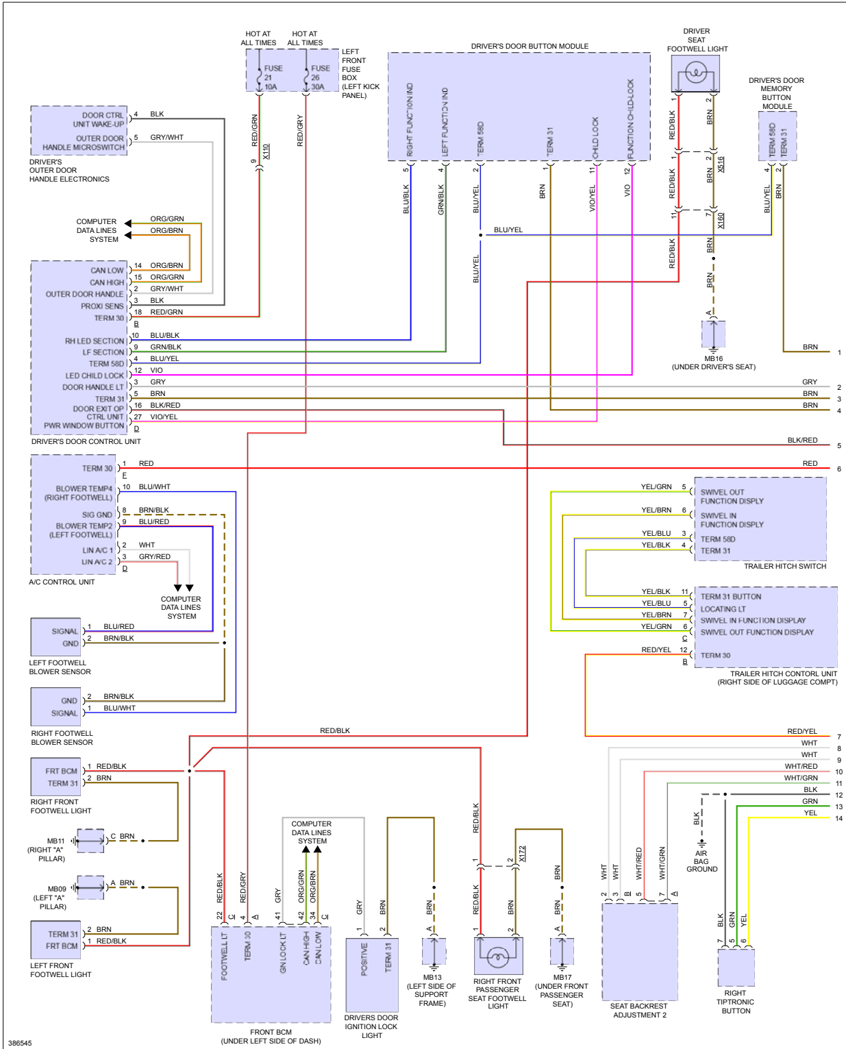
Fig 1: Interior Lights Circuit (1 of 5)
