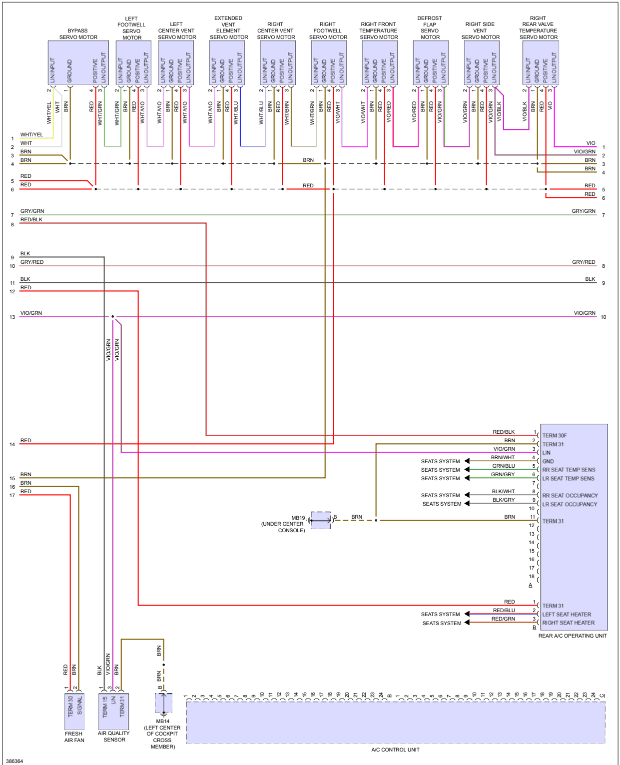
Fig 7: Automatic A/C Circuit, Hybrid (3 of 4)
