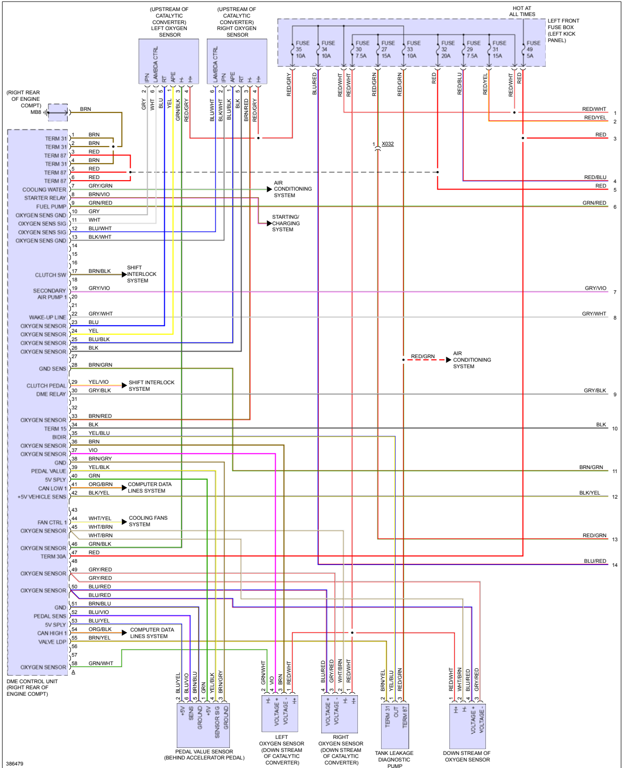
Fig 1: 3.6L, Engine Performance Circuit (1 of 5)
