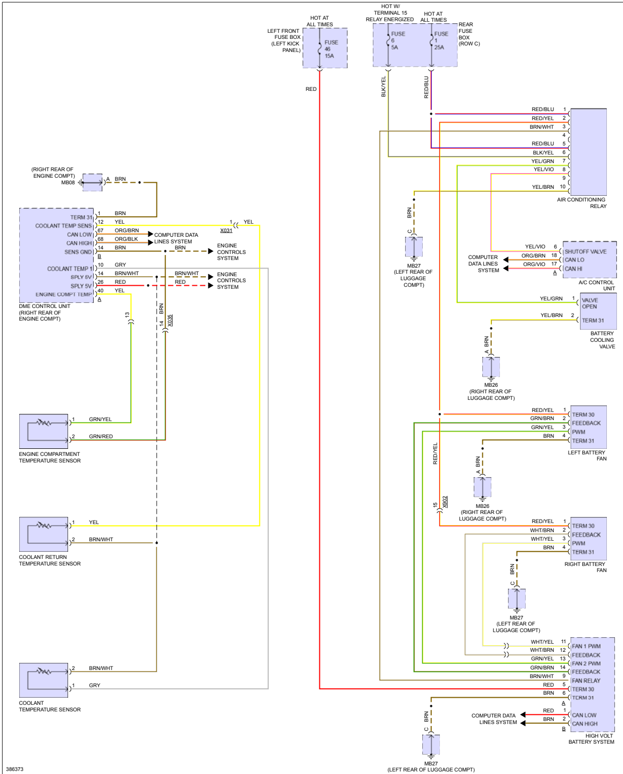
Fig 2: Cooling Fan Circuit, Hybrid
