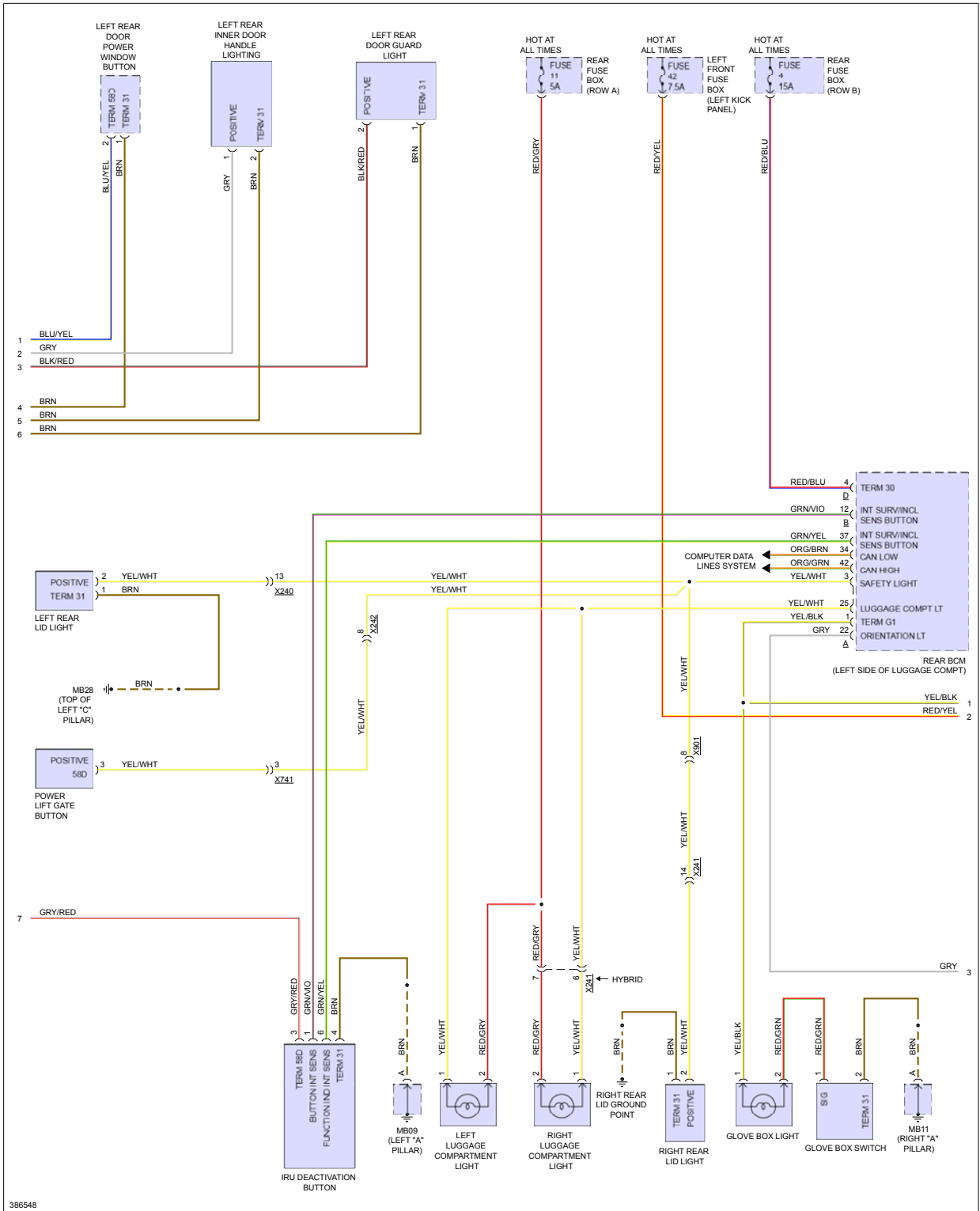
Fig 4: Interior Lights Circuit (4 of 5)
