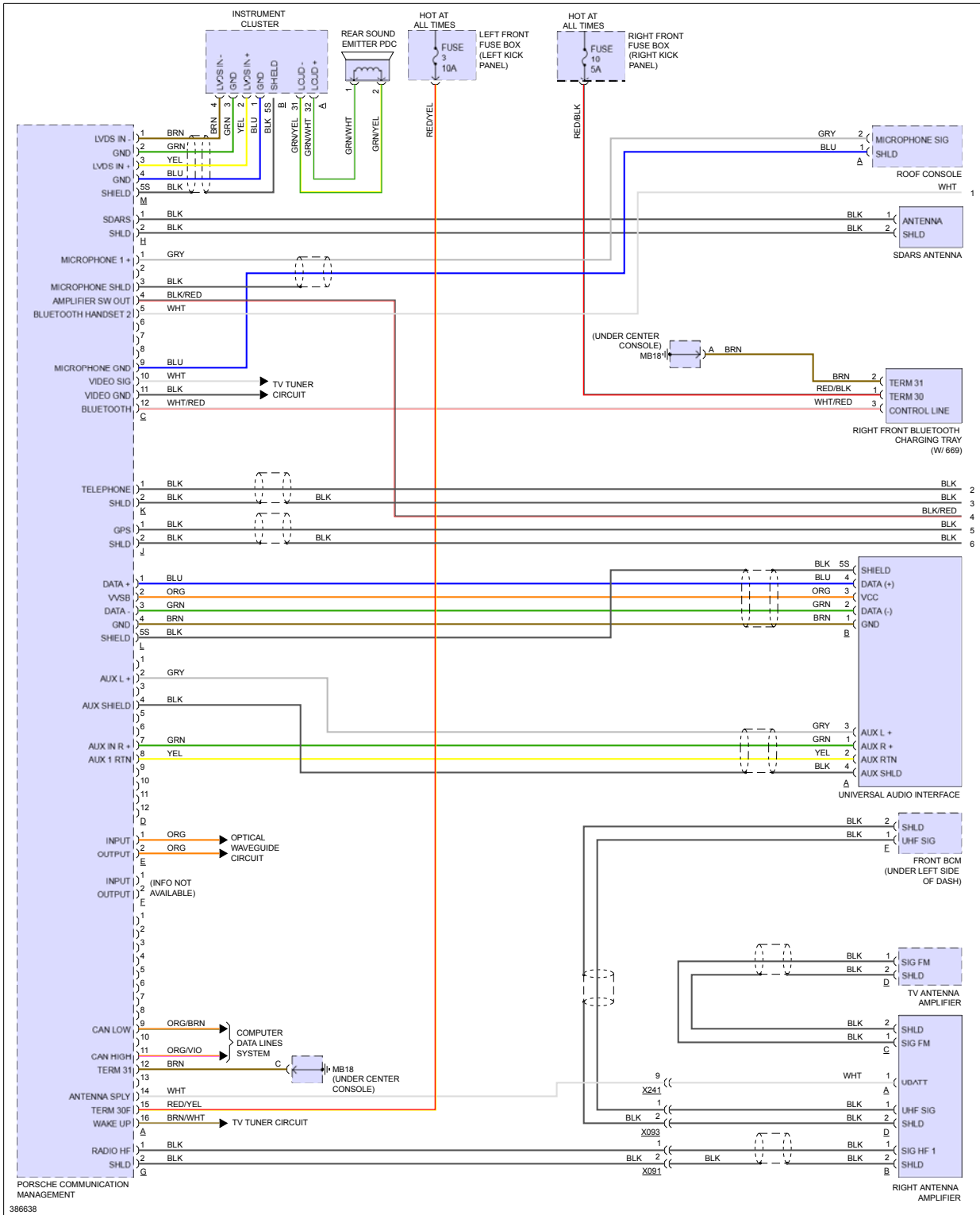
Fig 5: Premium Radio Circuit, W/ ASK (1 of 2)
