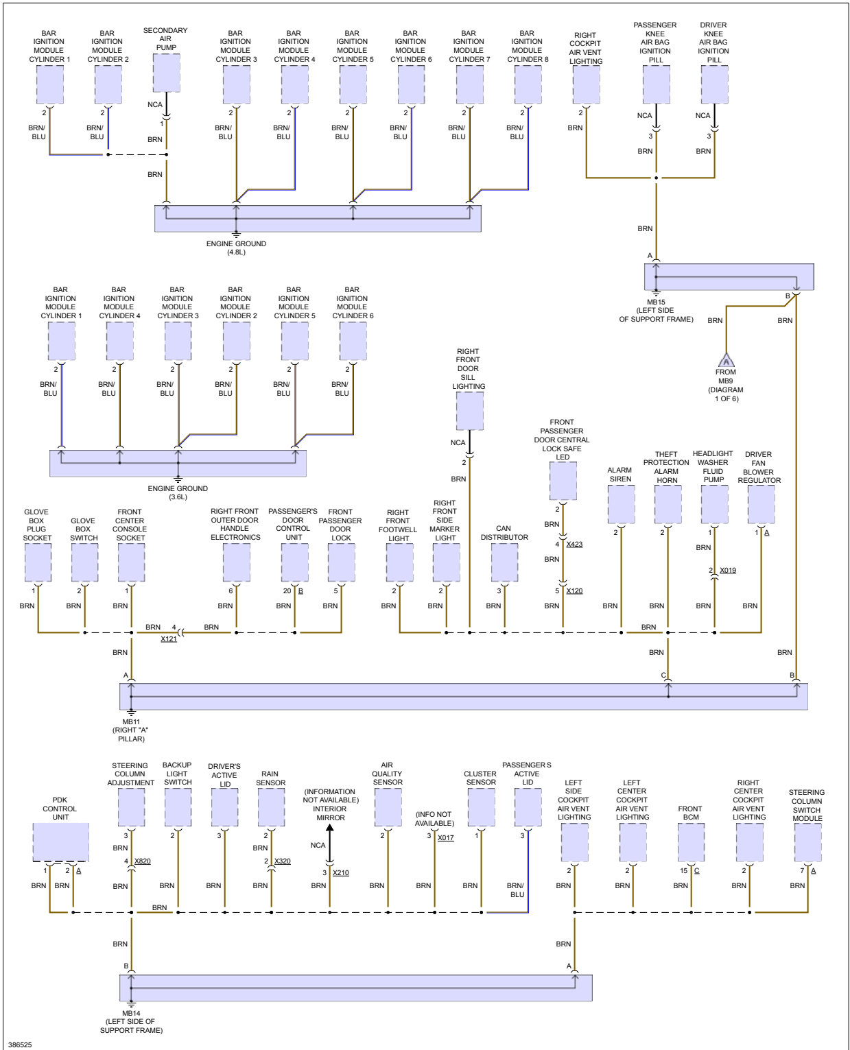
Fig 2: Ground Distribution Circuit (2 of 6)
