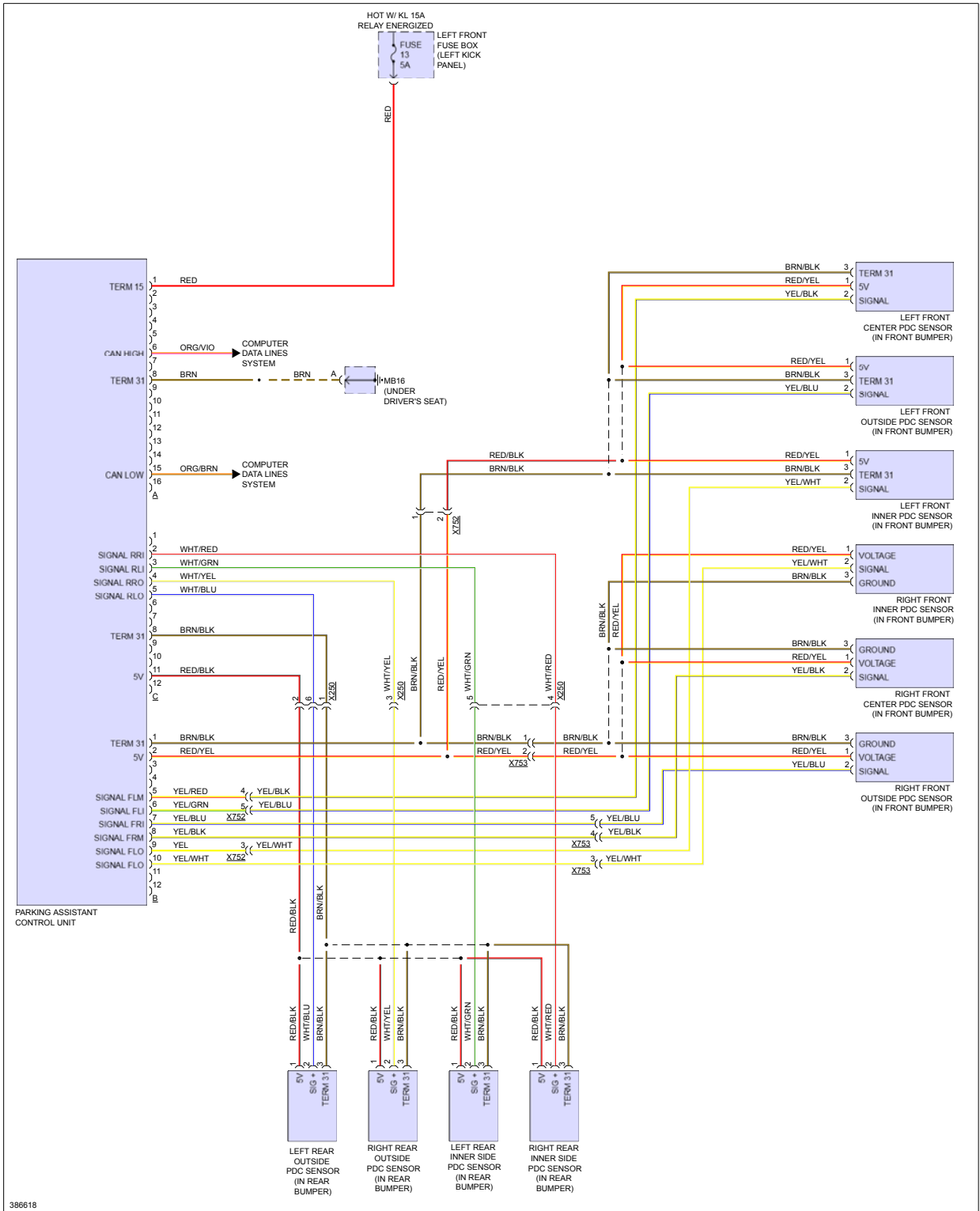
Fig 9: Parking Assistant Circuit
