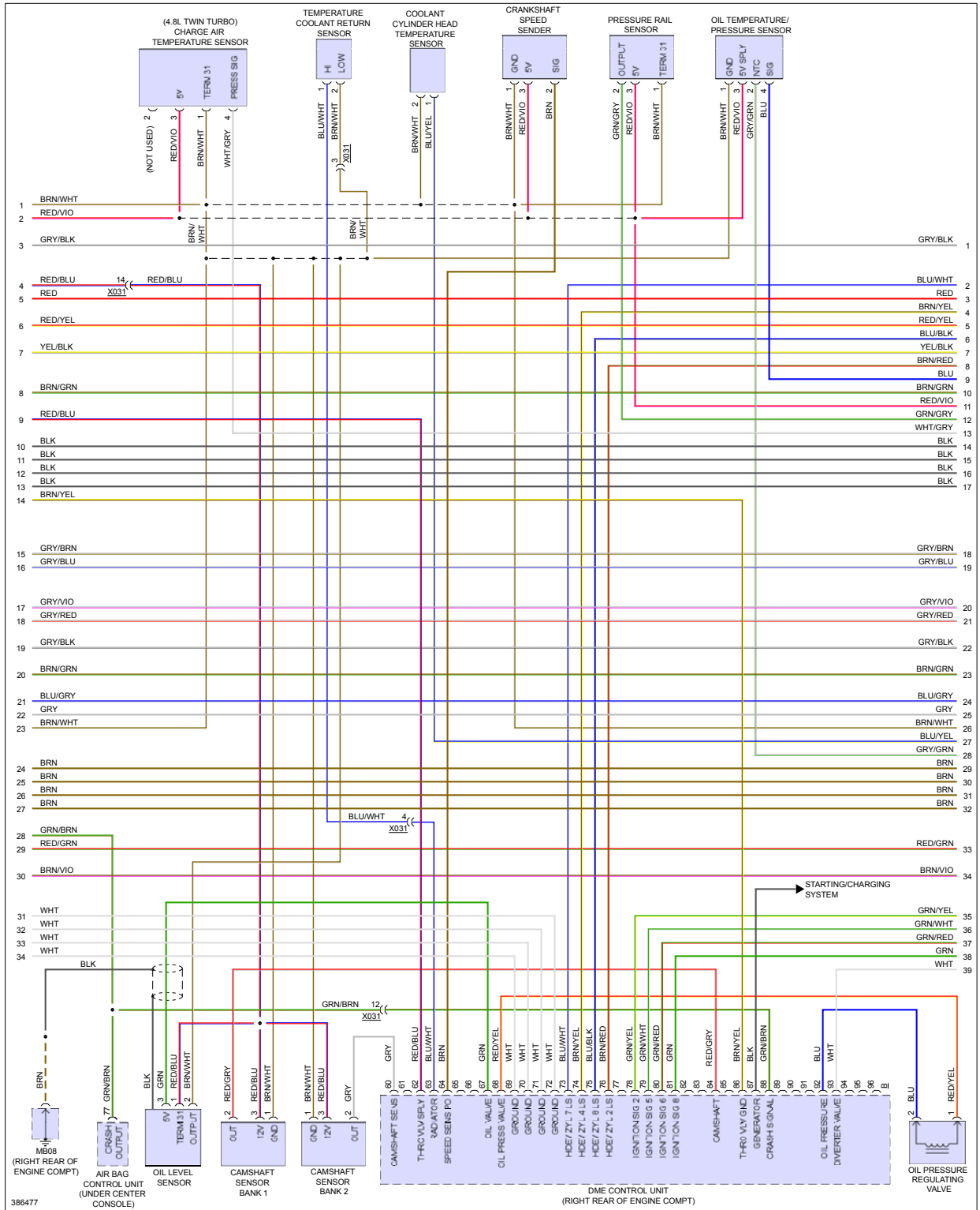
Fig 4: 4.8L, Engine Performance Circuit (4 of 5)
