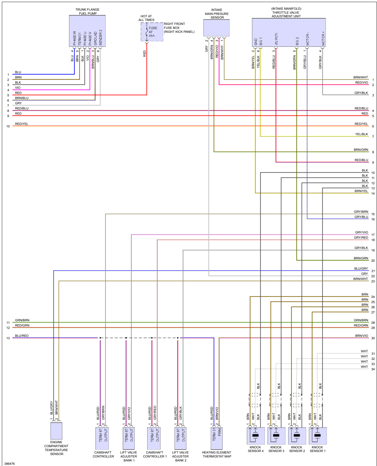
Fig 3: 4.8L, Engine Performance Circuit (3 of 5)
