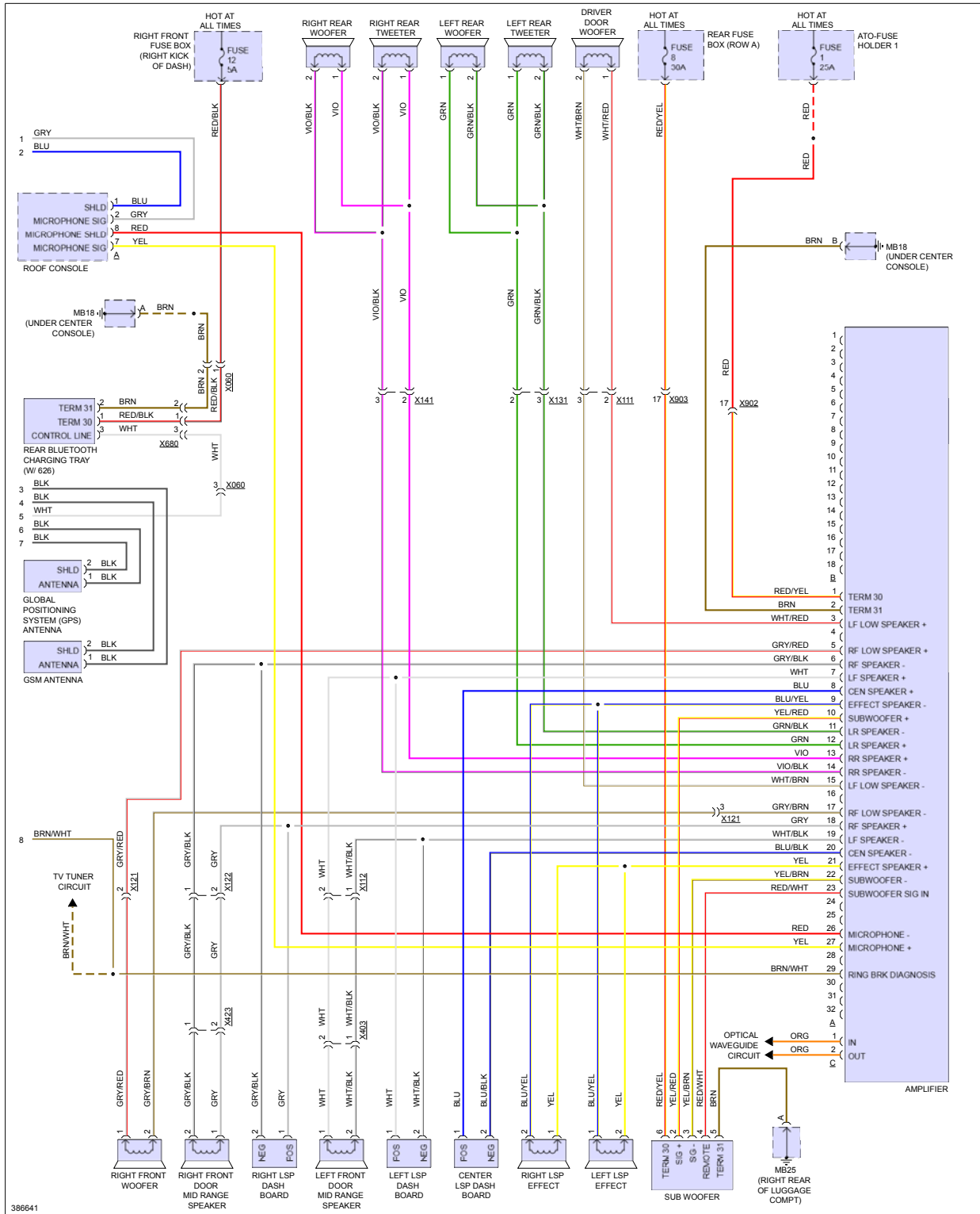
Fig 8: Premium Radio Circuit, W/ Bose (2 of 2)
