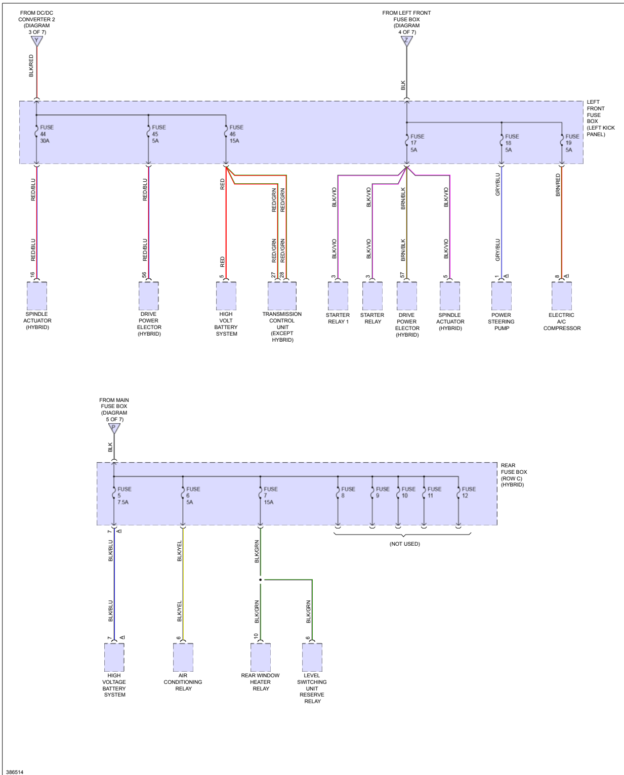
Fig 7: Power Distribution Circuit (7 of 7)
