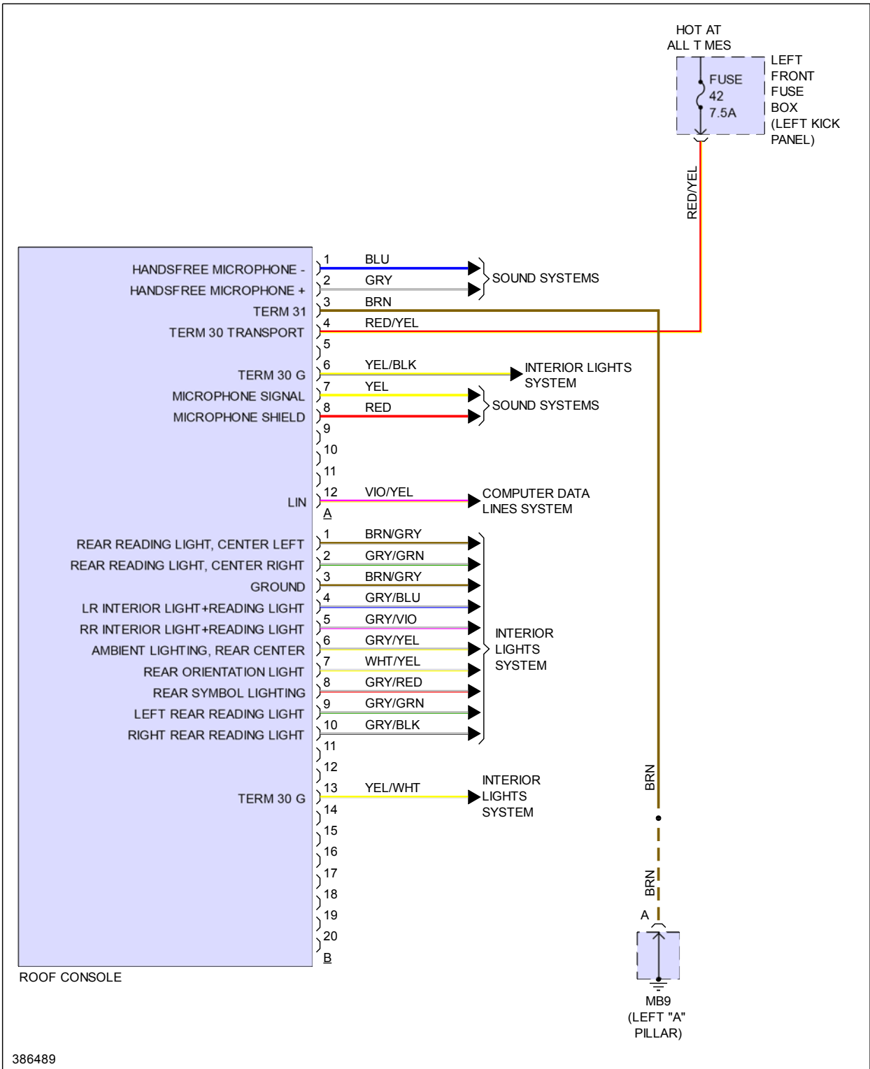
Fig 2: Overhead Console Circuit
