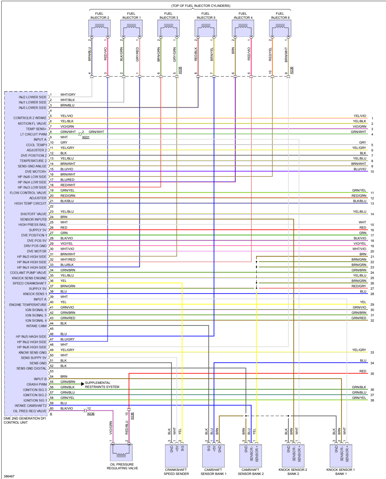
Fig 1: 3.0L Hybrid, Engine Performance Circuit (1 of 7)
