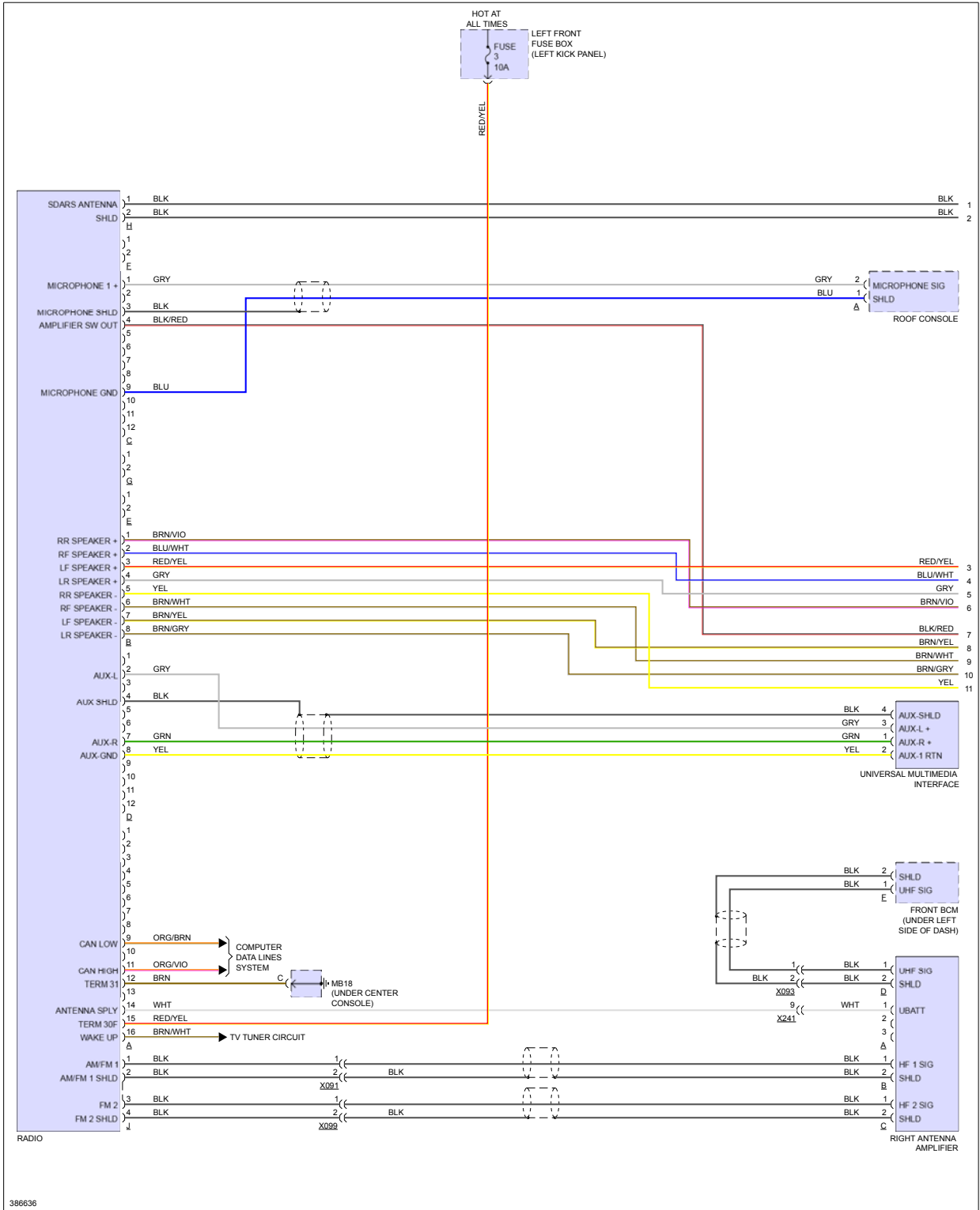
Fig 1: Base Radio Circuit, W/ Amplifier (1 of 2)
