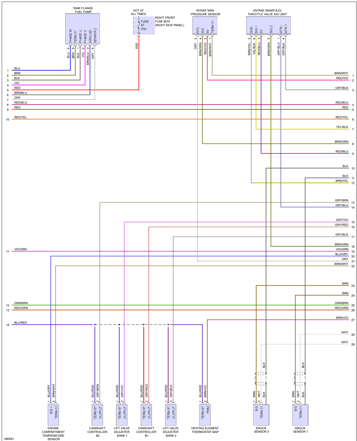
Fig 3: 3.6L, Engine Performance Circuit (3 of 5)
