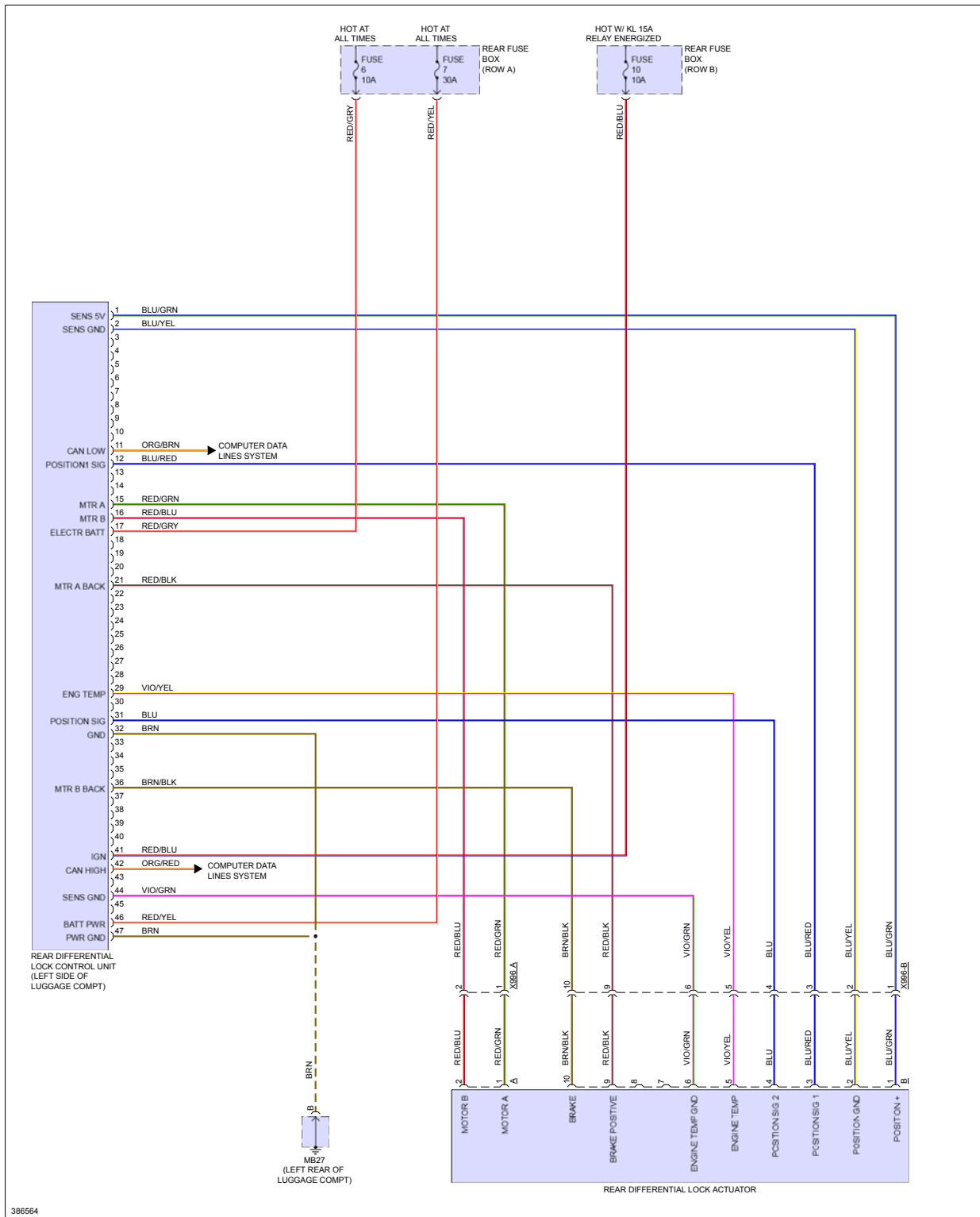
Fig 4: Rear Differential Lock Circuit
