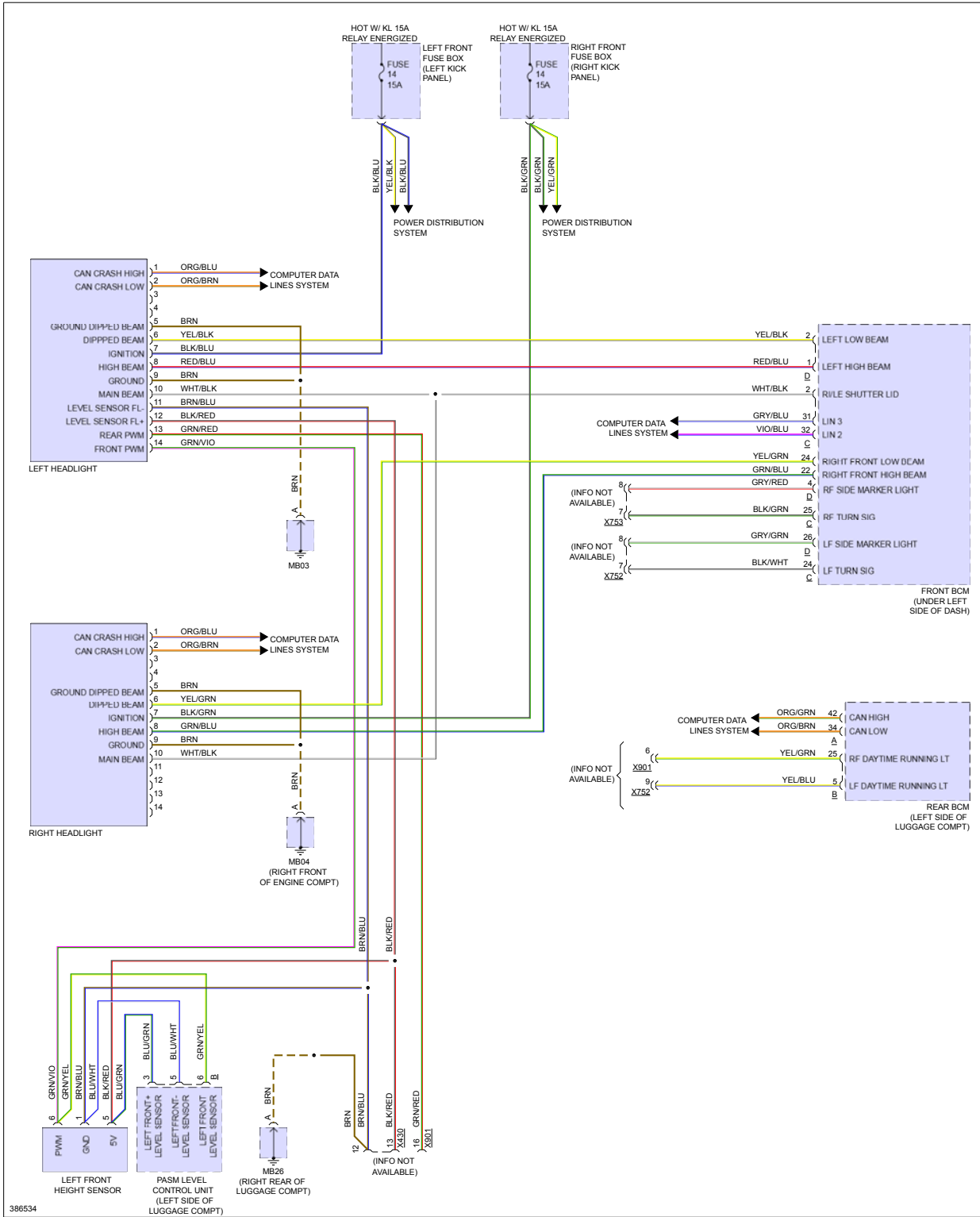
Fig 1: Headlights Circuit, W/ Cornering Headlights
