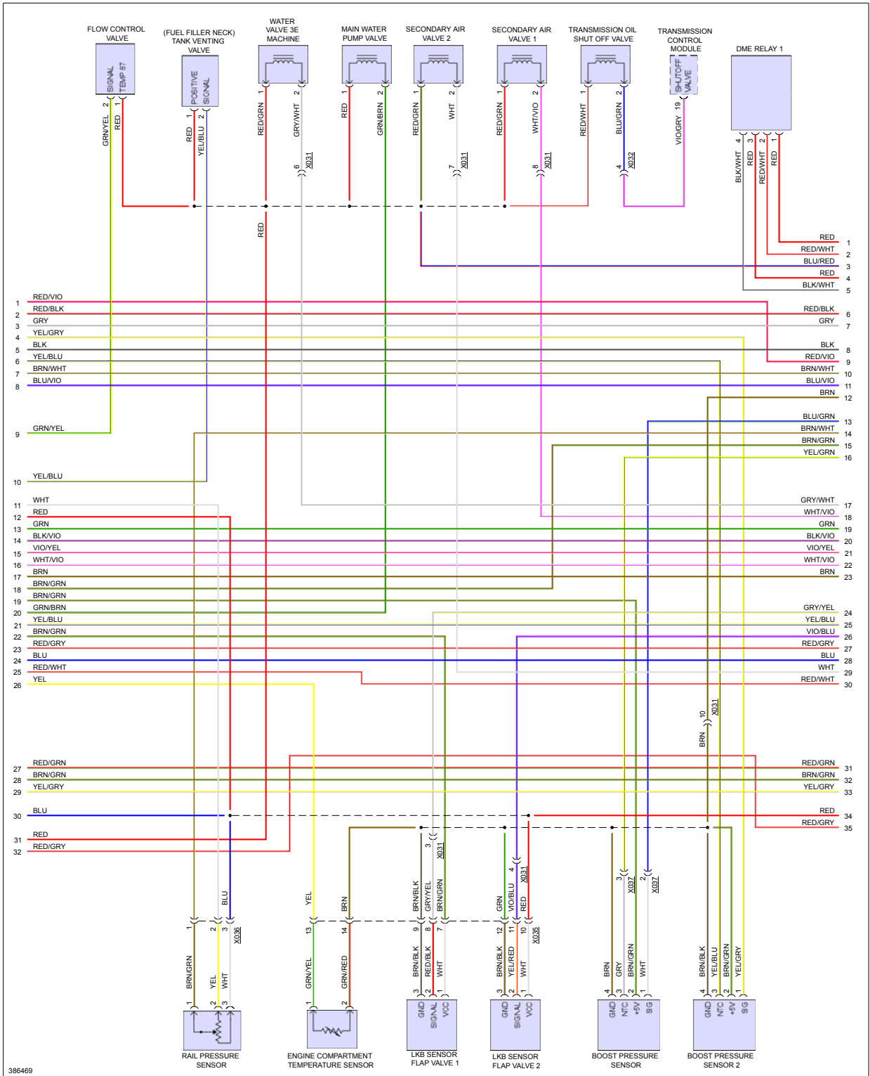
Fig 3: 3.0L Hybrid, Engine Performance Circuit (3 of 7)
