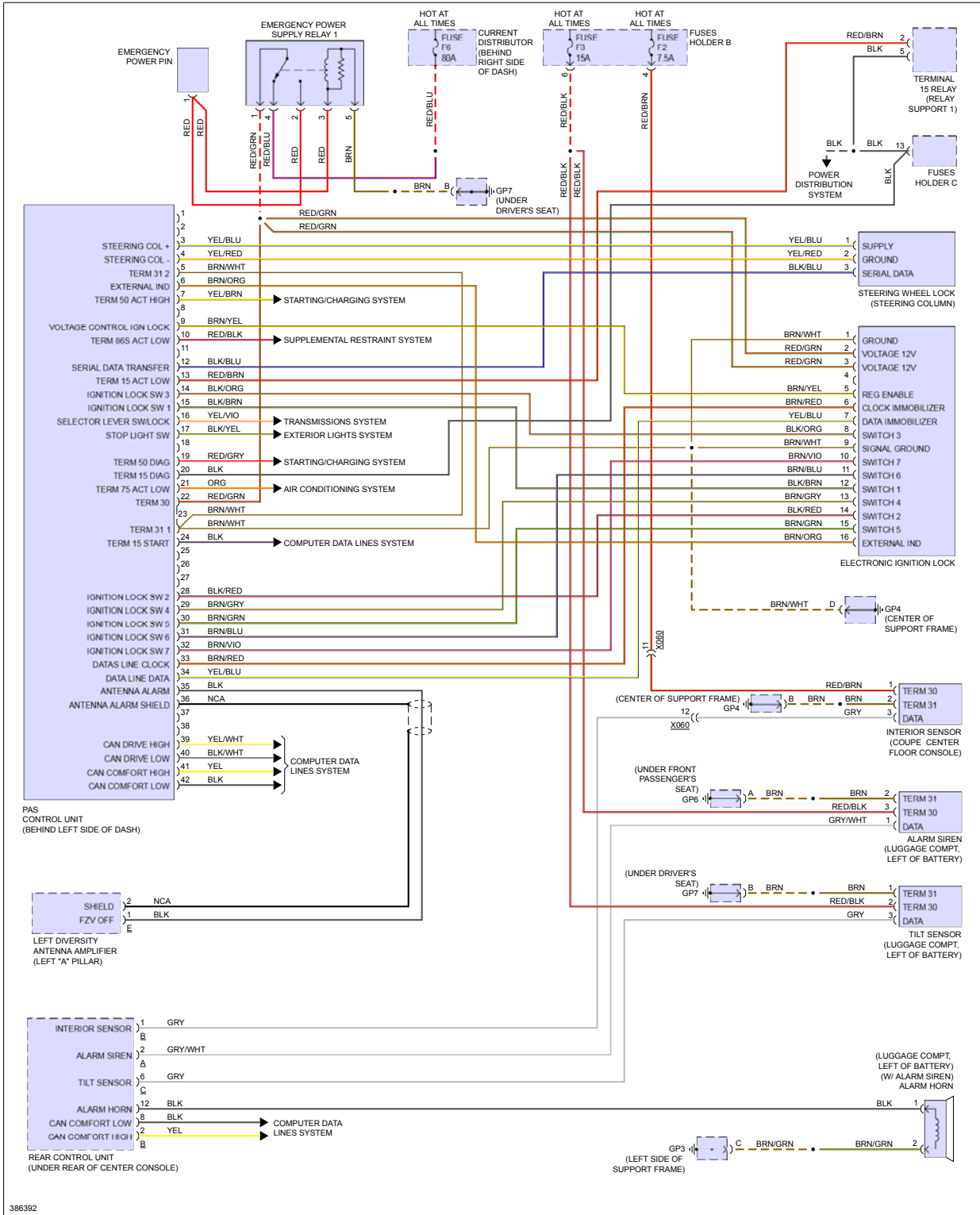
Fig 1: Anti-theft Circuit
