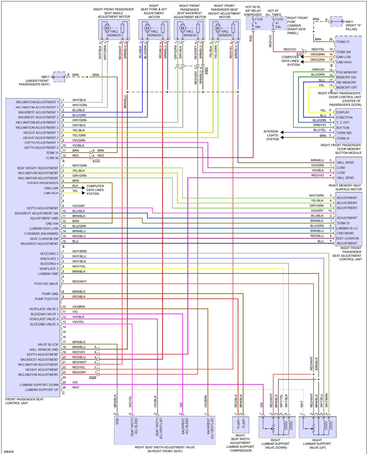
Fig 5: Passenger's Memory Seat Circuit, Sport Comfort
