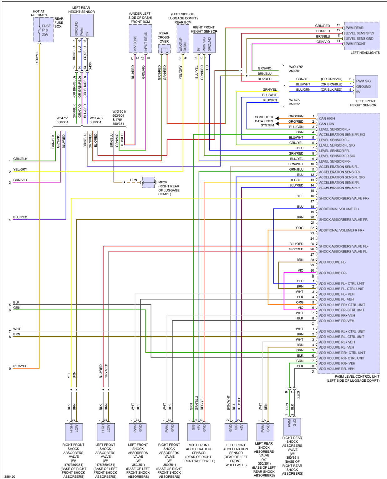
Fig 3: Electronic Level Control Circuit (2 of 2)
