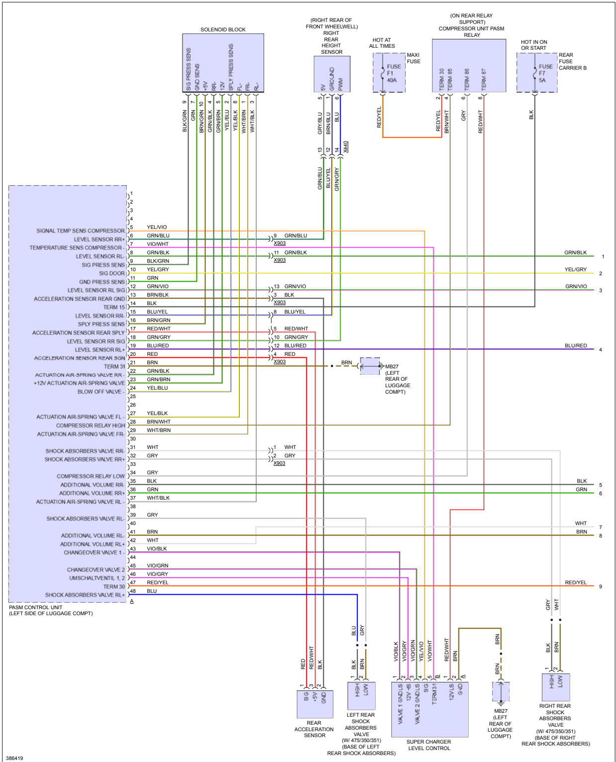
Fig 2: Electronic Level Control Circuit (1 of 2)
