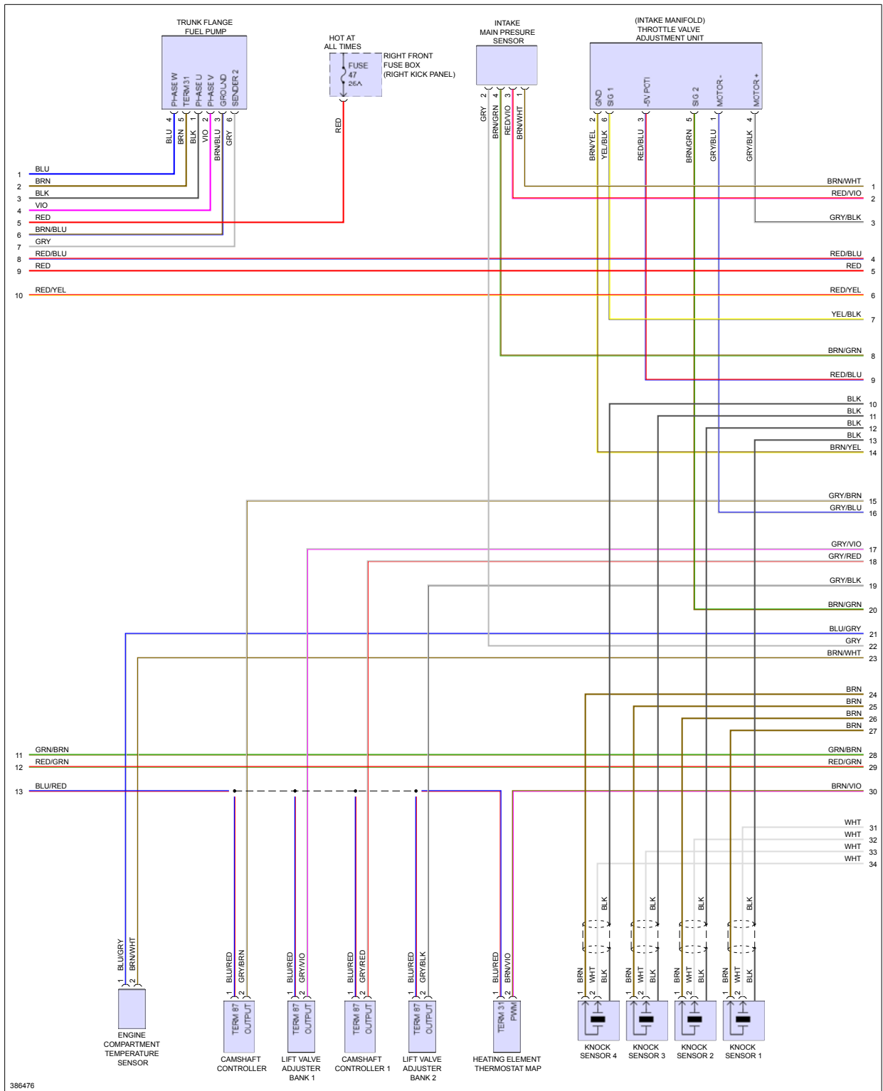
Fig 3: 4.8L Twin Turbo, Engine Performance Circuit (3 of 5)
