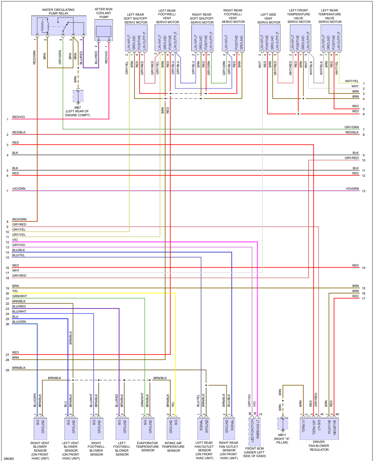
Fig 6: Automatic A/C Circuit, Hybrid (2 of 4)
