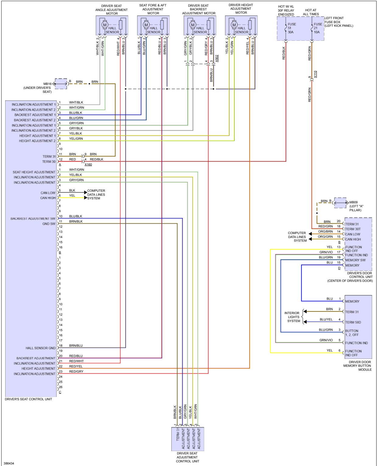
Fig 1: Driver's Memory Seat Circuit, Except Sport Comfort
