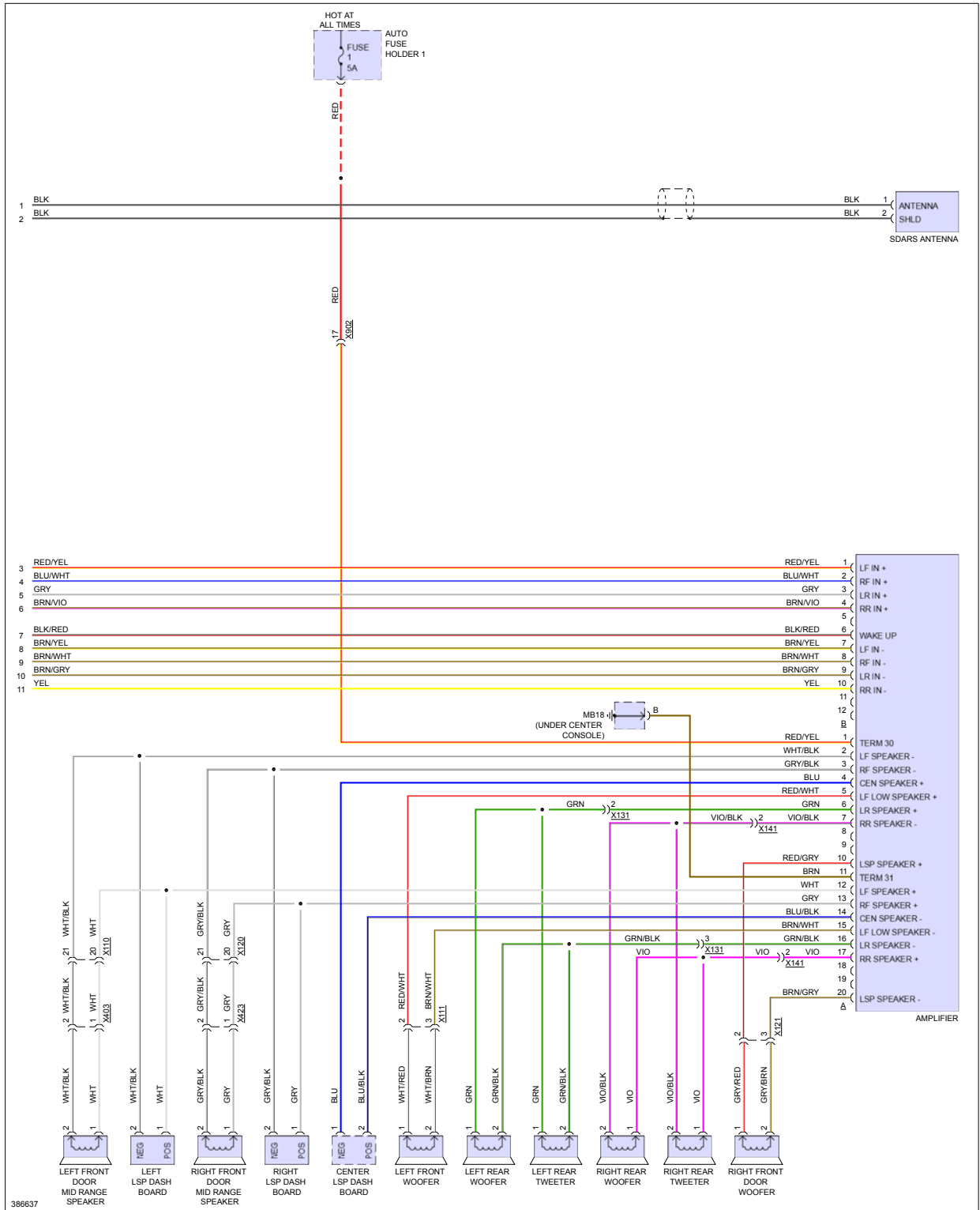
Fig 2: Base Radio Circuit, W/ Amplifier (2 of 2)
