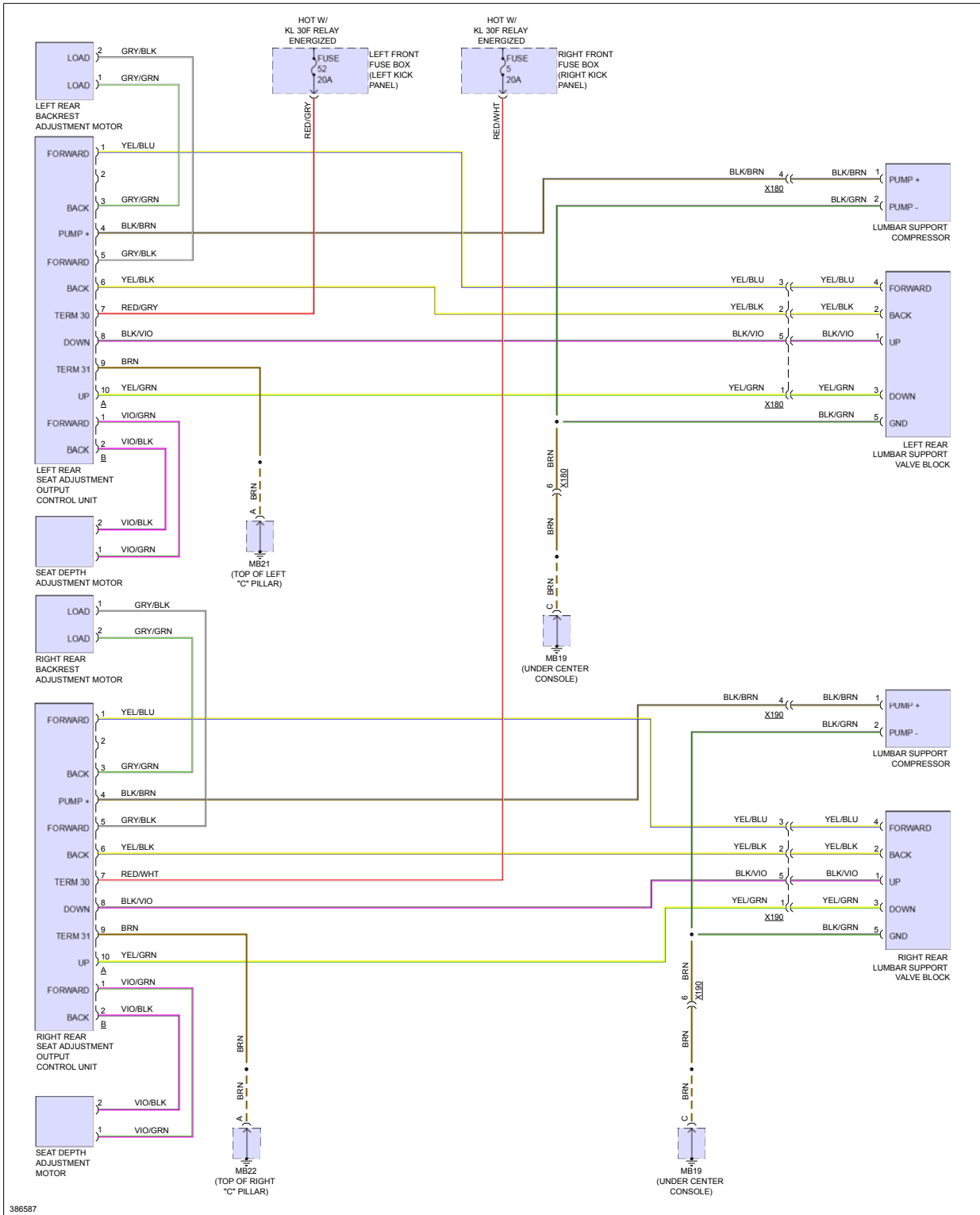
Fig 5: Rear Power Seat Circuit
