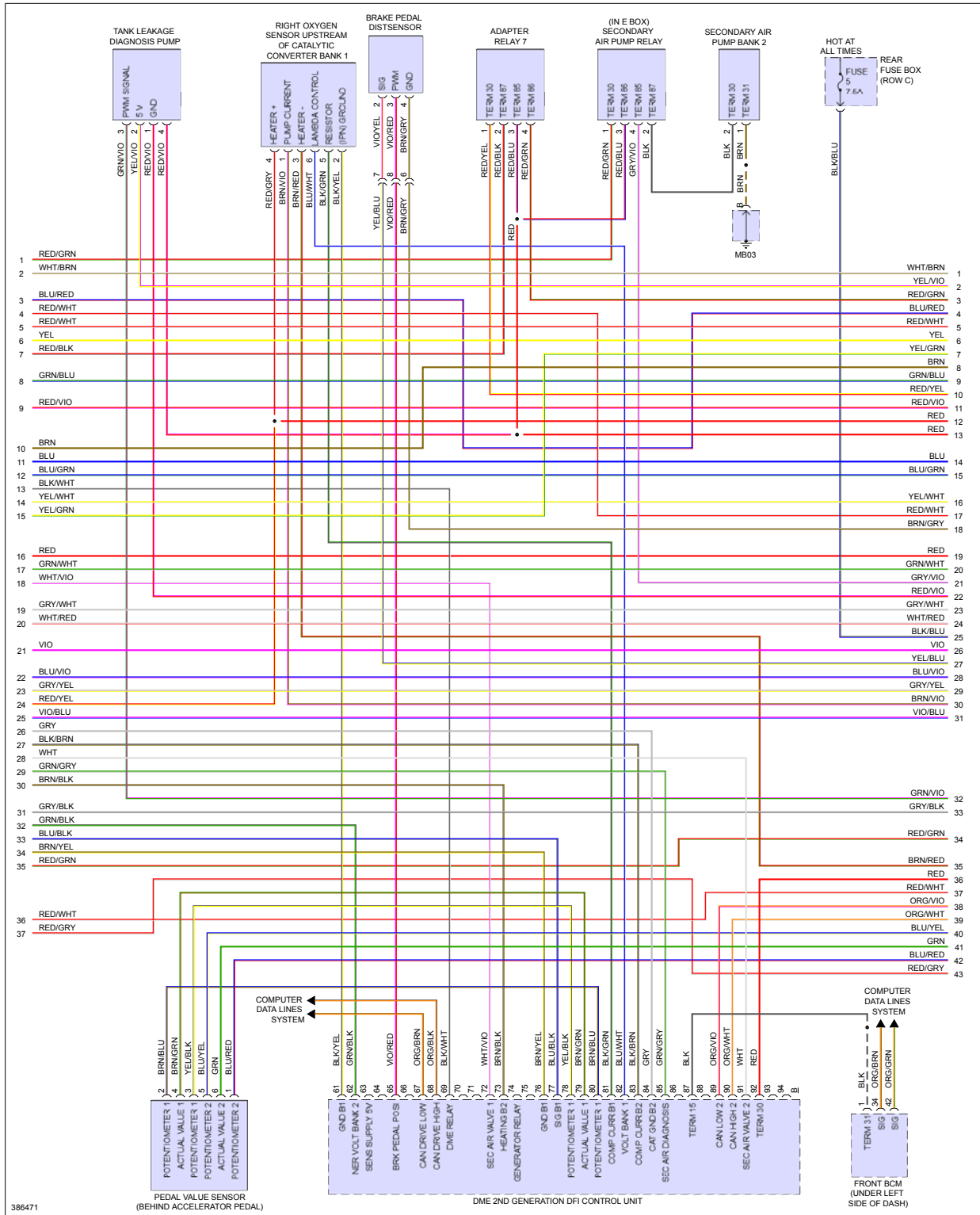
Fig 5: 3.0L Hybrid, Engine Performance Circuit (5 of 7)
