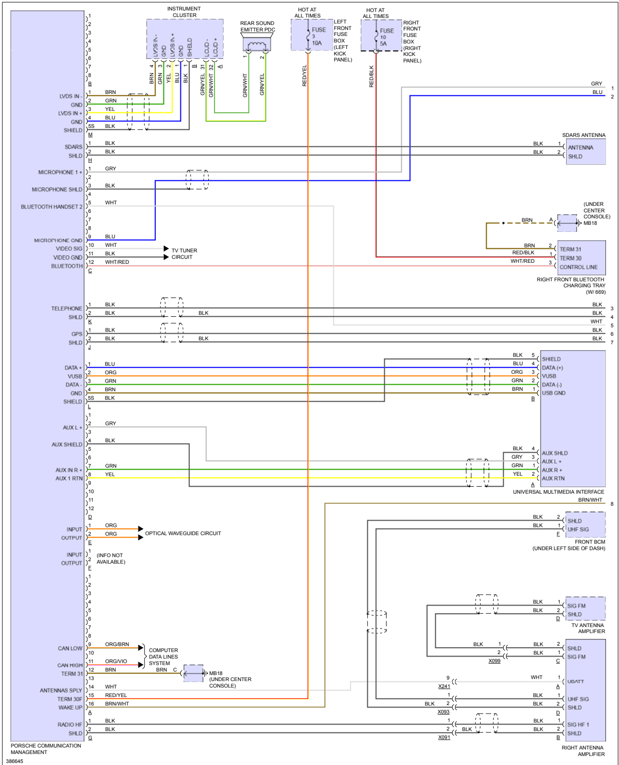
Fig 9: Premium Radio Circuit, W/ Burmester (1 of 3)
