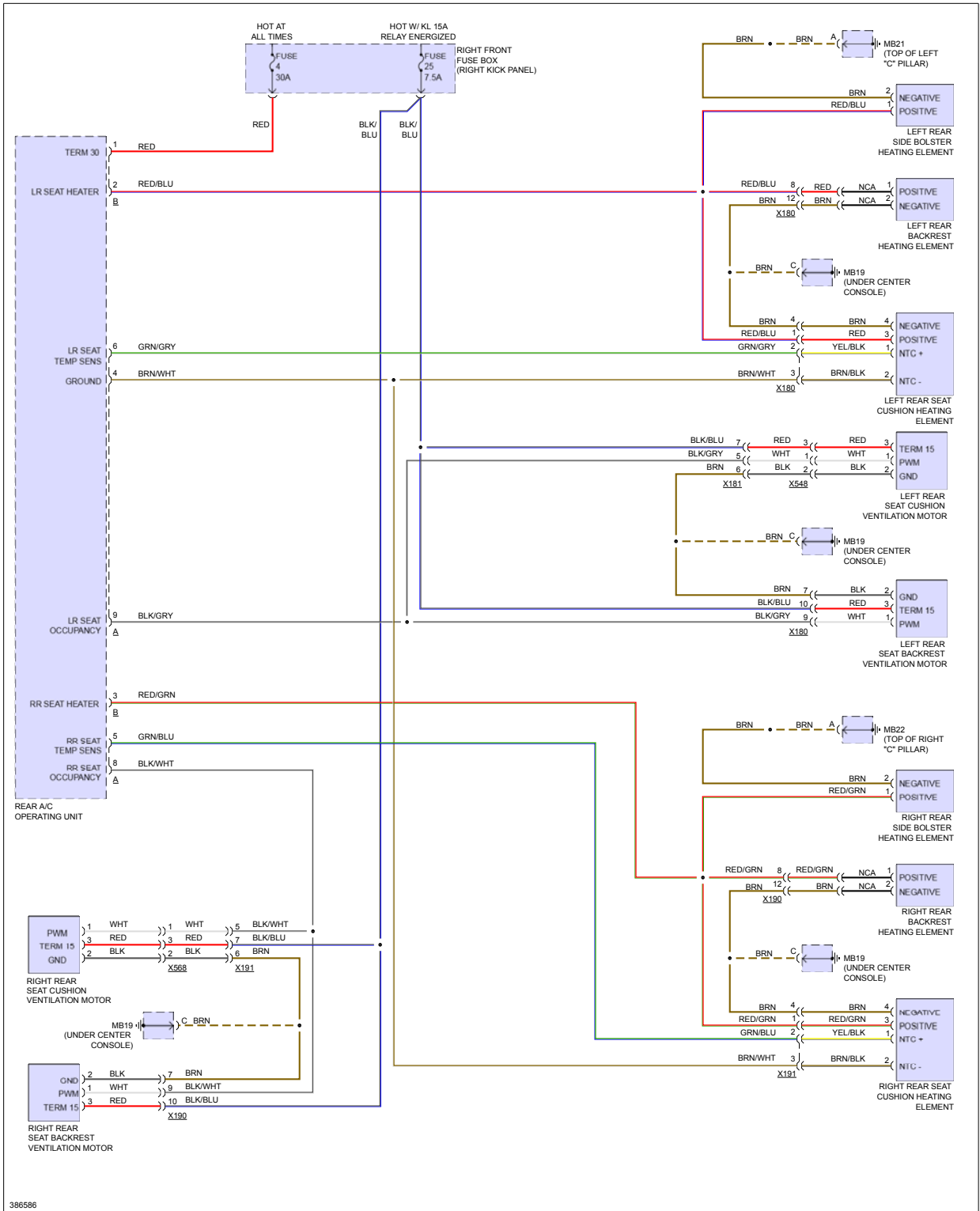
Fig 4: Rear Heated Seats Circuit
