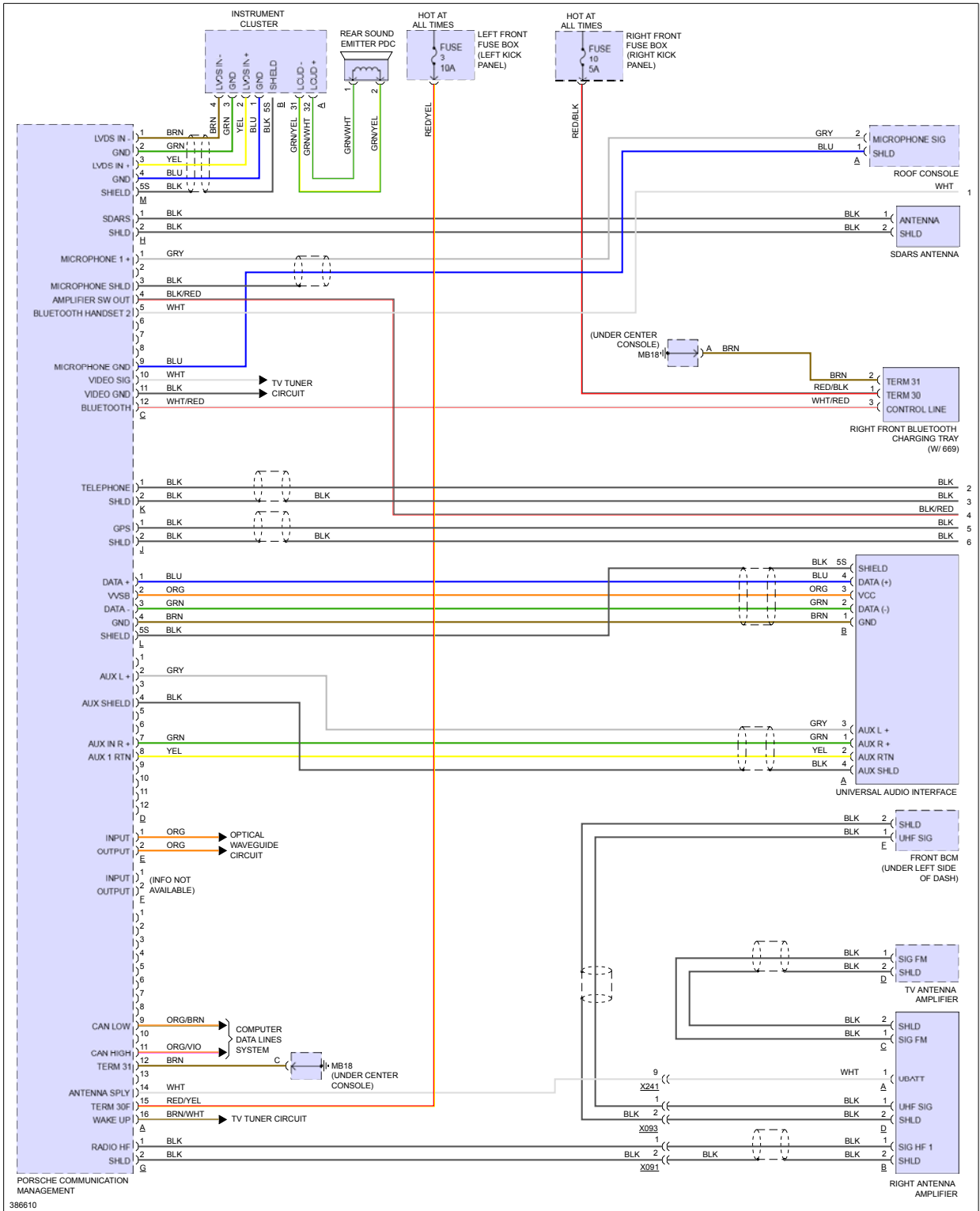
Fig 2: Navigation Circuit, W/ ASK (1 of 2)
