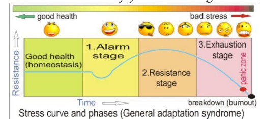
Stress curve and phases (General adaptation syndrome)
