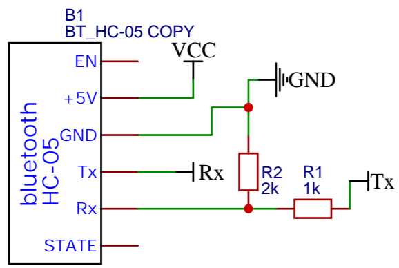
Bluetooth(slave & master)
