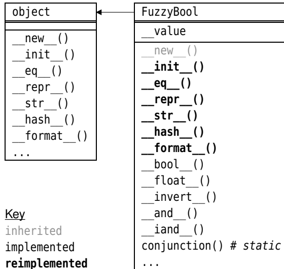
Figure 6.4 The FuzzyBool class's inheritance hierarchy
