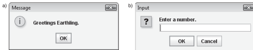
Figure 2-19 Dialog boxes
