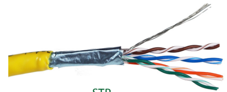
STP Shielded Twisted Pair
