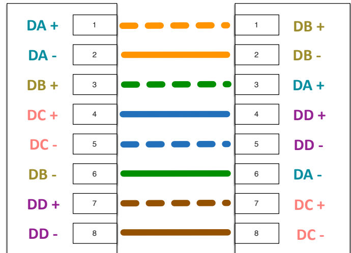
Media Dependent Interface (MDI) Network Interface Card
