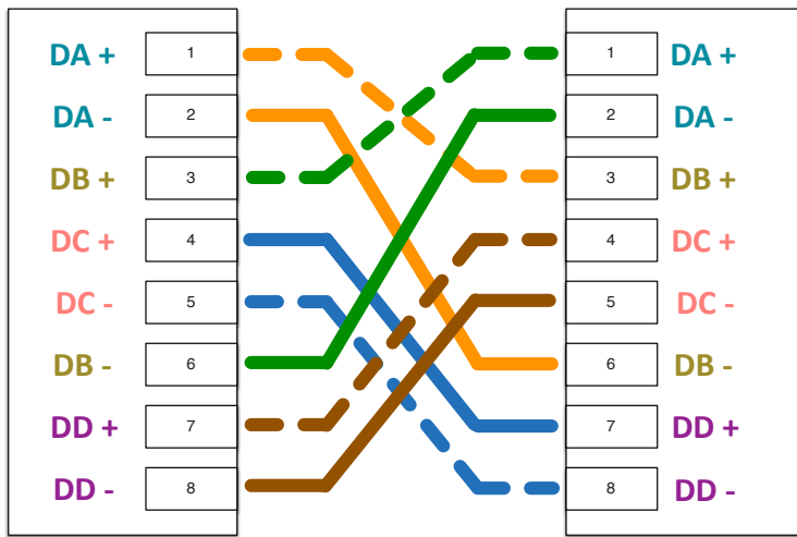
Media Dependent Interface (MDI) Network Interface Card
